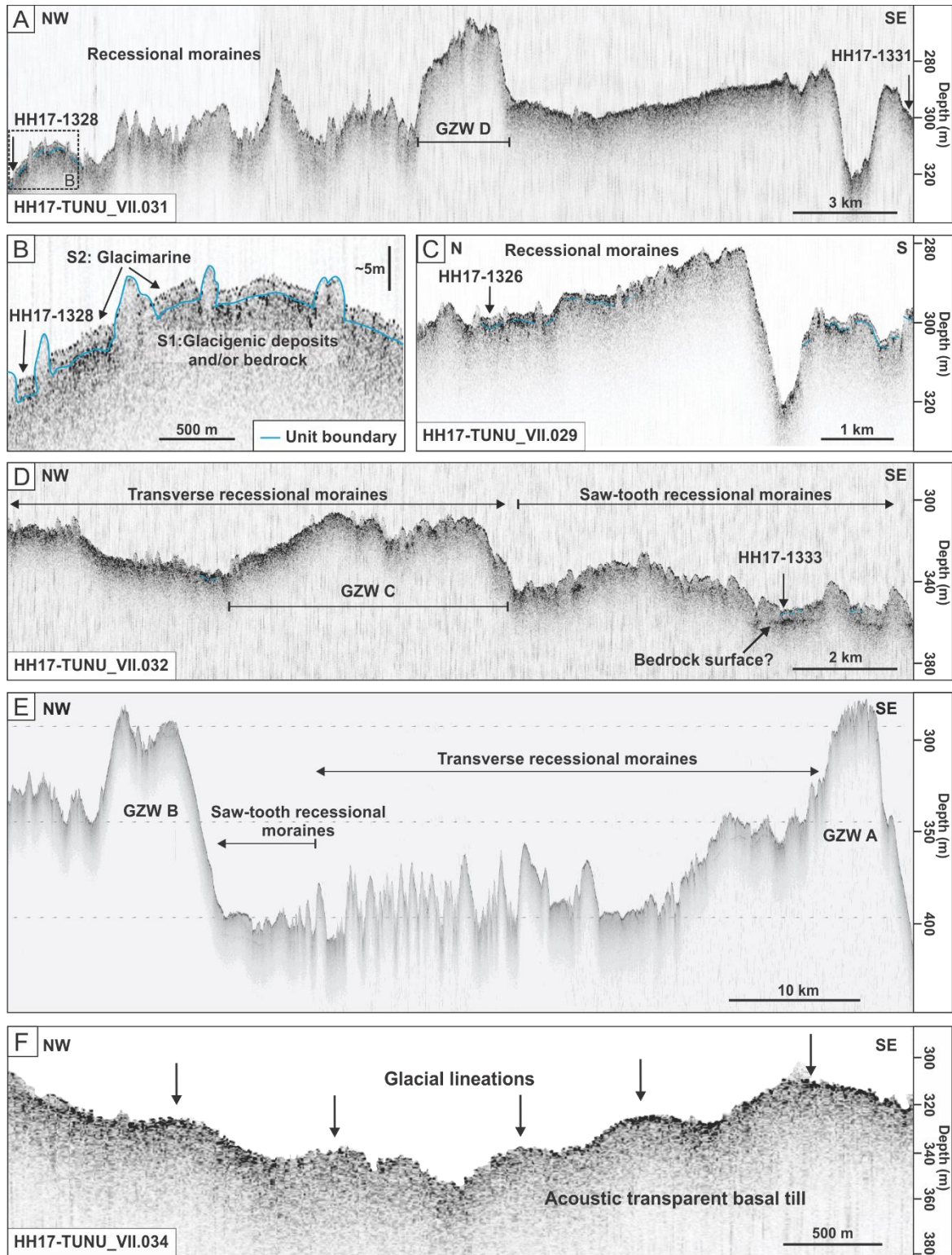
Figure 7. High-resolution seismic profiles from Store Koldewey Trough. See Fig. 1C for locations. (A) Chirp line HH17-TUNU_VII.031 across grounding zone wedge D and recessional moraines from the middle trough area. Projected positions of sediment cores HH17-1328 and HH17-1331 are shown. Black dotted rectangle shows extent of the profile in (B). (B) Part of chirp line HH17-TUNU_VII.031 showing a zoom-in example of the configuration of units S1 and S2. (C) Chirp line HH17-TUNU_VII.029 from the inner part of the trough, with recessional moraines. Projected position of sediment core HH17-1326 is indicated. (D) Chirp line HH17-TUNU_VII.032 across grounding zone wedge C. The locations for transverse recessional moraines, saw-tooth recessional moraines and sediment core HH17-1333 are indicated. (E) Chirp line across grounding zone wedge A and B, separated by saw-tooth- and transverse recessional moraines. Modified from Laberg et al. (2017). (F) Part of chirp sub-bottom profile HH17-TUNU_VII.034 showing the acoustically transparent deposits interpreted as basal till/glacial lineations. The ridges of the latter are indicated with arrows.
