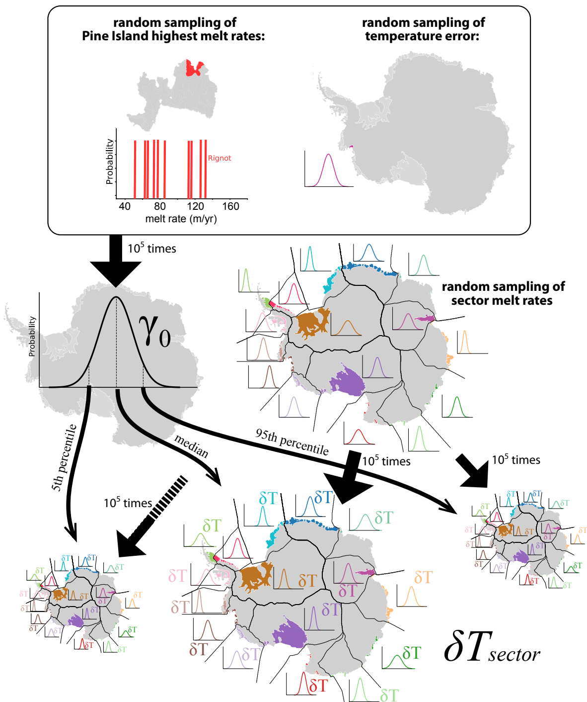
Figure 4. PIGL method used to calibrate \gamma_0 and \delta T_{sector} .
