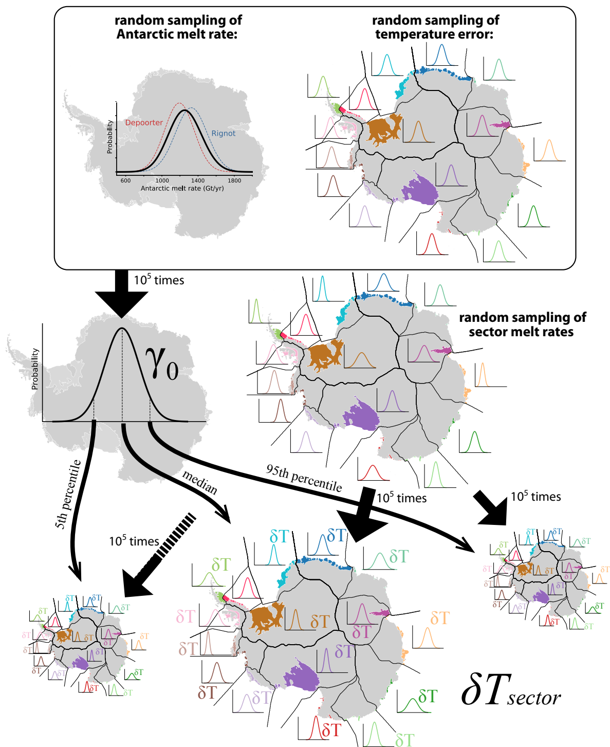
Figure 3. MeanAnt method used to calibrate \gamma_0 and \delta T_{sector} .
