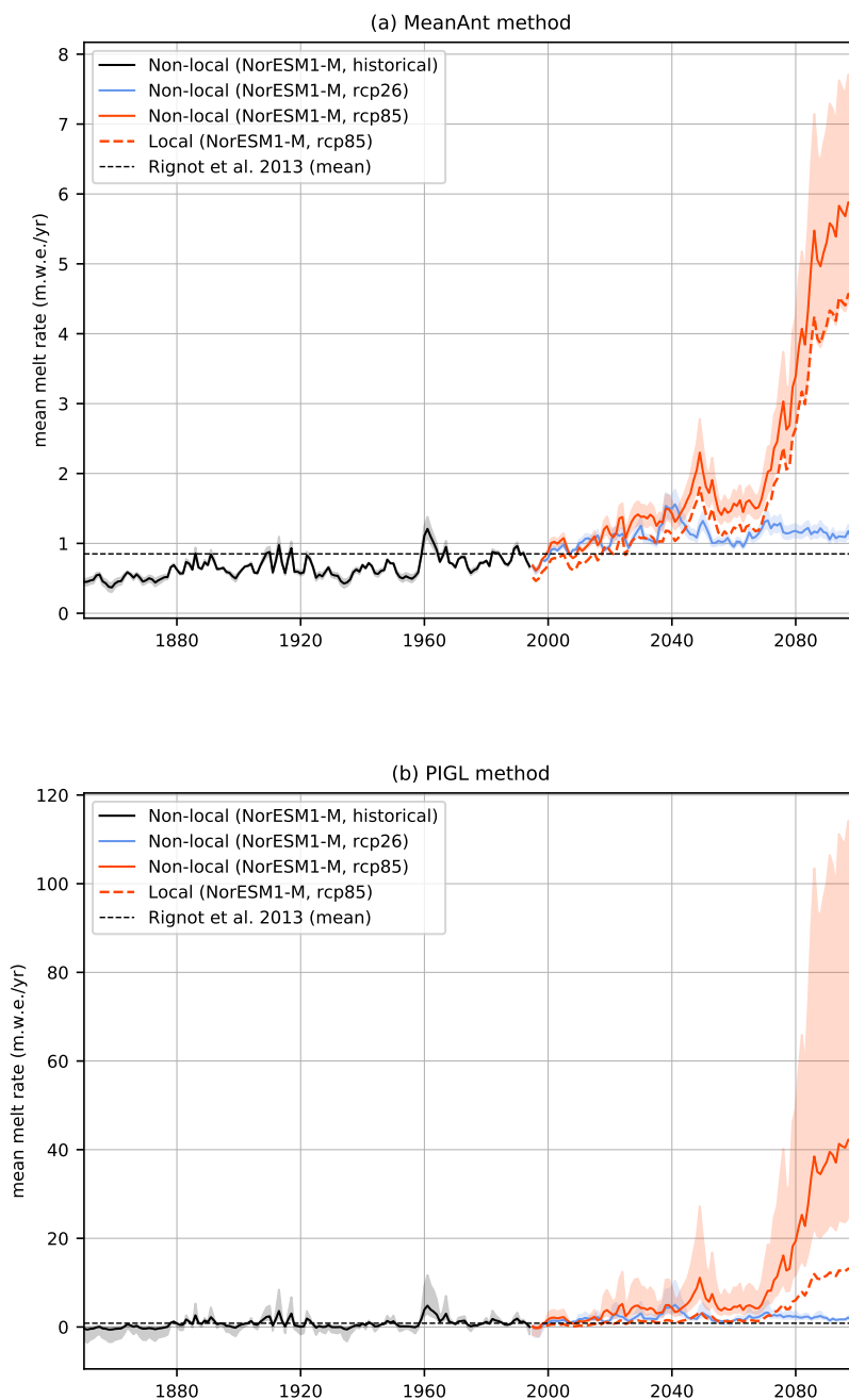
Figure 9. Time series of mean Antarctic ice-shelf basal melt rates (using the non-local parameterization and assuming a static ice-sheet geometry), based on the non-local parameterization, calibrated following (a) MeanAnt method and (b) PIGL method, and obtained from the NorESM1-M CMIP5 simulations. The semi-transparent area indicates the 5-95th percentile range related to the uncertainty in \gamma_0 . Note the different amplitudes for the melt rates.
