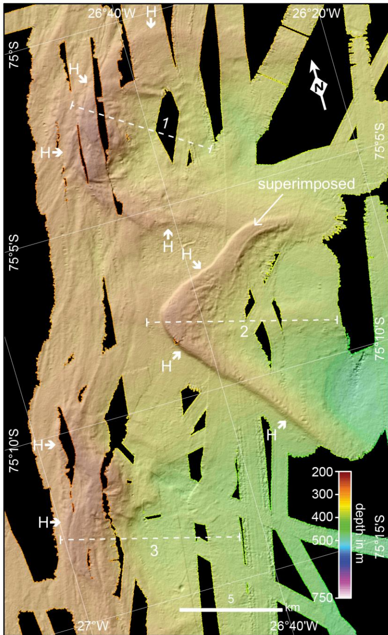
Figure 3: High-resolution bathymetric map of the McDonald Bank showing crescent-shaped ramps of Class H (fronts marked by bold short arrows), note that the northern part of ramp 2 superimposes on the southern part of ramp 1 and the locally irregular seafloor morphology on the top of ramp 2. Dashed numbered lines indicate locations of ramp profiles shown in Fig. 5.
