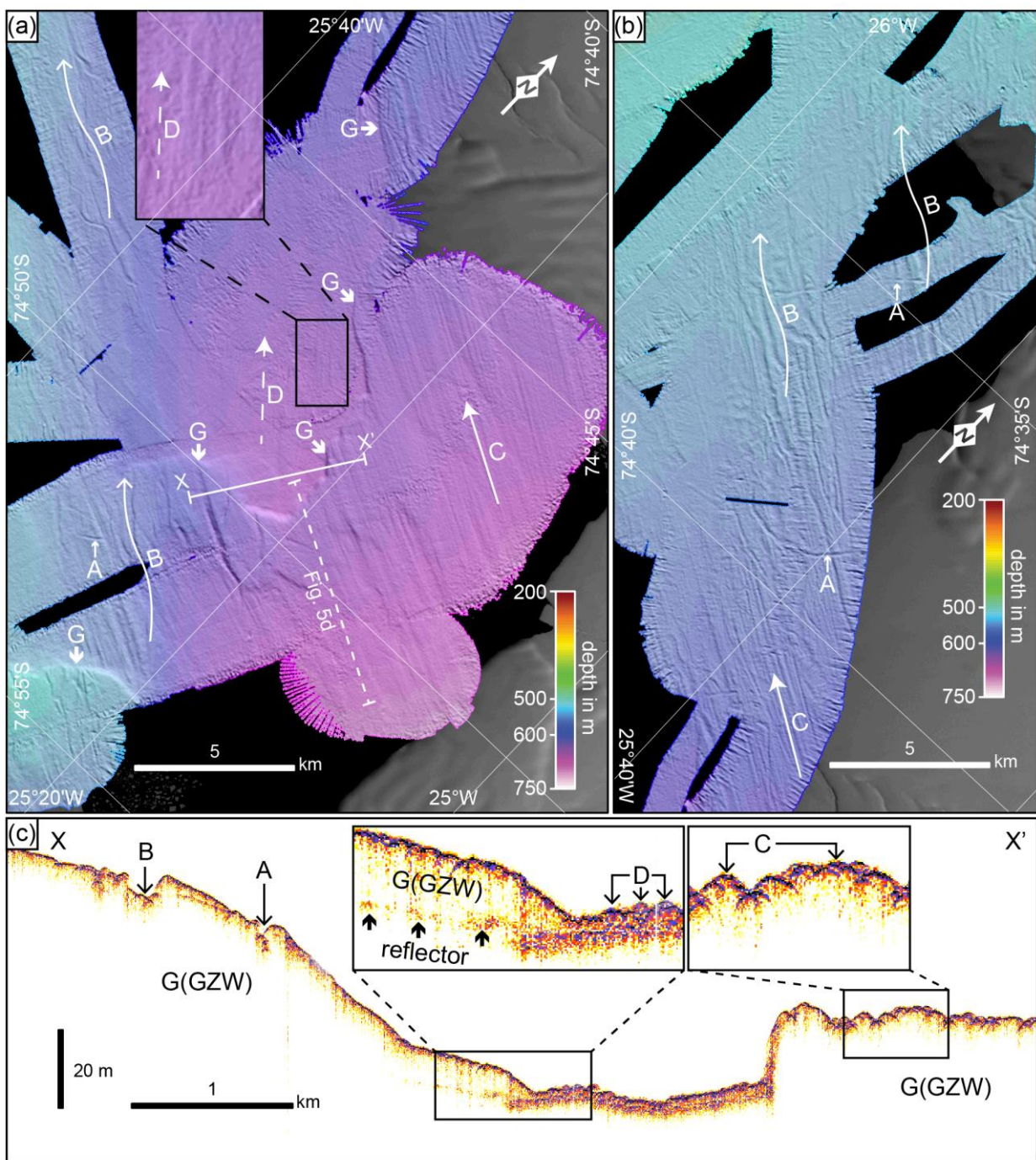
Figure 6: High-resolution bathymetric map from (a) inner and (b) middle Stancomb-Wills Trough showing ploughmarks eroded by individual icebergs (Class A) and by icebergs pushed by an ice shelf in a preferred orientation (Class B), glacial lineations (long arrows = Class C, long dashed arrows = Class D), and two grounding-zone wedge (GZW) fronts (bold short arrows, Class G). The acoustic subbottom profile (c), whose location is shown in (a), crosses bedforms landforms of Classes A, B, C, D and G.
