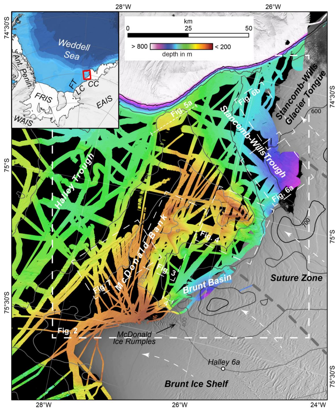
Figure 1: Overview map of the study area showing color-coded high-resolution bathymetric data and geographic locations mentioned in the text. Greyscale contour lines are in 100 m interval from the IBCSO V1.0 data set (Arndt et al., 2013). Background satellite image is from Landsat, courtesy of the U.S. Geological Survey. Locations of other figures and two bathymetric cross profiles, shown in Fig. 5, are indicated by dashed rectangles and lines, respectively. The inset map shows the study area in a broader Antarctic context (background from Arndt et al., 2013). CC = Caird Coast; EAIS = East Antarctic Ice Sheet; FRIS = Filchner Ronne Ice Shelf; FT = Filchner Trough; LC = Luitpold Coast; WAIS = West Antarctic Ice Sheet.
