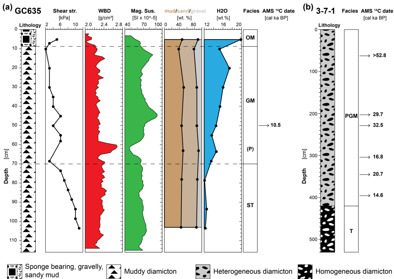
Figure 8: Sedimentological parameters and radiocarbon ages from cores in the study area (for location, see Fig. 2): a) Lithology, shear strength (str.), wet bulk density (WBD), magnetic susceptibility (mag. sus.), grain-size composition of sediment matrix, water content (H 2 O), facies interpretation and AMS 14 C ages of core GC635 (this study); b) Lithology and AMS 14 C ages of core 3-7-1 (modified from Stollendorf et al., 2012). For ages, see Table S2.
