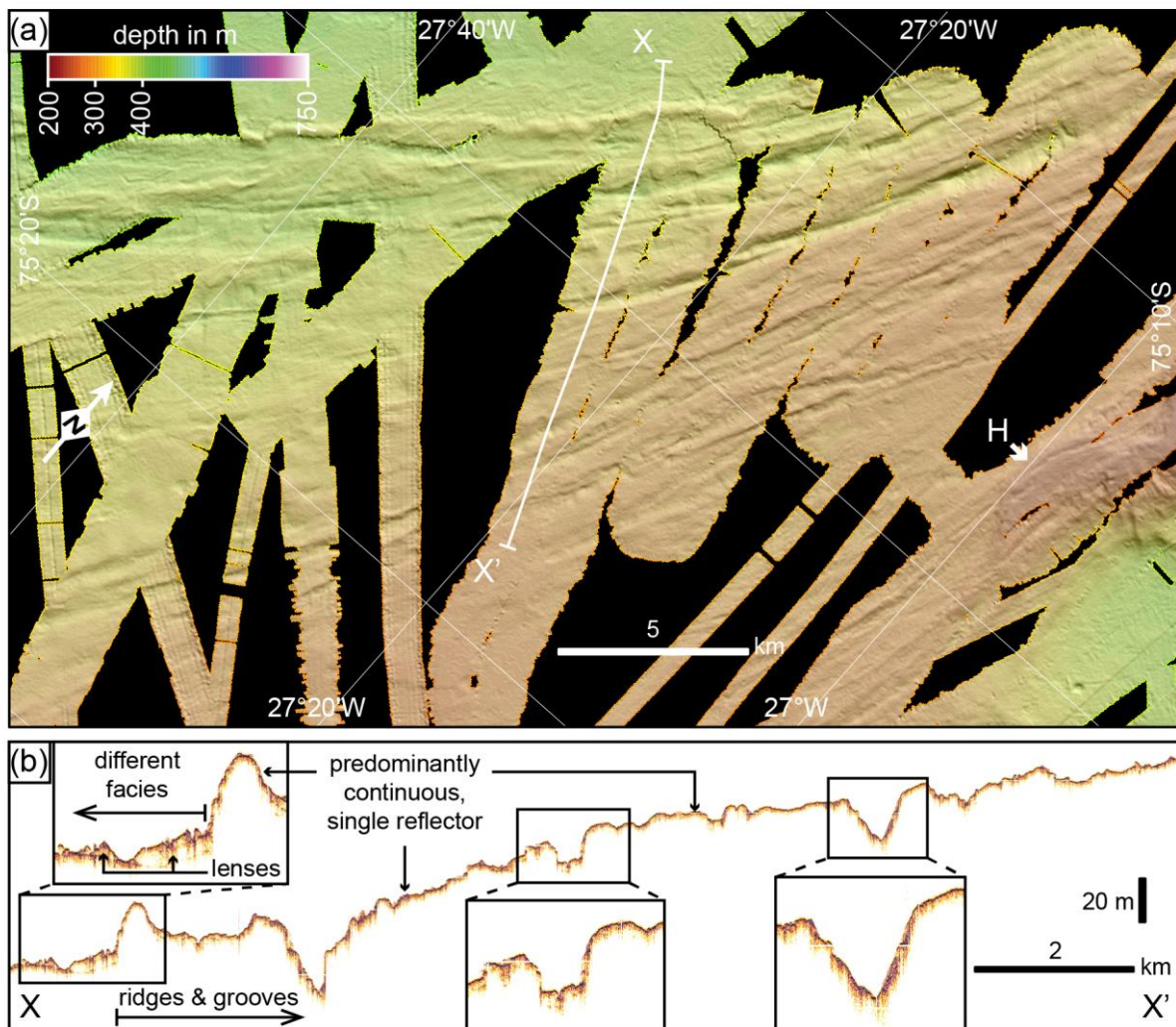
Figure 7: High-resolution bathymetric map (a) from the western slope of McDonald Bank showing curvilinear ridges and grooves of Class I that are interpreted as ice marginal bedforms and landforms . Bold short arrow marks the front of the westernmost Class H ramp. Subbottom profile (b) displays the depths of the groove incisions, the lack of penetration of the acoustic signal, and a different acoustic facies northwest of the ridges and grooves.
