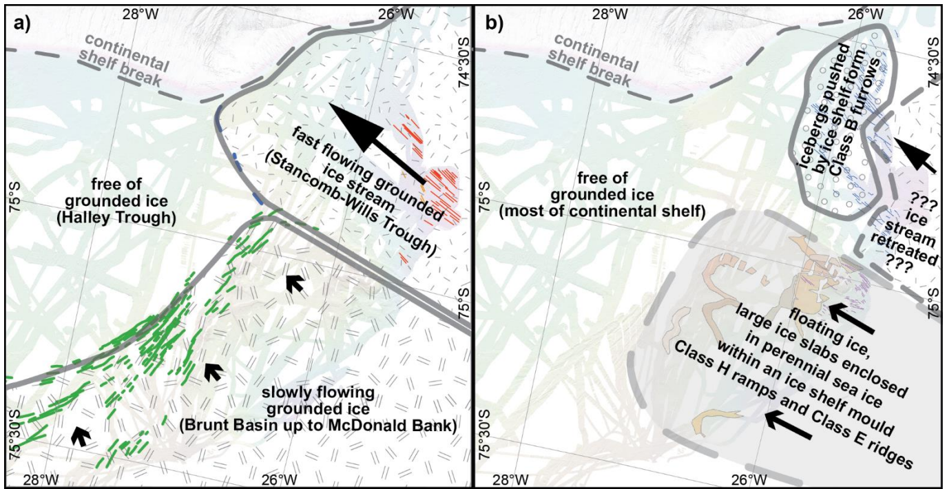
Figure 11: Schematic cartoon illustrating the two reconstructed glaciological regimes in Brunt Basin and on McDonald Bank: a) The first regime with slow flowing grounded ice forming Class I ridges at its margin, b) the second regime in which large ice slabs mould Class H ramps and Class E ridges. Background and landforms relevant for the respective regimes correspond to Fig. 2.
