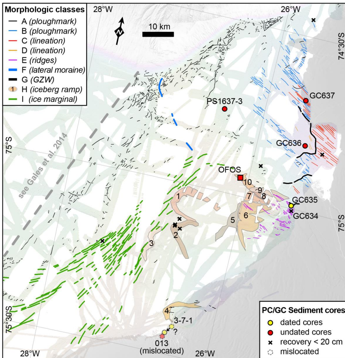
Figure 2: Mapped landform classes in the study area, for location see Fig. 1. Dots and crosses mark the locations of piston cores (PC) and gravity cores (GC) (for core site details, see Supplementary Table S1). Note that cores 13 and 3-7-1 are presumedably to have been mislocated due to inaccurate positioning capabilities in the 1970s, when these cores were retrieved. Core site 3-7-1 is relocated by shifting it to the nearest location in the high-resolution bathymetry data that has the same water depth as measured at the core location. The red square indicates the area where seafloor images were taken by the Ocean Floor Observation System (OFOS; see Fig. S1).
