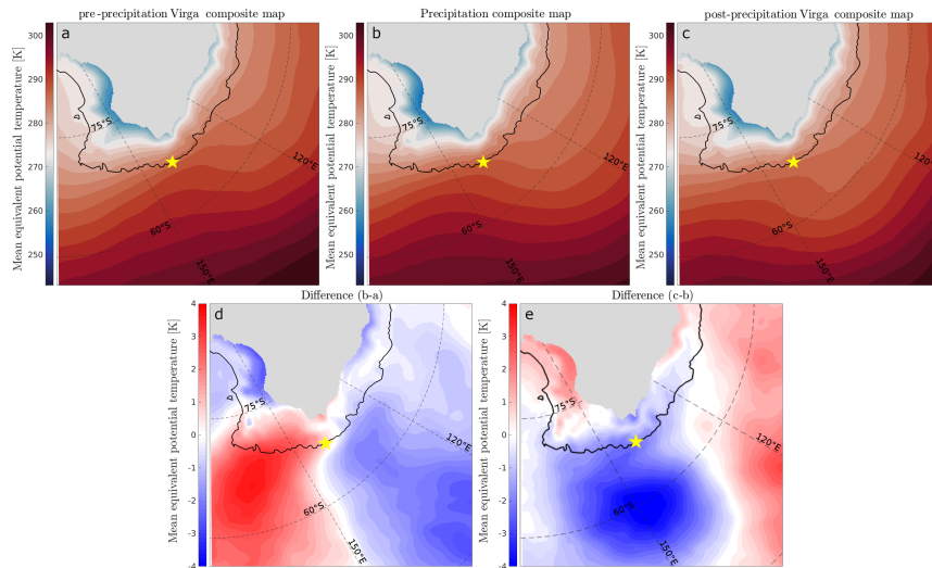
Figure 5: Composite maps of equivalent potential temperature at 700 hPa for the pre-precipitation virga composite (panel a), surface precipitation composite (panel b) and post-precipitation virga composite (panel c). Panel d shows the difference between panel b and panel a, panel e the difference between panel c and panel b. Regions with a topography higher than 2500 m ( \approx altitude of the 700 hPa level) has been shaded.
