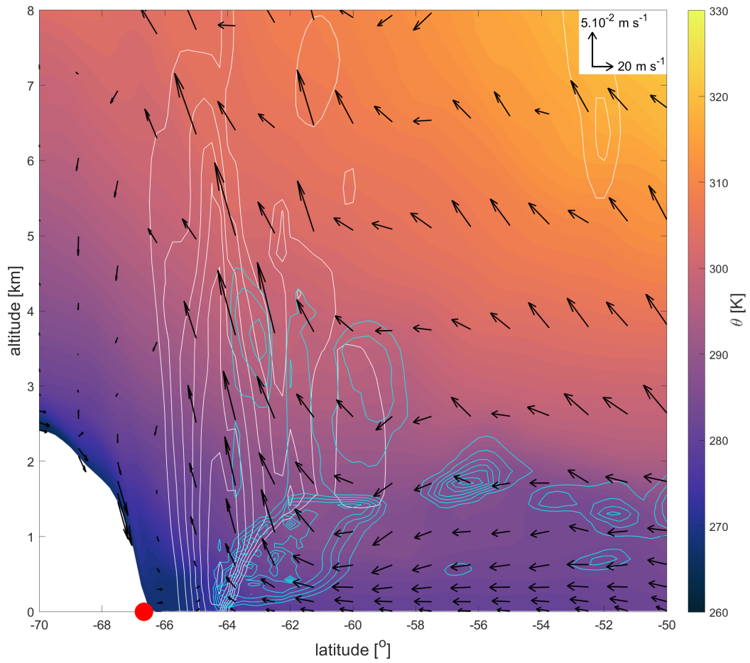
Figure 2: 140.00°E meridional cross-section of the potential temperature (shading), meridional and vertical wind (black arrows), snow+ice water contents (white contours), cloud liquid water content (cyan contours) from ERA5 data on Feb 08 2017 00:00:00 UTC. Contour interval is 5 \cdot 10^{-5} \text{ kg kg}^{-1} . Horizontal and vertical components of the wind vectors are scaled with the same ratio as the horizontal and vertical extents of the transect. DDU location is indicated by the red circle (140.00°E, 66.66°S).
