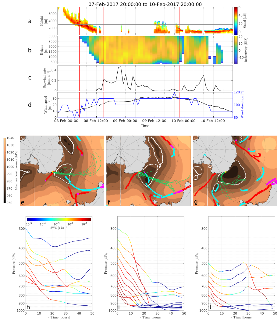
Figure 3: Case study of a precipitation event at DDU. Panel a shows a time-height plot of the lidar signal. The 3000 m MRR maximum height is marked with a grey line. Mind the lidar signal attenuation during precipitation periods. Panel b is a time-height plot of the MRR reflectivity. Panel c is the time series of the snowfall rate derived from MRR measurements. Panel d shows the time series of the 10-m wind speed and direction. Panels e, f and g show, for three different times indicated with red vertical lines in panels a-d, the sea level pressure (shading), the cyclone mask (white contours), the front lines (red for warm front, cyan for cold front, magenta for undefined) as well as the 2-day back-trajectories of the precipitating air parcels (in green). The yellow star locates DDU. Panels h, i and j show the corresponding time evolution of the pressure along the back-trajectories. Colors indicate the snow water content.
