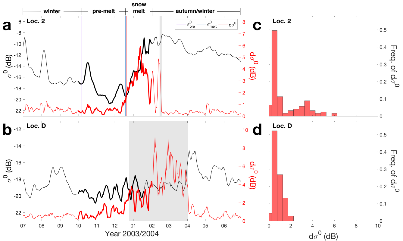
Figure 4. Typical annual time series of mean daily QSCAT radar backscatter ( \sigma^0 , black) and its diurnal variations ( d\sigma^0 , red) 15 for location 2 on perennial (a) and location D on seasonal sea ice (b) in 2003/2004. Colored vertical lines illustrate snow pre-melt ( \sigma^0_{\text{pre}} , magenta), and melt ( \sigma^0_{\text{melt}} , blue) onset derived from backscatter time series only, and snowmelt onset derived from
