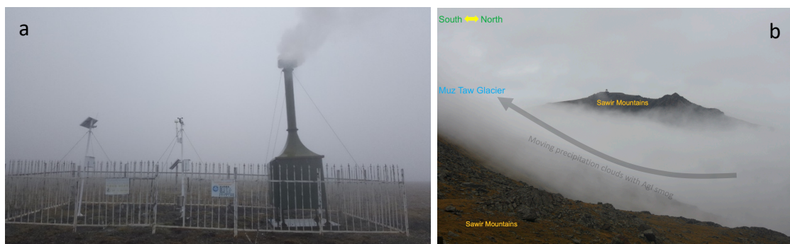
Figure 3 a) Igniting the AgI smog generators along the terminal river when the cloud accumulated late on the afternoon of 19 and 22 Aug 2018, and b) the accumulating of clouds in the valley of the Muz Taw Glacier favoured by the AgI particles moved up towards the summit of the glacier.
