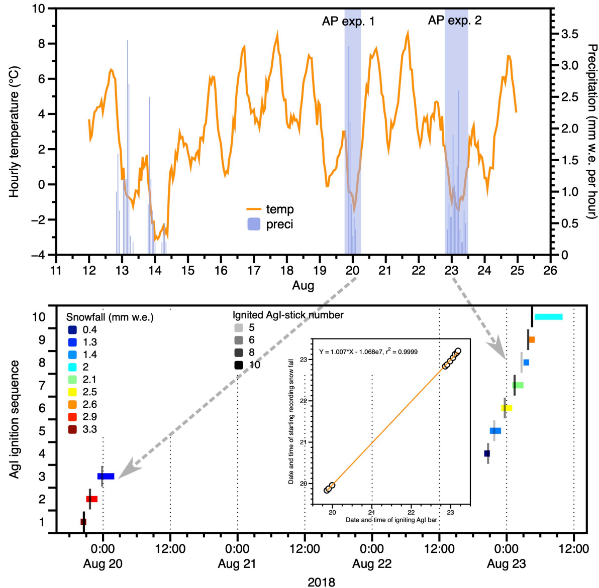
Figure 5 a) The daily snowfalls and hourly averaged temperature recorded by the AWS at ELA from 12 to 24 Aug 2018, where the two artificial-precipitation experiments (AP exp. 1 and 2) are marked, and b) the hourly snowfall amounts (indicated by color) and time periods (indicated by length) recorded by the AWS at ELA and the ignited Agl-stick number (indicated by color) and time during the two experiments.
