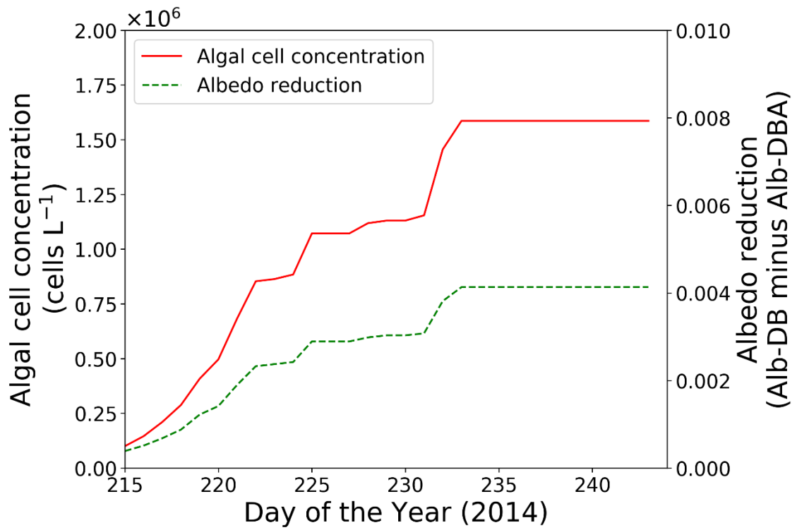
745 Figure 5: Temporal changes in algal cell concentration and albedo reduction from day 215 to 243 at the study site; algal cell concentration (red solid line) and albedo reduction (green dotted line).
