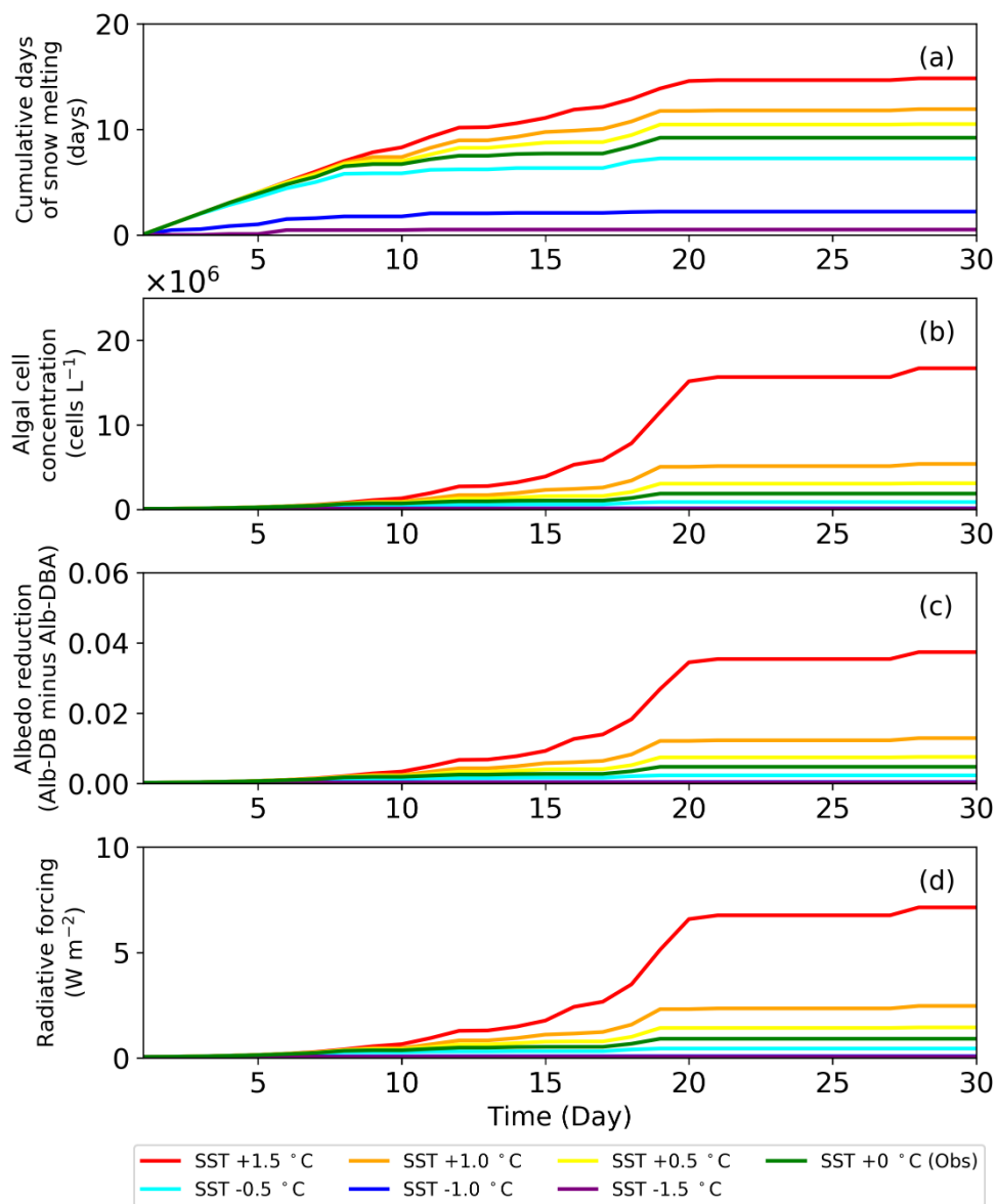
Figure 7: Temporal changes in (a) cumulative days of snow melting (b) algal growth, (c) albedo reduction by snow algae, and (d) radiative forcing by snow algae for 30 days under various surface snow temperature (SST) conditions at the study site.
