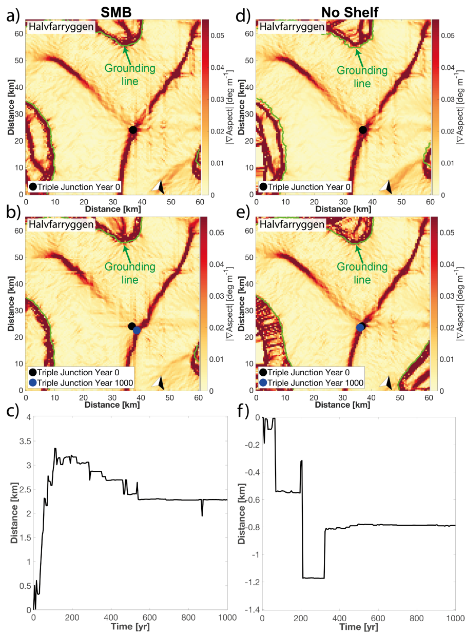
Figure 12. Triple junction migration for Halvfarryggen ice rise induced by surface mass balance perturbation for the refined mesh (a-c) and ocean perturbation (shelf removal) for the refined mesh (d-f). Upper and middle panels (a,b,d,e) show triple junction position at the start and end of the simulation period, respectively. Lower panel (c,f) shows mean divide migration for the respective perturbation simulations. Negative numbers indicate migration to the west. Note different y-axis scales in (c) and (f).
