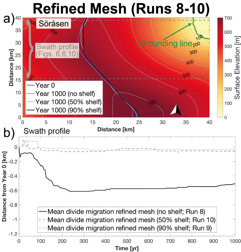
Figure 11. Ice-rise divide migration for Söråsen ice rise induced by different ocean perturbations (shelf removal, 50% ice-shelf thickness, and 90% ice-shelf thickness) for the refined mesh (a,b). (a) shows divide positions at the end of the simulation period. (b) shows mean divide migration for the different perturbations. Negative numbers indicate migration to the west.
