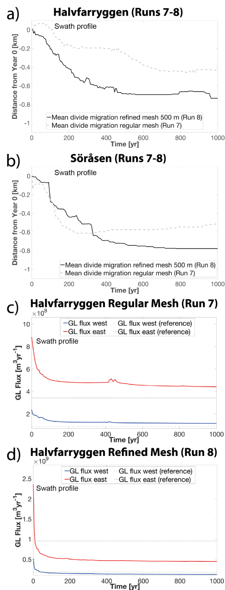
Figure 8. Ice-rise divide migration for Halvfarryggen ice rise (a) and Söråsen ice rise (b) induced by ocean perturbation (shelf removal) for different mesh resolutions. Negative numbers indicate migration to the west. (c,d) show grounding-line (GL) fluxes for the eastern and western side of the divide to the grounding line for Halvfarryggen ice rise. “Swath profile” indicates that computed divide migration is averaged over cross-sections shown in Figure 9. For the GL flux, this means that the flux is summed along the current grounding-line position over the swath length. Note different y-axis scales in (c) and (d).
