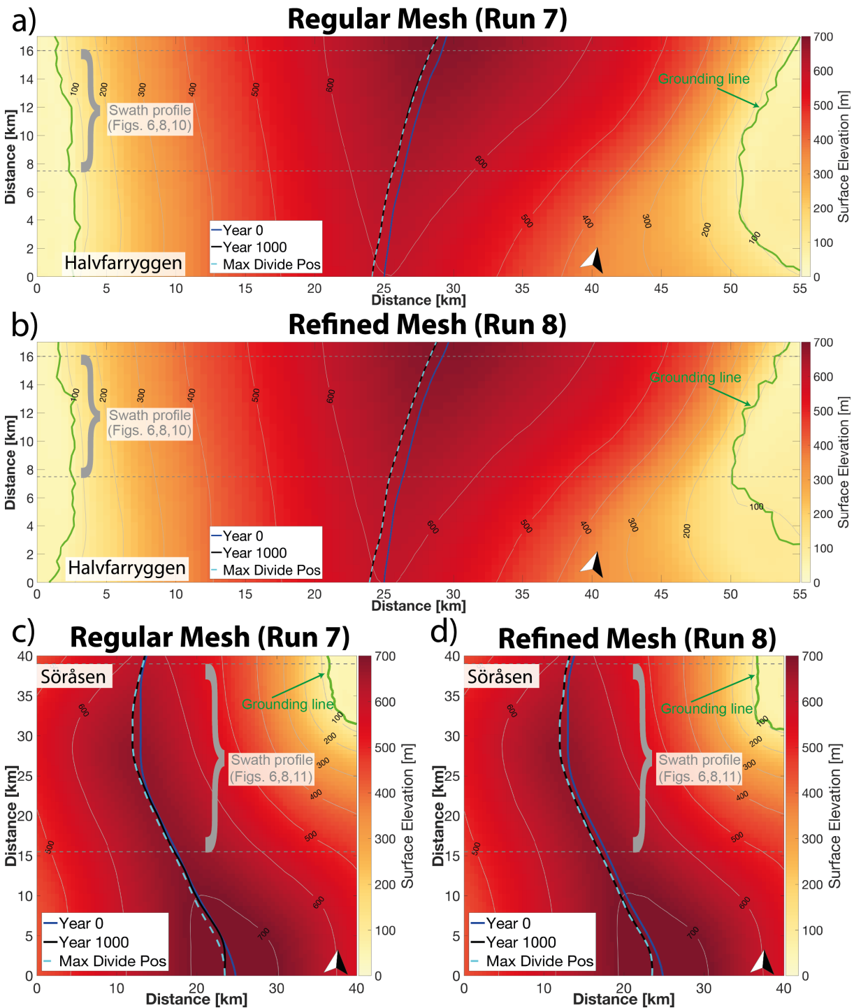
Figure 9. Ice-rise divide positions at selected times for Halvfarryggen ice rise (a,b) and Söråsen ice rise (c,d) induced by ocean perturbation (shelf removal) for the regular mesh (a,c) and the refined mesh (b,d).
