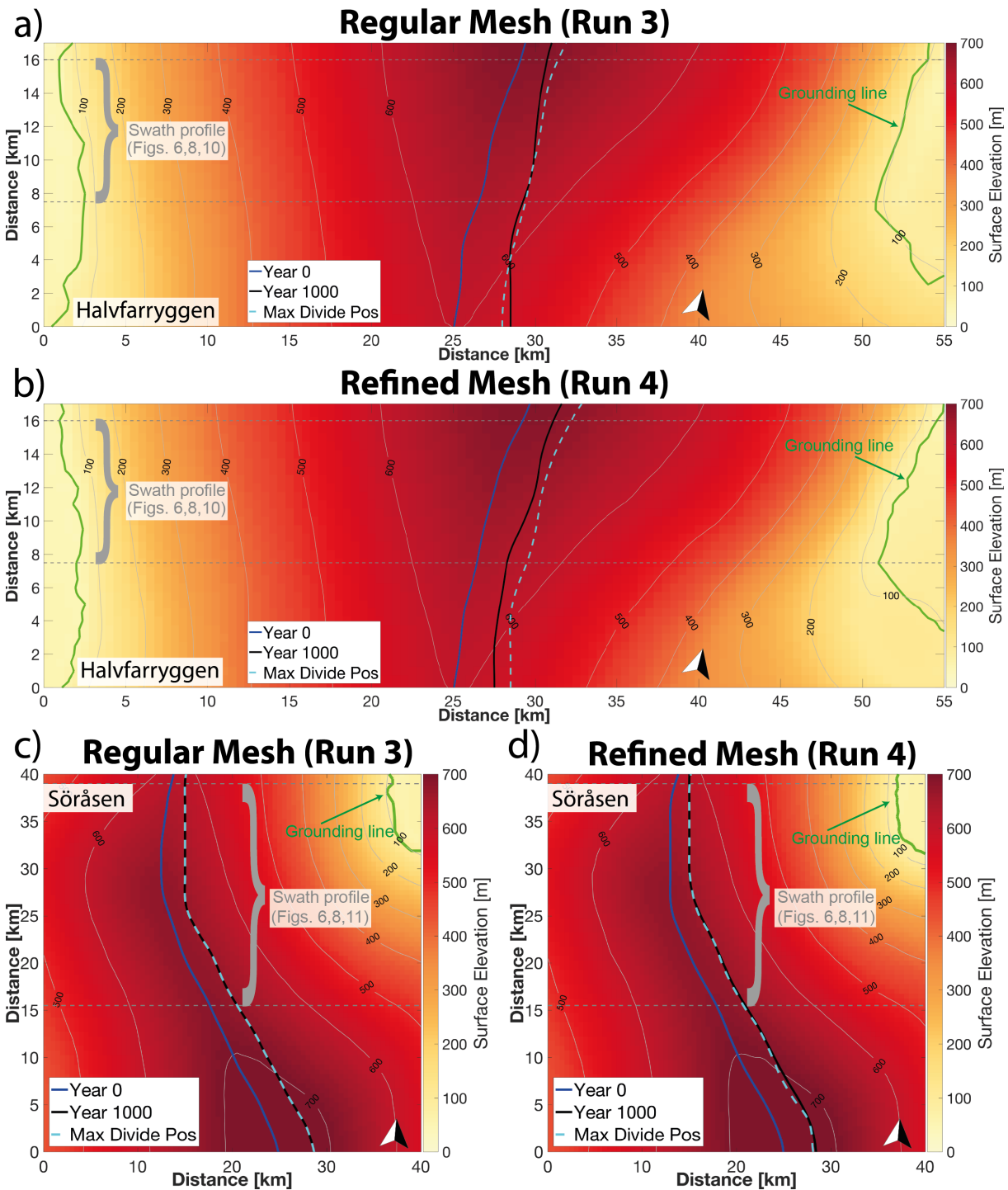
Figure 7. Ice-rise divide positions at selected times for Halvfarryggen ice rise (a,b) and Söråsen ice rise (c,d) induced by surface mass balance perturbation for the regular mesh (a,c) and the refined mesh (b,d).
