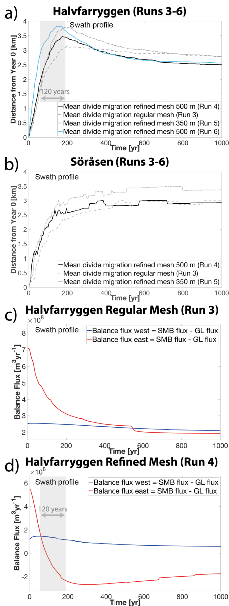
Figure 6. Ice-rise divide migration for Halvfarryggen ice rise (a) and Söråsen ice rise (b) induced by surface mass balance perturbation for different mesh resolutions. Positive numbers indicate migration to the east. (c,d) show balance fluxes for the eastern and western side of the divide to the grounding line for Halvfarryggen ice rise. Grey shaded areas in (a) and (d) highlight time lag between balance flux east being smaller than corresponding flux west and the start of backward migration. “Swath profile” indicates that computed divide migration is averaged over cross-sections shown in Figure 7. For the grounding line (GL) flux, this means that the flux is summed along the current grounding-line position over the swath length. The surface mass balance (SMB) flux is area averaged from the current divide position to the respective grounding-line position in the east and west of the divide over the swath length. Note different y-axis scales in (c) and (d).
