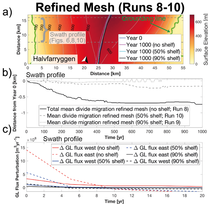
Figure 10. Ice-rise divide migration for Halvfarryggen ice rise induced by different ocean perturbations (shelf removal, 50% ice-shelf thickness, and 90% ice-shelf thickness) for the refined mesh (a-c). (a) shows divide position at the end of the simulation period. Grey dashed lines approximate area used for flux calculations in (c). (b) shows mean divide migration for the different perturbations. Negative numbers indicate migration to the west. (c) displays ice flux perturbation across the grounding line for the eastern and western side of the divide for the first two decades. Perturbation fluxes smaller than 0 indicate that ice flux across the grounding line is reduced in comparison to the reference simulation. (b,c) “Swath profile” indicates that computed divide migration is averaged over cross-sections as shown in (a). For the \Delta\text{GL} flux, this means that the flux is summed along the current grounding-line position over the swath length.
