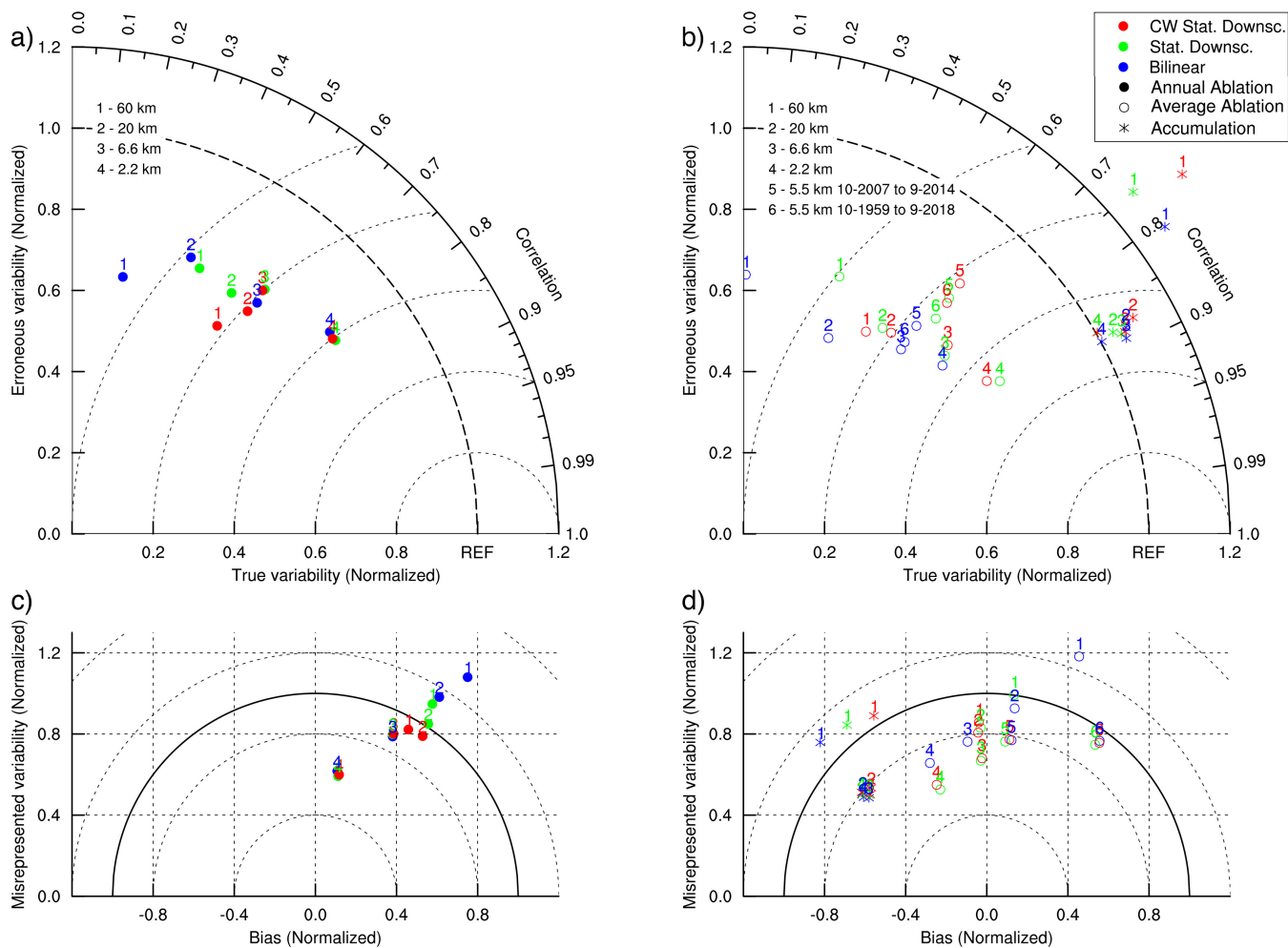
Figure 7. Graphical representation of the statistics of refined RACMO2 data for a, c ) exact time-matching ablation observations, b, d ) all ablation (circles) and accumulation (stars) observations, respectively. Subfigures a, b ) are Taylor diagrams; subfigures c, d ) show the contribution of the bias (horizontal axis) and misrepresented variability (vertical axis) to the RMSD (circles around (0,0)). All data in this Figure are scaled with the standard deviation of the observation dataset. The 5.5 km data are taken from Noël et al. (2019). The legend in b ), upper right corner, applies to all panels.
