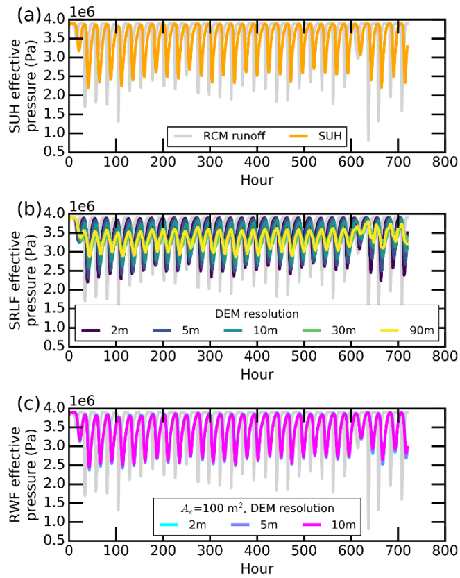
Figure 3. Subglacial effective pressures for IDC1 as simulated by SHAKTI, with inputs to the subglacial system via a single moulin prescribed by the moulin discharges (shown in Figure 2) generated by the various surface meltwater routing models. The effective pressure shown is the spatial mean over the entire 1-km square domain which contains the moulin input at its center.
