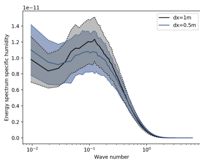
990 Figure A3: Energy spectrum for the total specific humidity at 65 meters above lowest point of the topography, averaged over the simulation hour. Shading indicates one standard deviation. The vertical axis is pre-multiplied with the wavenumber.
