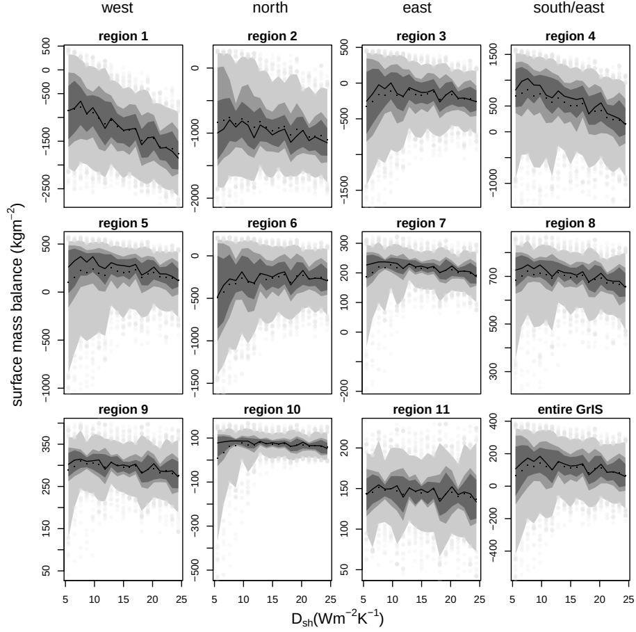
Figure 8. The dependency of the SMB on the turbulent heat exchange coefficient D_{SH} is displayed in a similar matter as Figure 8-7 for PD. The shading represents the different quantiles: 5/95(light grey), 25/75 (grey) 33/66 (dark) and the median (solid black line). The black dots are the ensemble mean based on 20 intervals. The panels are sorted by elevation and regions, with the lowest elevation (0-1000 m) in the top row, and the highest elevation at the bottom. Each column is related to a region in Greenland: W-N-E-SE/S (fig. 5).
