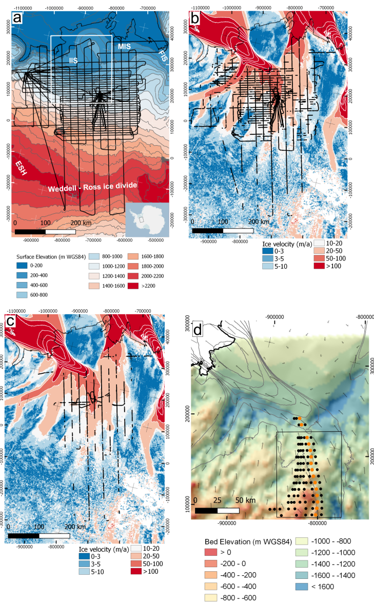
Figure 1. (a) Ice-penetrating radar survey flights over the catchments of the Institute and Möller ice streams (thick black lines), overlain on ice surface elevation (m WGS84) (Bamber et al., 2009). Thin black line in 1a-1d is MODIS grounding line (Bohlander and Scambos, 2007); Grey lines are ice surface elevation contours at 100 m intervals; White box is extent of Figure 1d; Möller Ice Stream (MIS), Institute Ice Stream (IIS), Foundation Ice Stream (FIS), Weddell-Ross ice divide and Ellsworth Subglacial Highlands (ESH) are indicated. Inset shows location of Figures 1a-c in Antarctica; (b & c) Observations of deep-ice units R1 (b) and R2 (c) in radargrams across the study area (thick black lines), overlain on MEASURES ice velocity (Rignot et al., 2017). White lines are velocity contours at 50 m/a -1 intervals. Gaps in observations are where either data were not acquired or where the deep ice unit could not be identified in the radar data (e.g. because of signal attenuation etc.); (d) Folded deep ice beneath IIS, relative to basal topography (Ross et al., 2012) and surface ice flow (Rignot et al. 2017). The location of fold axes peaks, identified in radargrams, are represented by circles. The orange dot denotes the position of the fold with the 'hand-shaped-reflection' (Figure 3d) at its core. Black box defines limits of Figure 3e. Thin grey lines are 50 m contours of MEASURES ice velocity (Rignot et al., 2017). Arrows show direction and magnitude of ice flow.
