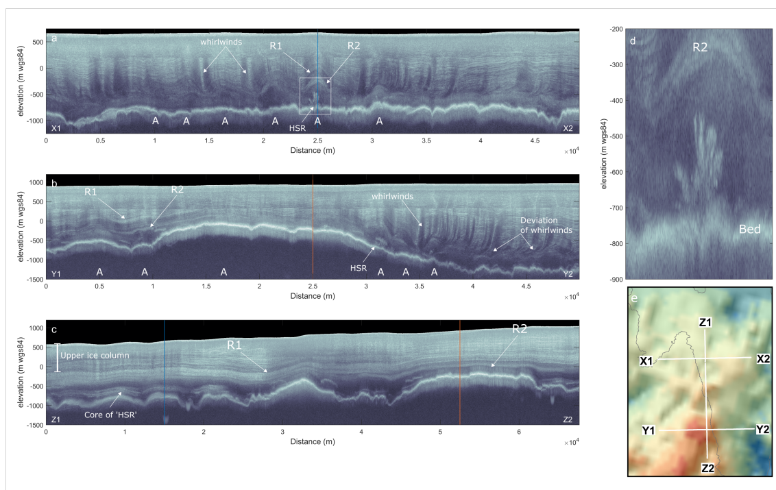
Figure 3. Ice-penetrating radargrams showing detailed englacial layering and folding: (a) down-ice, across-flow radargram (X1-X2), with englacial folds and hand-shaped reflection ('HSR'). Intersection with along-flow radargram Z1-Z2 indicated by blue vertical line. Position of fold anticlines indicated ('A'). White box is location of Fig. 3d.; (b) up-ice, across-flow radargram (Y1-Y2), showing early development of englacial folds and their positions ('A'). Intersection with along-flow radargram Z1-Z2 indicated by red vertical line. (c) Down ice-flow radargram (Z1-Z2) connecting 3a and 3b. Deep-ice units R1 and R2 are annotated. Intersections with radargrams X1-X2 and Y1-Y2 are indicated by blue and red vertical lines, respectively; (d) zoom-in of hand-shaped reflection from Fig 3a; (e) map of subglacial topography (Ross et al. 2012) showing positions (white lines) of radar transects X1-X2, Y1-Y2 and Z1-Z2. Thin grey line is 50 \text{ m a}^{-1} velocity contour (Rignot et al. 2018). Note that Fig. 3a has a different Y-axis scale to Figs. 3b and 3c.
