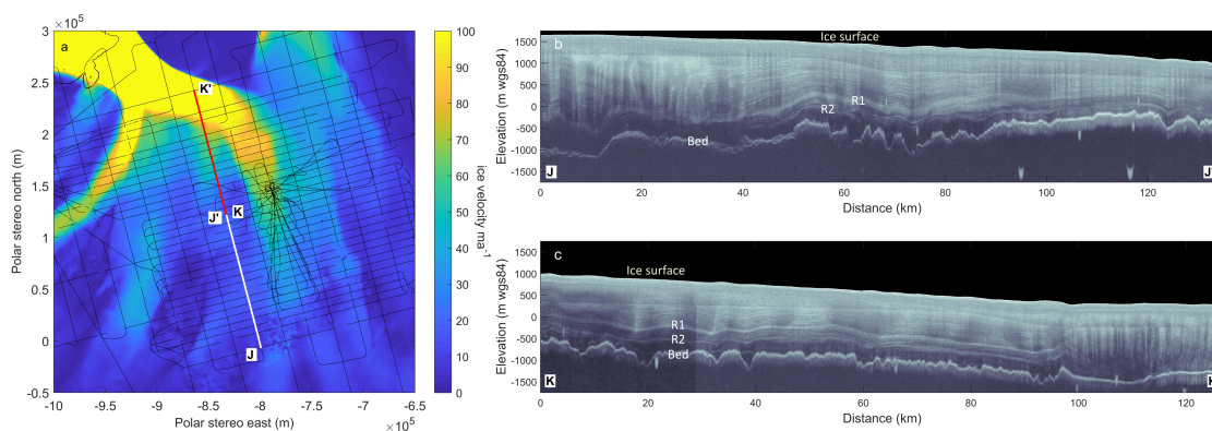
Figure 2. 260 km of radar data demonstrating the typical stratigraphy of the ice column (high reflectivity meteoric ice, underlain by low reflectivity lower ice column with high reflectivity layers, and the brightness, ubiquity and widespread nature of the deep-ice layers (R1 and R2) throughout the IIS and MIS catchments: (a) map of ice velocity (Mouginot et al., 2019) with IMAFI survey grid (thin black lines), grounding line (thin black line) and location of radar data in 2b (white line) and 2c (red line). Ice velocity colour scale is saturated at 100 \text{ m a}^{-1} ; (b) radargram of upper to mid IIS catchment (white line in 2a). Note bifurcation of R2 into 3-4 layers between 60-80 km; (c) continuation of radargram show in b into the mid- to lower- IIS catchment (red line in 2a). Isolated U-shaped ‘blobs’ are artefacts associated with SAR processing of data.
