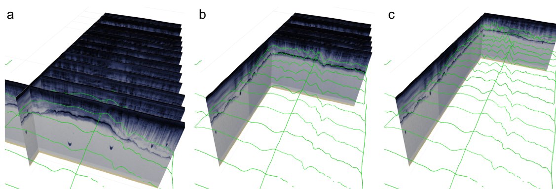
Figure 4. 3D visualisation of the picked (green lines) englacial layer R1 demonstrating 3D pattern of folding and density of survey lines: (a) radargram across ice flow lines 14-2; (b) across ice flow line 7-2; (c) across ice flow line 2. Ice flow is into page and there is 105 km between across flow lines 14 and 2. Long down-ice ‘tie’ line shown in a-c is tie line 9 (figure 2c).
