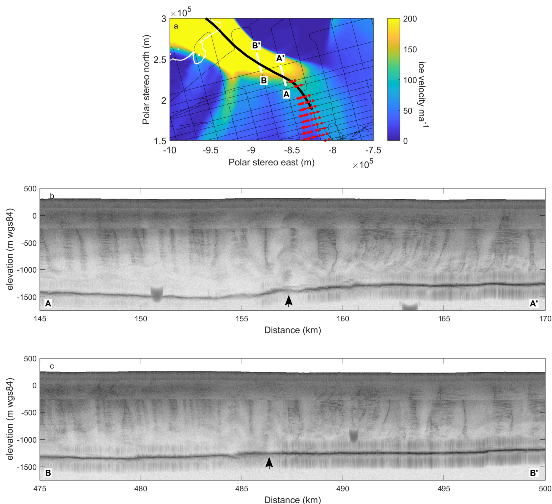
Figure 5. Englacial folds and ice flow of the IIS trunk: (a) mapped englacial fold axes (red dots) and prominent surface flow stripe (thick black line) mapped using RADARSAT and MODIS mosaics of Antarctica, overlain on ice flow (Mouginot et al., 2019), IMAFI survey grid (thin black lines), and grounding line (thin white line) (Rignot et al. 2011). Thick white lines show positions of radar data shown in 5b and 5c; (b & c) up-ice (b) and down-ice (c) radar data across the IIS trunk and perpendicular to the flow stripe and ice flow, showing the subtle, yet apparent, signature of englacial folding, including the hand-shaped reflection (HSR) fold (black arrows), within the faster flowing trunk. A qualitative increase in basal reflectivity is apparent to the right of the HSR fold in both radargrams.
