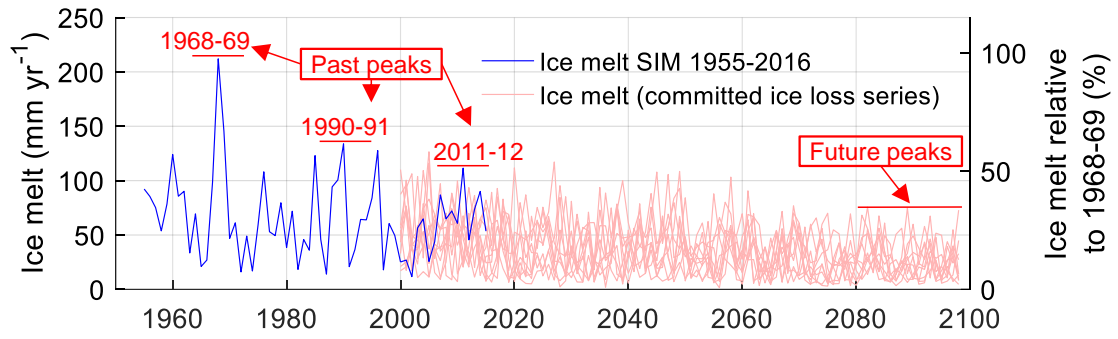
940 Figure 10: Variations in ice melt in the Maipo River Basin for the past period (1955-2016, in blue) and each one of the ten committed ice loss scenarios (light red). The peaks of ice melt over the past period and those at the final decade of the committed ice loss scenarios are highlighted in red. On the right axis, we set the ice melt estimated for the severe drought of 1968-1969 as 100%. Ice melt is computed for the Maipo River Basin (i.e. runoff units are normalized by the basin area). For visual purposes, we present the committed ice loss scenarios using the period 2000-2100 in the x-axis.
