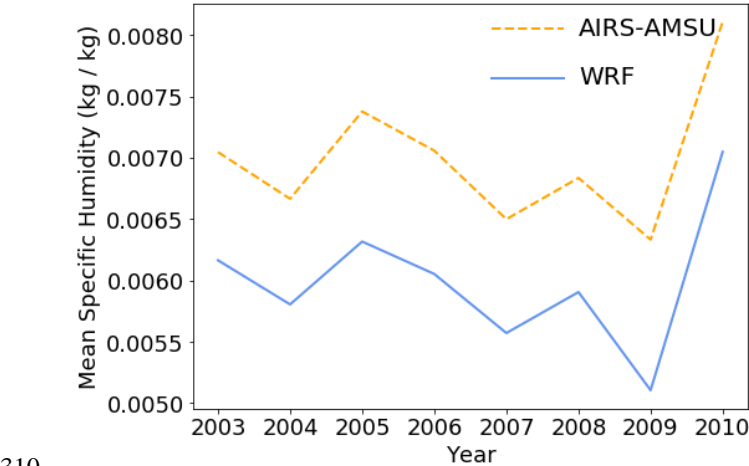
310 Figure 7: May-September mean specific humidity at 2 metres from WRF (blue, solid line) and AIRS-AMSU surface humidity (orange, dashed line) for a 1° x 1° bin around 38.5° N, 77.5° E, which is an irrigated area in the Tarim that contributes to the snowfall in WSKS.
