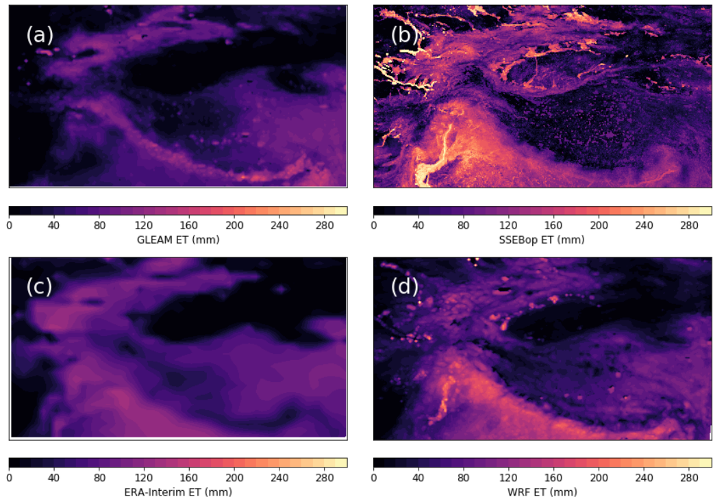
Figure 6: Evapotranspiration for July 2010 from GLEAM (a), SSEBop (b), ERA-Interim (c), and WRF (d). Mean values for the plotted domains are: 44 mm (a), 46 mm (b), 57 mm (c), and 59 mm (d).
