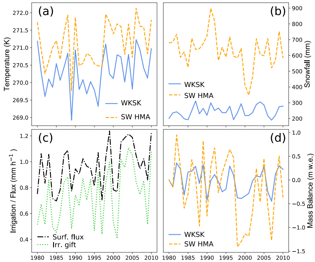
Figure 9: Time series of annual mean temperature (a), annual snowfall (b), mass balance (d) for two nearby 2 \times 3^\circ bins in WSKK and southwestern HMA that have, on average, growing glaciers ( 38\text{--}40^\circ \text{N} , 73\text{--}76^\circ \text{E} , blue lines) and shrinking glaciers ( 35\text{--}37^\circ \text{N} , 72\text{--}75^\circ \text{E} , orange, dashed lines). Panel c shows the time series of annual irrigation gift (green, dotted line) and annual surface moisture flux (black, dot-dashed line) for the most heavily irrigated point in the Tarim.
