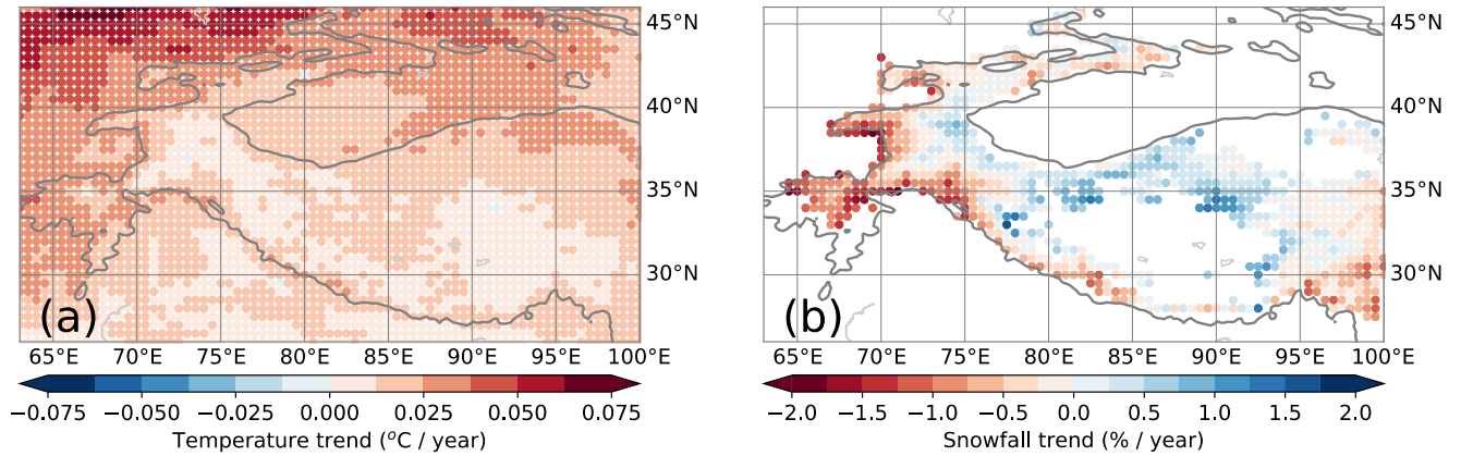
Figure 8: Trends between 1980-2010 of temperature in the melt season (a) and annual snowfall (b), averaged over 0.5x0.5° bins for clarity. Regions with monthly snowfall of less than 10 mm were masked out. The 2000 m elevation contour is indicated by a solid line.
