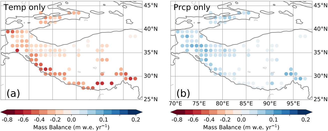
Figure 13: Simulated mean mass balance between 2000-2010 forced by a spatially uniform and constant temperature increase of +0.01 °C yr -1 , with snowfall kept constant (a), and a spatially uniform and constant snowfall increase of +0.5% yr -1 of the annual mean value, with temperature kept constant (b). Panels a and b thus show the relative sensitivity to temperature and snowfall, respectively.
