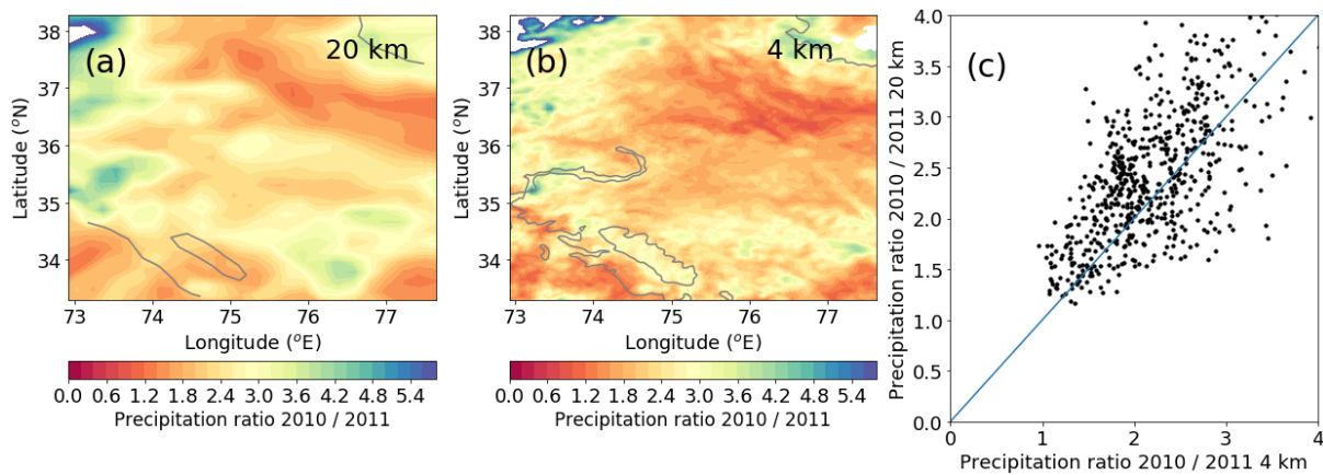
Figure 16: Precipitation ratios between May-September of two years for the WRF run at 20 km, with cumulus parameterisation (a), that at 4 km resolution, without parameterisation (b), and the two compared, when binned at the resolution of the 20 km run (c). The 2000 m elevation contour is indicated by a solid line.
