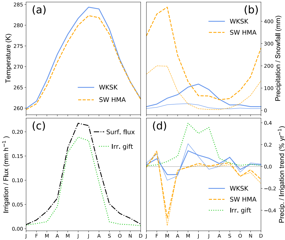
Figure 10: a) Mean seasonal cycle of temperature and b) precipitation (thick lines) and snowfall (thin lines) between 1980-2010 for the WSKS (blue lines) and southwestern HMA (orange, dashed lines), as shown in Fig. 14b,d. c) Mean seasonal cycle of the irrigation gift (green, dotted line) and surface moisture flux (black, dot-dashed line) of the most heavily irrigated point in the Tarim. d) Trends in precipitation (thick lines) and snowfall (thin lines) for the WSKS (blue lines) and southwestern HMA (orange, dashed lines), and the trend in irrigation from the most heavily irrigated point in the Tarim (green, dotted line), all as percentages of the annual mean value.
