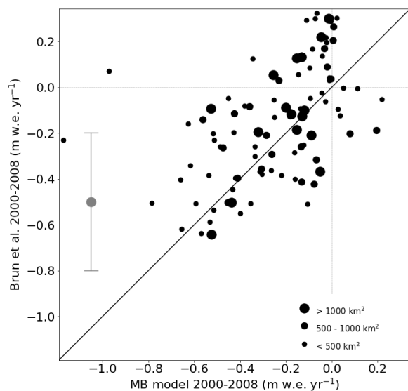
Figure 12: Comparison between mean modelled mass balances from this work, binned on a 1 \times 1^\circ grid as in Fig. 11, and those derived from observations of Brun et al. (2017), which are on the same grid, between 2000-2008. The size of the mean errors on the observed mass balances is illustrated by the grey error bar.
