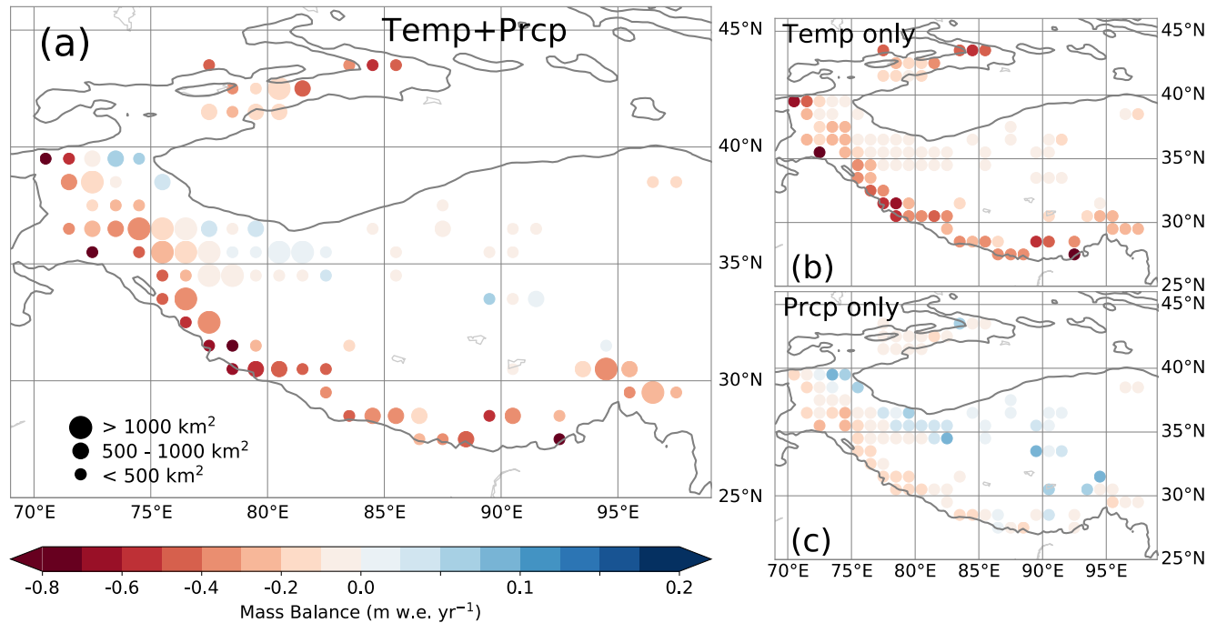
370 Figure 11: Simulated mean mass balance between 2000-2010 forced by changes in temperature and annual snowfall from WRF (a), only changes in temperature from WRF (b), and only changes in annual snowfall from WRF (c). Results are binned in 1 \times 1^\circ bins, and bins with total glacier volumes less than 5 \text{ km}^3 are not shown, to enable comparison with previous studies. The 2000 m elevation contour is indicated by a solid line.
