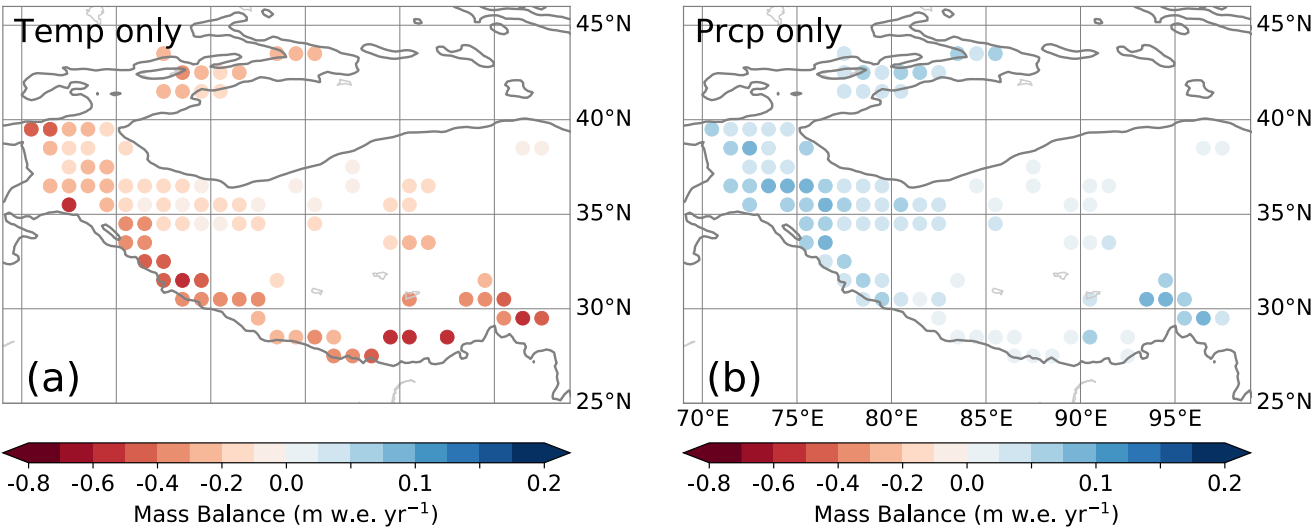
400 Figure 13: Simulated mean mass balance between 2000-2010 forced by a spatially uniform and constant temperature increase of +0.01\text{ }^{\circ}\text{C yr}^{-1} , with snowfall kept constant (a), and a spatially uniform and constant snowfall increase of +0.5\%\text{ yr}^{-1} of the annual mean value, with temperature kept constant (b). Panels a and b thus show the relative sensitivity to temperature and snowfall, respectively.
