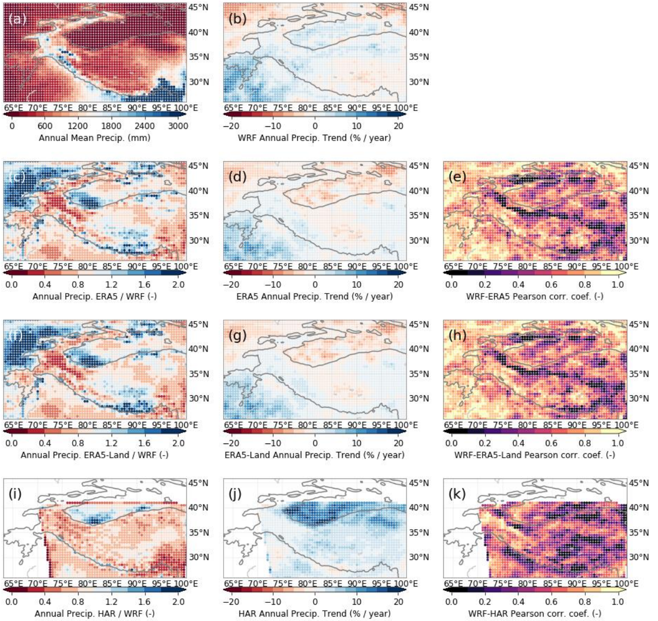
Figure 4: Comparison of WRF precipitation output [a-b] with three other datasets (ERA5 [c-e], ERA5-Land [f-h], and HAR [i-k]) between 2001-2010. Columns show precipitation multiplication factors (c,f,i) with respect to the annual mean precipitation (a), annual precipitation trends (b,d,g,j), and Pearson correlation coefficients between the datasets and our WRF results (e,h,k). The 2000 m elevation contour is indicated by a solid line.
