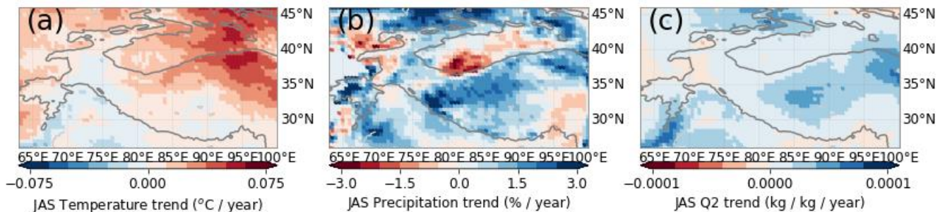
Figure 17: WRF trends between 1980-2010 of near-surface temperature (a), total precipitation (b), and specific humidity (c) between July-September, averaged over 0.5 \times 0.5^\circ bins for clarity. The 2000 m elevation contour is indicated by a solid line.
