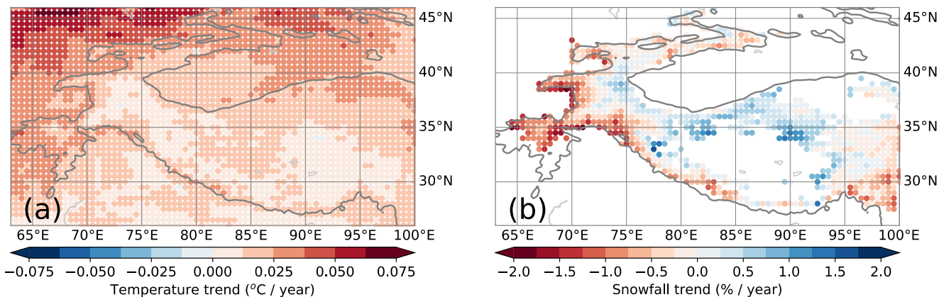
335 Figure 8: Trends between 1980-2010 of temperature in the melt season (a) and annual snowfall (b), averaged over 0.5x0.5° bins for clarity. Regions with monthly snowfall of less than 10 mm were masked out. The 2000 m elevation contour is indicated by a solid line.
