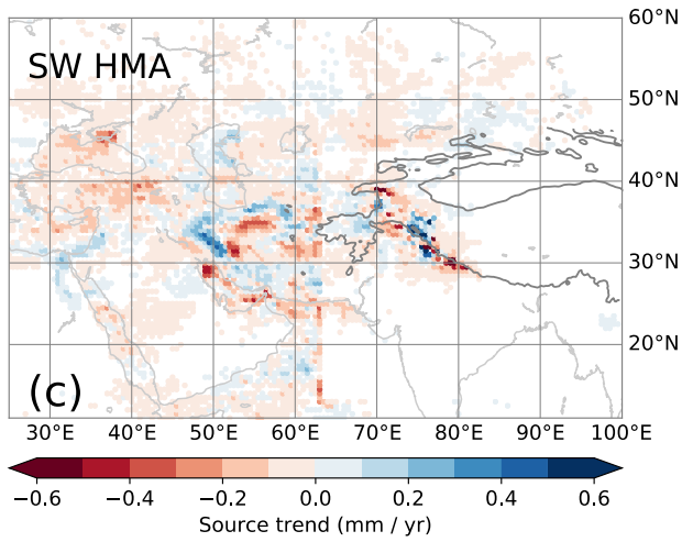
Figure 14: Trends in the amount of moisture from a given source contributing to precipitation trends in the target area (a,c), with a detailed view (b,d) around the target area from which the parcels were released (contoured in bold) for WSKS (a,b) and southwestern HMA (c,d). Trends with absolute magnitudes smaller than 0.02 \text{ mm yr}^{-1} are made white. The 2000 m elevation contour in the WRF domain is indicated by a solid line.
