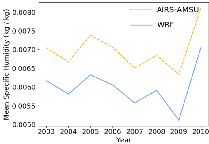
Figure 7: May-September mean specific humidity at 2 metres from WRF (blue, solid line) and AIRS-AMSU surface humidity (orange, dashed line) for a 1^\circ \times 1^\circ bin around 38.5^\circ \text{ N} , 77.5^\circ \text{ E} , which is an irrigated area in the Tarim that contributes to the snowfall in WSKS.
