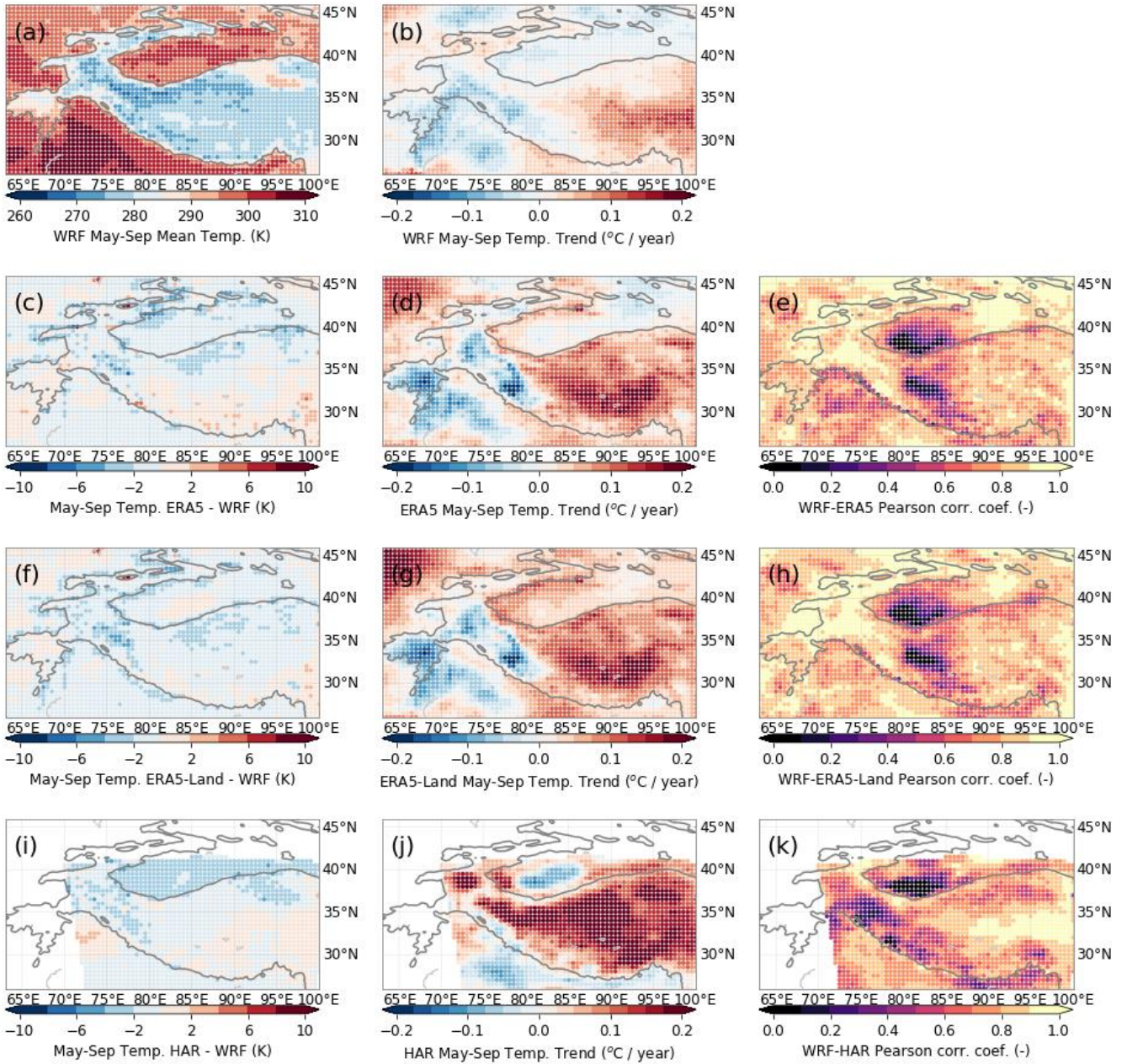
Figure 3: Comparison of WRF temperature output [a-b] with three other datasets (ERA5 [c-e], ERA5-Land [f-h], and HAR [i-k]) between 2001-2010. Columns show biases (c,f,i) with respect to the May-September mean temperature (a), May-September temperature trends (b,d,g,j), and Pearson correlation coefficients between the datasets and our WRF results (e,h,k). The 2000 m elevation contour is indicated by a solid line.
