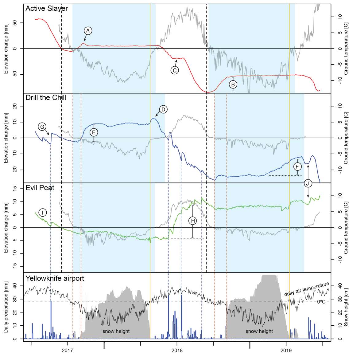
Figure 5. Daily elevation change and ground temperature (0.30–0.35 mm) recorded at the three sites, with nearby (<25 km) precipitation (blue steps) and snow height (grey polygons). Air temperature (black) is shown relative to 0°C (dashed) for context and without scale. Blue shading indicates approximate period of soil freezing, orange vertical lines indicate the approximate timing of snowpack ripening and meltwater input into the ground, vertical dashed lines indicate one full measurement year (black), selected precipitation events (blue) and the approximate duration of the autumn zero-curtain periods at Drill the Chill and Evil Peat (red). Letters in circles identify events discussed in the main text.
