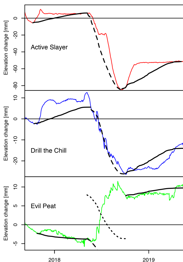
Figure 6. Visual comparison of observed elevation change (colour) with predictions (black) based on the Stefan equation and ground temperature. Solid black lines represent freezing seasons and dashed lines thawing seasons. The dotted line for site Evil Peat has been shifted upwards for clarity, illustrating that the observed thawing season was accompanied by surface heave, whereas the Stefan model predicts subsidence. Predictions are scaled and shifted to coincide with observations at the start and end of the freezing and thawing seasons and, therefore, can only be used to visually assess how well they resemble the temporal pattern of elevation, but not seasonal magnitude.
