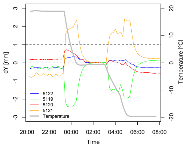
Figure 3. Tilt measured by differing sensors in the laboratory. The instruments, identified by their serial numbers, have not been moved during the experiment; instrument 5119 is not used in the field. Inclination is expressed as equivalent elevation change dY assuming an arm of length 1.5 m as is used in the field.
