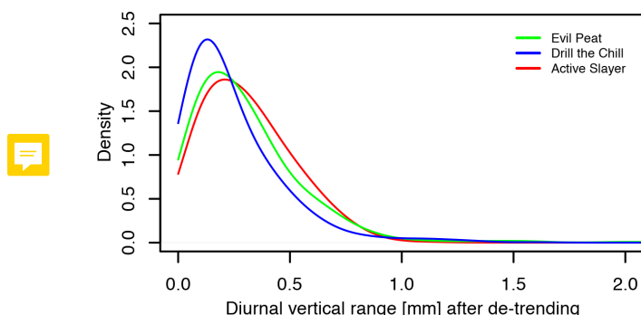
Figure 4. Density of diurnal vertical movement for all three sites.
