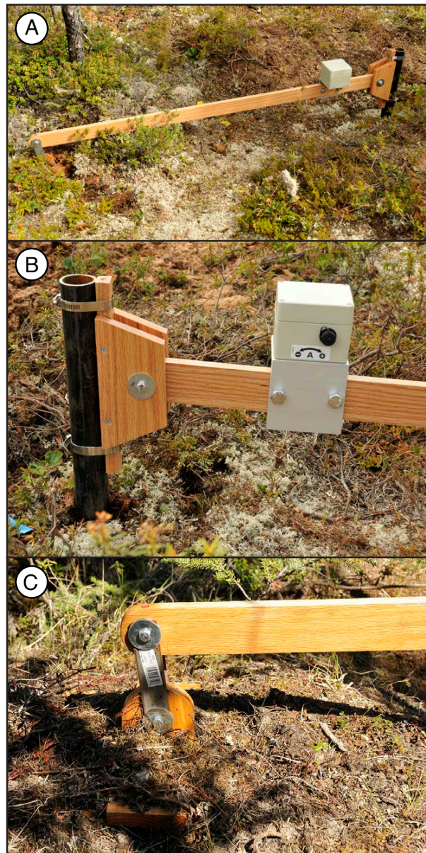
Figure 1. Tilt arm installed at site Evil Peat (A) with detailed views on the logger and the attachment to the anchor pipe (B) and the double-pivot mechanism (C) just above the wooden grille inserted beneath the vegetation.
