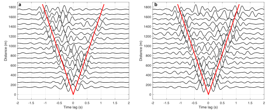
Figure R2: (a) Stacked sections of NCC in the frequency band 2.5-6 Hz averaged over two days (the 27 th and the 28 th of July 2016). The red line shows the propagation of the Rayleigh waves with velocity of 1680 m/s (also in f). (b) Stacked sections of NCC reconstructed in the frequency band from 2.5 to 6 Hz from the CSDM eigenspectrum equalization averaged over two days (the 27 th and the 28 th of July 2016).
