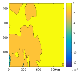
Figure 1: The cost function gradient with respect of k_2(x,y) averaged over 10 iterations. Note also, that this gradient map is in "full space" and it should be re-interpolated on sparse grid where the k_2 control is defined.
