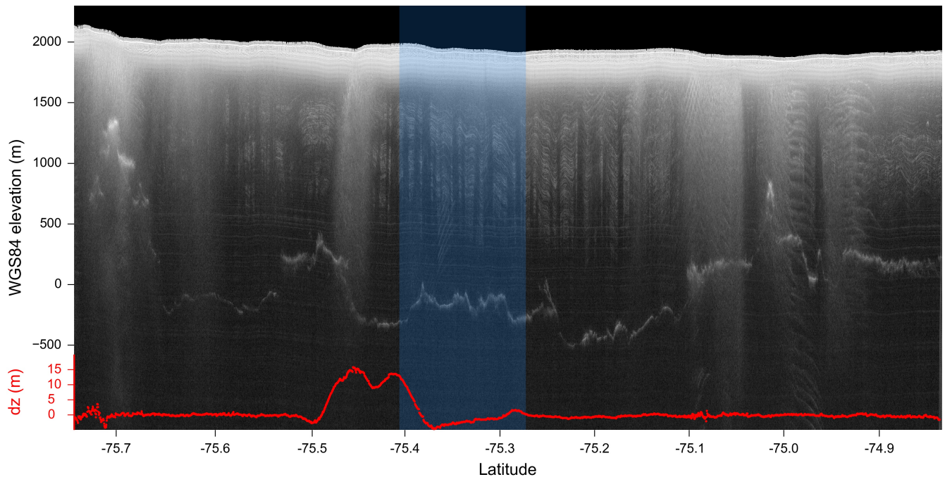
Figure 3. Focused radargram DVG/IBH0c/GL0328c. Location of the transect is shown in Fig. 7 and its overlap with the D2 lake outline is highlighted in light blue. Observed surface elevation change is shown in red. The radargram has been depth-corrected based on laser surface elevations and truncated 20 m above the surface.
