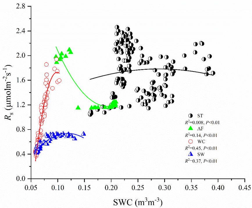
Fig. 4. Relationships between soil temperature and moisture at 5cm depth and R_s flux at summer thawing stage (ST), autumn freezing stage (AF), winter cooling stage (WC), and spring warming stage (SW)
