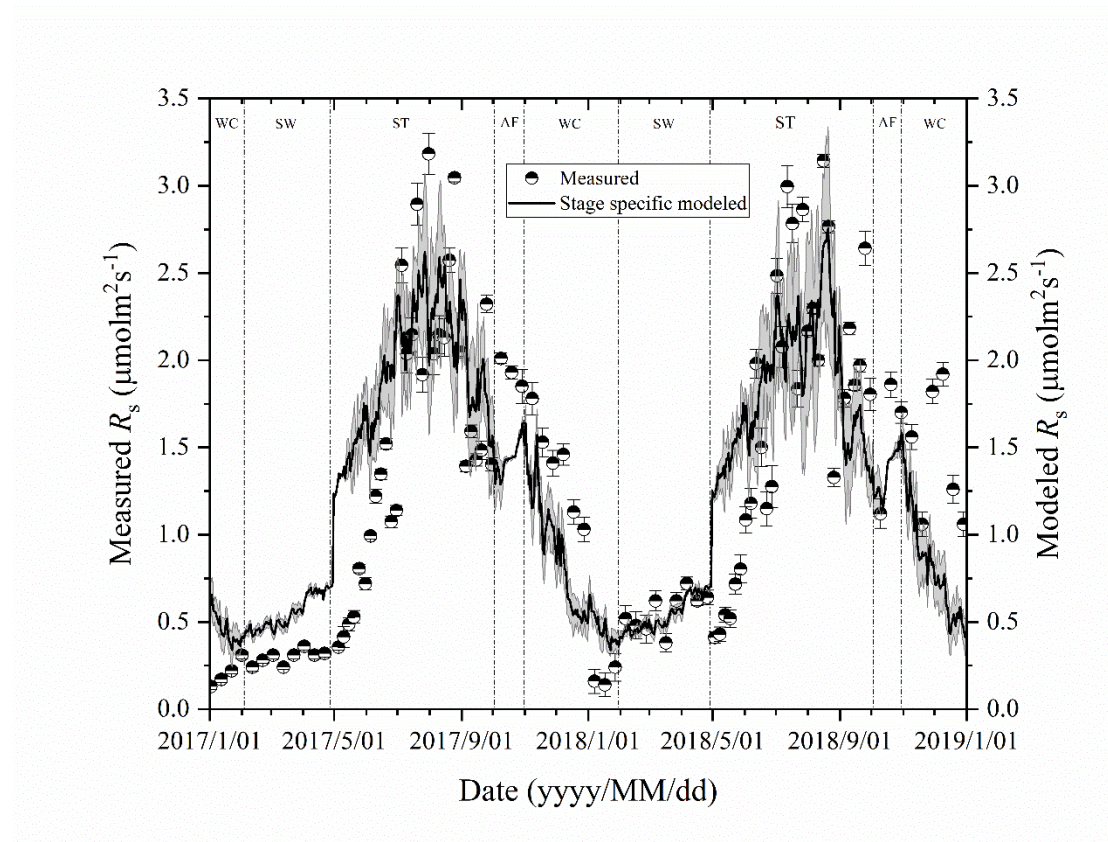
Fig.3. Variations of measured and modeled R_s fluxes at different freeze-thaw stages in 2017 and 2018. Error bars represent standard error of measured R_s ( n=6 )
