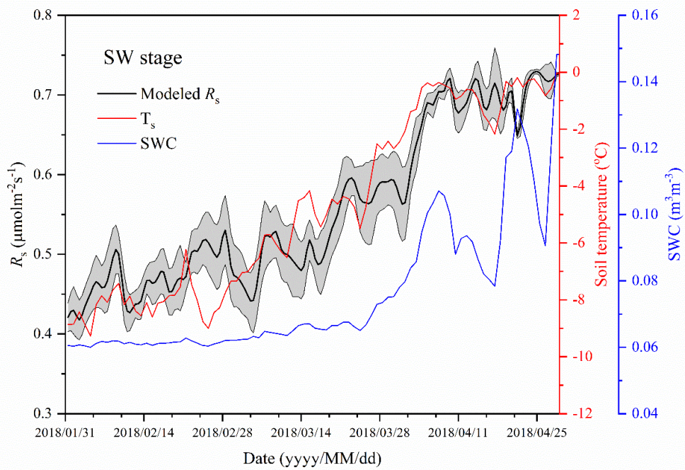
Fig.6. Variations in modeled soil respiration ( R_s ), soil temperature ( T_s ) and soil water content (SWC) for the four freeze-thaw stages including summer thawing stage (ST), autumn freezing stage (AF), winter cooling stage (WC), and spring warming stage (SW) in a complete freeze-thaw cycle from late April 2017 to late April 2018. The SWC unit stands for water volume per total soil volume. The error band of modeled R_s stands for 95% confidence interval.
