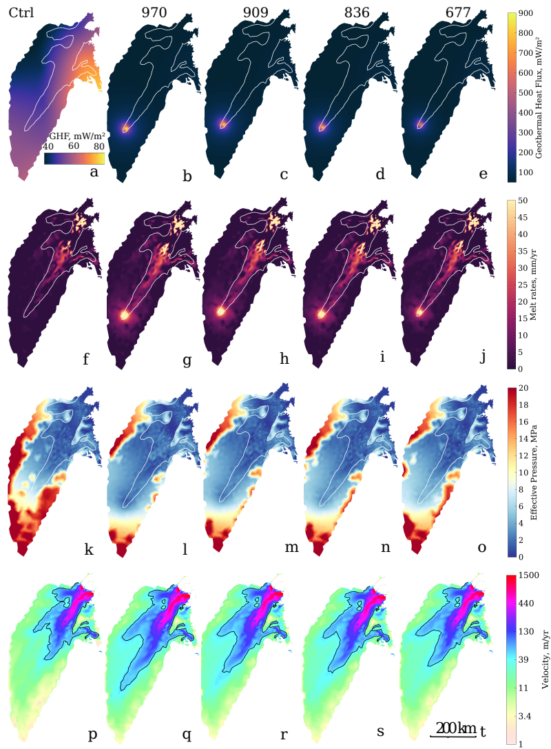
Figure 2. Model results for the Ctrl and the plume677, plume836, plume909 and plume970 simulations. a-e show the modelled geothermal heat flux-GHF (note the different color scale for Ctrl) and f-j shows the corresponding basal melt rates, forcing the hydrology model which computes the corresponding effective pressure (k-o) and finally the resulting surface velocity (p-t). White lines show the 50 m yr -1 observed velocity contour, and black lines show the 50 m yr -1 modelled velocity contour.
