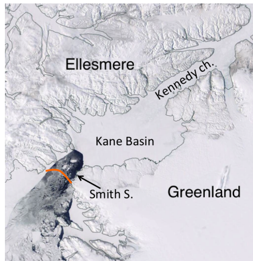
Figure 1. NASA Worldview image of a stable landfast ice arch in Nares Strait, from Moderate Resolution Imaging Spectroradiometer (MODIS) Corrected Reflectance imagery (True Color), on May 1st 2018. The orange curve indicates the position of the stable ice in (Dansereau et al., 2017)
