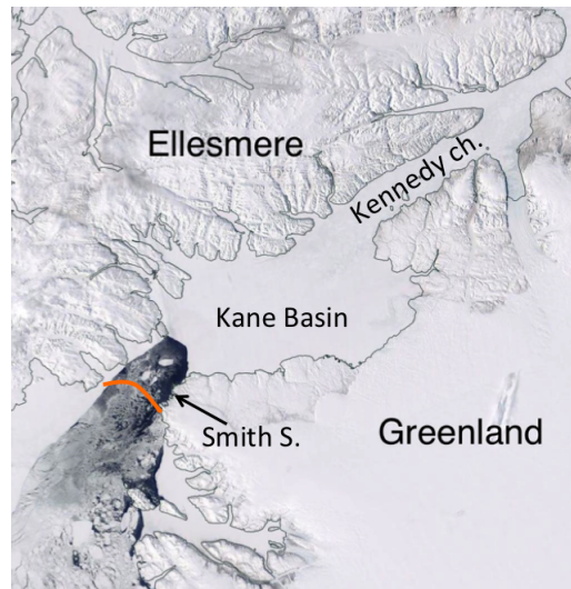
Figure 1. NASA Worldview image of a stable landfast ice arch in Nares Strait, from Moderate Resolution Imaging Spectroradiometer (MODIS) Corrected Reflectance imagery (True Color), on May 1st 2018. Orange curves indicate The orange curve indicates the position of the stable ice arch in (Dansereau et al., 2017)
