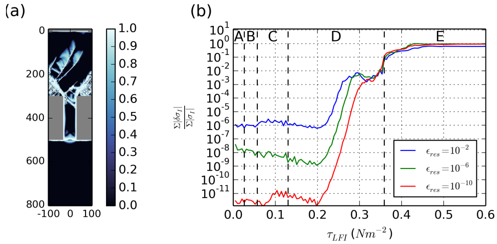
Figure 14. a) Asymmetries dominating the damage fields after the ice bridge collapse (Stage E) in Fig. 4). b) Evolution of normalized, domain-integrated asymmetries in the \sigma_I field when using different residual tolerance \epsilon_{res} on the solution. Dashed lines indicate the beginning and end of the simulation phases (A,B,C,D,E).
