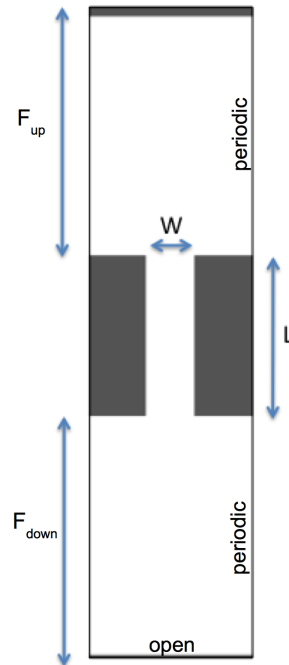
Figure 3. Idealized domain with a solid wall to the north, open boundary to the south and periodic boundaries to the East and West. The channel in the control simulation has a width W \approx 60 \text{ km} , length L \approx 200 \text{ km} and fetch F_{up} and F_{down} \approx 300 \text{ km} in the upstream and downstream basins respectively.
