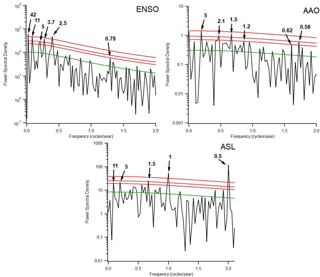
Figure 8. Spectral analysis of the rBC concentrations and comparison with existing datasets (Sentinel Hotspots Australia, ASL, AAO and ENSO indexes). Numbers in bold indicate cycle frequency, in years. Red lines are confidence intervals 99% (top), 95% (middle) and 90% (bottom). Green line indicates AR1 red-noise background. The question mark in the Australian fire spots spectrum indicates a longer, unidentified cycle.
