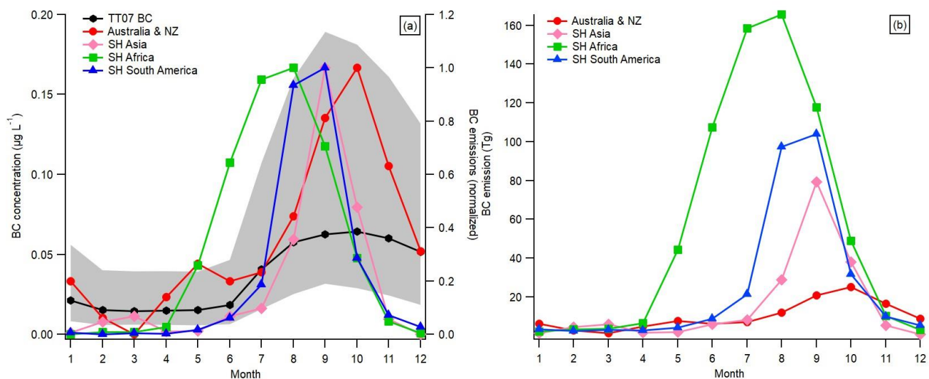
700 Figure 7(a). TT07 rBC (monthly averages, 1968-2014) and BC emissions estimated from GFED4s for the four SH regions (normalized, 1997-2014). The shaded area represent 1 geometric standard deviation of monthly rBC values. (b) Absolute BC emissions estimated from GFED4s for the SH.
