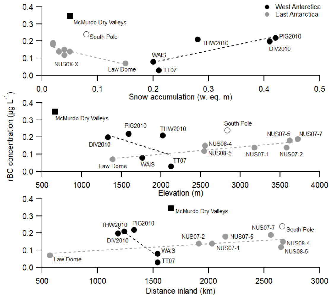
695 Figure 6. rBC records from Antarctica. rBC concentrations plotted against snow accumulation, elevation and distance from the sea. Solid lines indicate statistically significant correlations ( p < 0.05 ), while dashed lines indicate not significant correlations ( p > 0.05 ).
