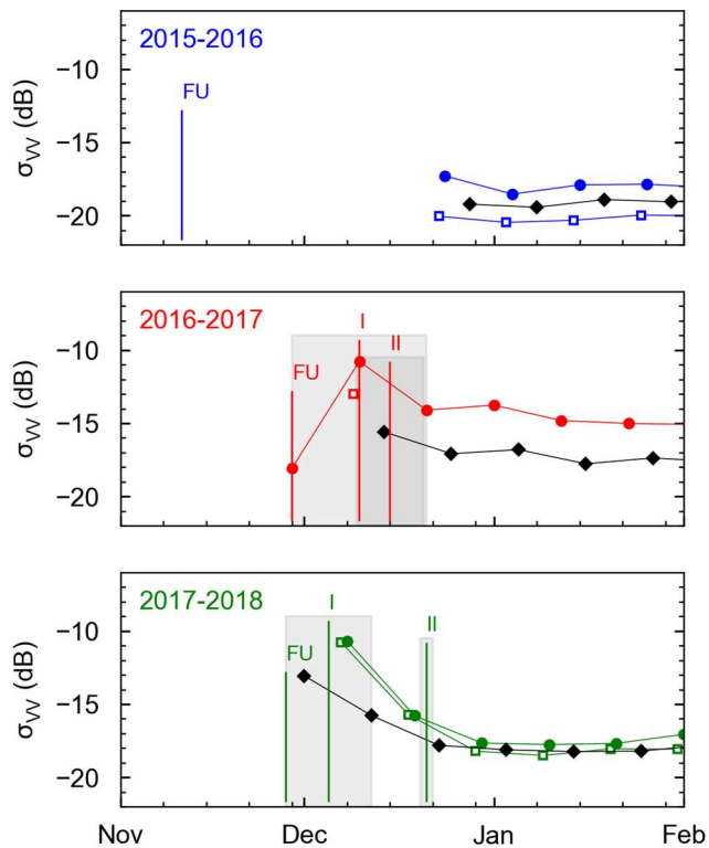
290 Figure 9: TerraSAR-X median VV backscattering is plotted versus time for each year (color-coded). Three orbits are shown for: orbits 13 (empty square), 21 (circle), and 89 (black diamond). The freeze-up date (FU, from time-lapse photography), the post-freeze-up peak (I, from TerraSAR-X), and the beginning of monotone X-band (II, from TerraSAR-X) are identified with vertical bars. Estimates for each indicator are indicated by shaded grey areas.
