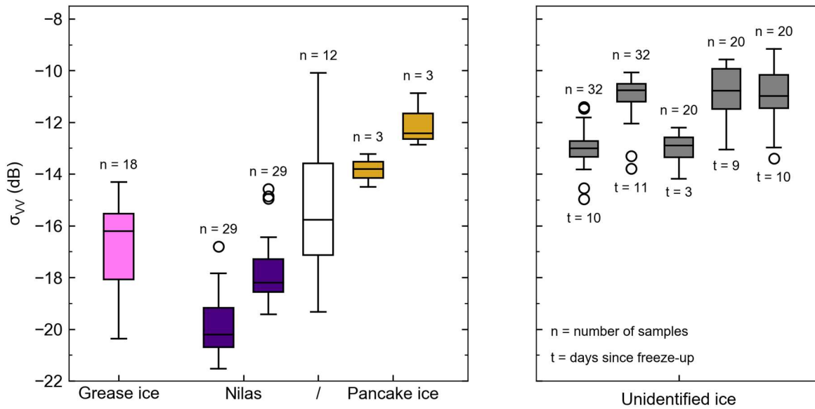
270 Figure 8: TerraSAR-X median VV backscattering values observed over AOIs of ice types identified from time- lapse photography in 2016 and 2017. The number of median values used (n) is written above each box. Outliers are plotted as empty white circles. Left: Grease ice (pink) was observed on the orbit 13 image from 26 November 2017. Nilas (dark purple) was observed on 28 and 29 November 2016 in orbits 13 and 21, respectively. A mix of nilas and pancake ice (white) was observed on 26 November 2017 in orbit 13. Pancake ice (yellow) was observed on 28 275 and 29 November 2016 in orbits 13 and 21. Right: Unidentified young ice (grey) was observed on 9 and 10 December 2016 in orbits 13 and 21, as well as on 1, 7 and 8 December 2017 in orbits 89, 13, and 21. The number of days since the freeze-up date (t) is written below each box.
