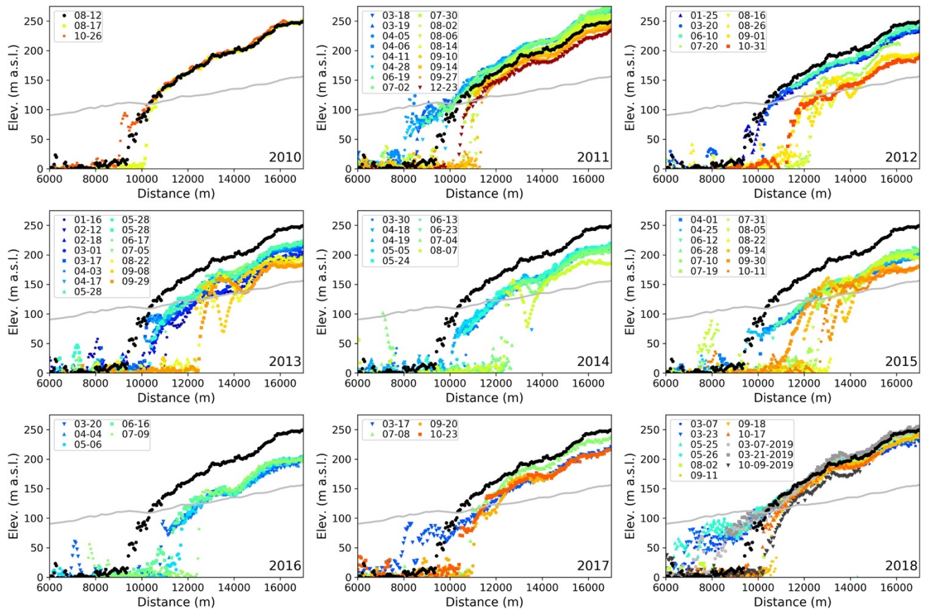
745 Figure 3. Plots for each year from 2010 through 2018 showing the available near-terminus elevation profiles, with three 2019 profiles included in the 2018 plot (see Fig. S2 for separate 2018 and 2019 plots). Profiles are labelled by date (MM-DD) and the profile location is shown in Fig. 1. For reference, the initial 2010 profile (2010-08-12) is included in each plot. All elevations are relative to nominal mean sea-level (EGM2008 geoid). The grey line indicates the flotation height as estimated using bed elevations (Fig. S1) from BedMachine v3 (Morlighem et al., 2017).
