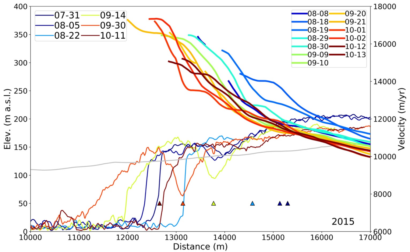
775 Figure 7. Elevation and velocity profiles for summer 2015 illustrating the evolution of an advecting transverse surface depression. The legends give the nominal dates (MM-DD) in 2015. As in Fig. 3, the grey line indicates nominal height of flotation. The triangles show the estimated locations (see text) of parcel of ice that evolved to form the bottom of the depression discussed in the text (see also white circles in Fig. 8), which served as a detachment point for a calving event(s) that occurred between September 30 and October 11.
