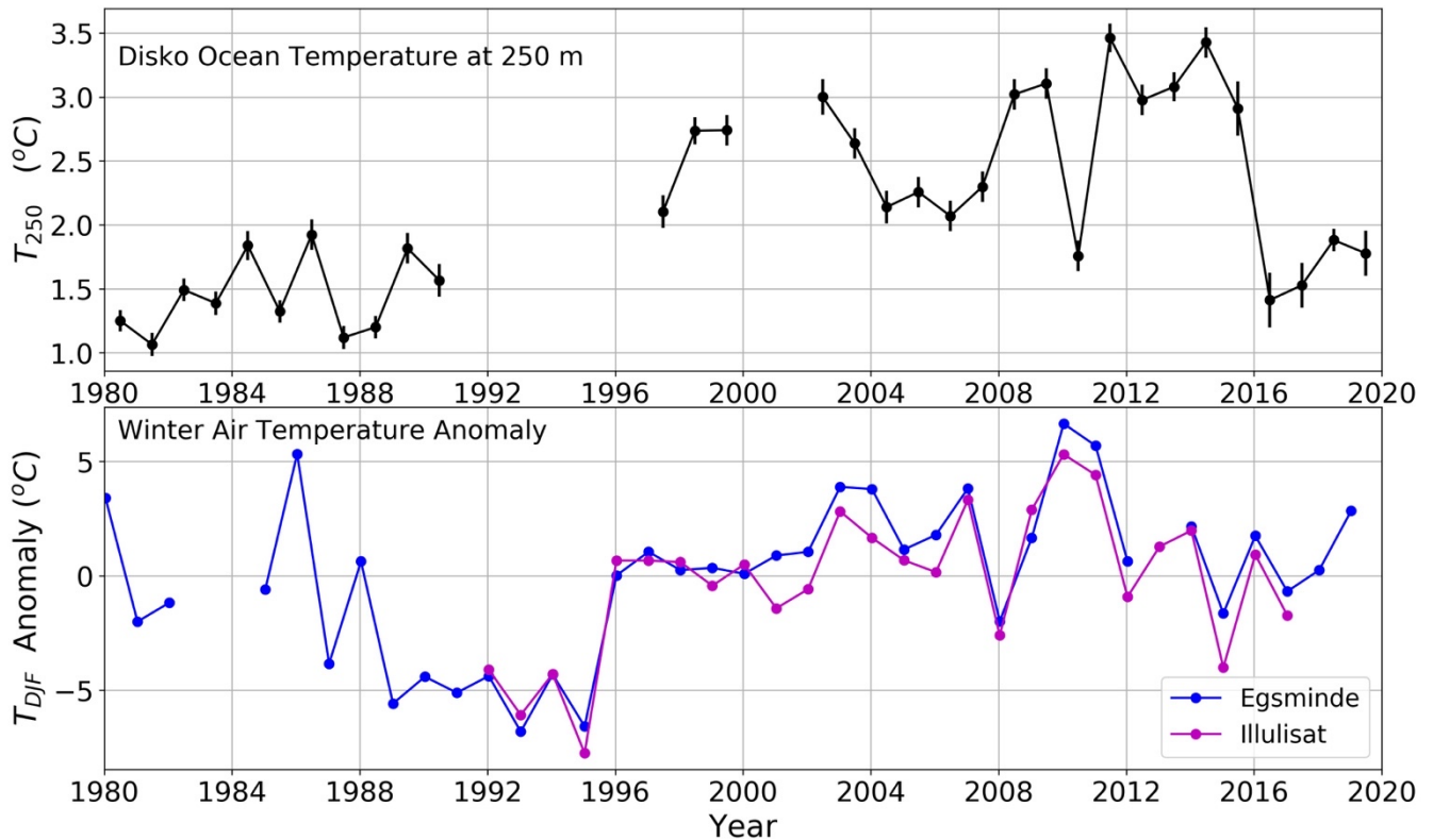
765 Figure 6. (top) Ocean temperatures at 250-m depth in Disko Bay (all available casts in the region: 68.6^\circ < \text{latitude} < 69.4^\circ , -54^\circ < \text{longitude} < 52^\circ ), which is based on a similar figure by Khazendar et al. (2019). Small differences with their results exist based on the sampling region and the averaging scheme. The ocean temperatures for 2015–2019 are extracted from the Ocean Melting Greenland data set ( https://doi.org/10.5067/OMGEV-AXCTD ) and for 1980–2014 are extracted from the International Council for the Exploration of the Sea Oceanography ( http://www.ices.dk/marine-data/data-portals/Pages/ocean.aspx ) database. To obtain estimates representative of 250-m depth, we averaged temperatures from 225 to 275 m depth. The bars indicate uncertainty in the mean based on the number of points in the sampling region. To compute them, we take the mean intra-annual standard deviation averaged over the full record as the intrinsic uncertainty for a single point (i.e., how representative a point measurement is for the entire region). We then scale this value by 1/\sqrt{\text{number of points}} to determine the plotted bar for each annual mean. (bottom) Winter 2-m air temperature (D-J-F) anomalies relative to the mean for the period from weather stations in Egsminde and Illulisat (GISTEMP Team 2019, 2019). 770
