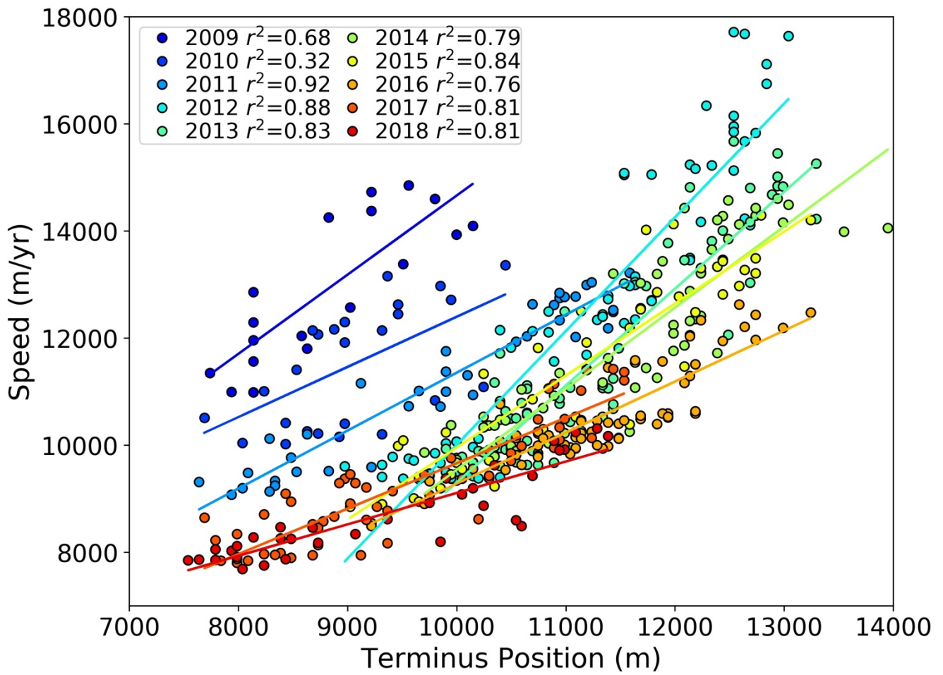
760 Figure 5. Speed at T_{\max}-1 km (see grey points Fig. 1) as function of terminus position (relative to the profile shown in Fig. 1) for each year from 2009 to 2018, with greater terminus positions indicating greater retreat. Lines show linear regressions for each year with r^2 values included in the legend.
