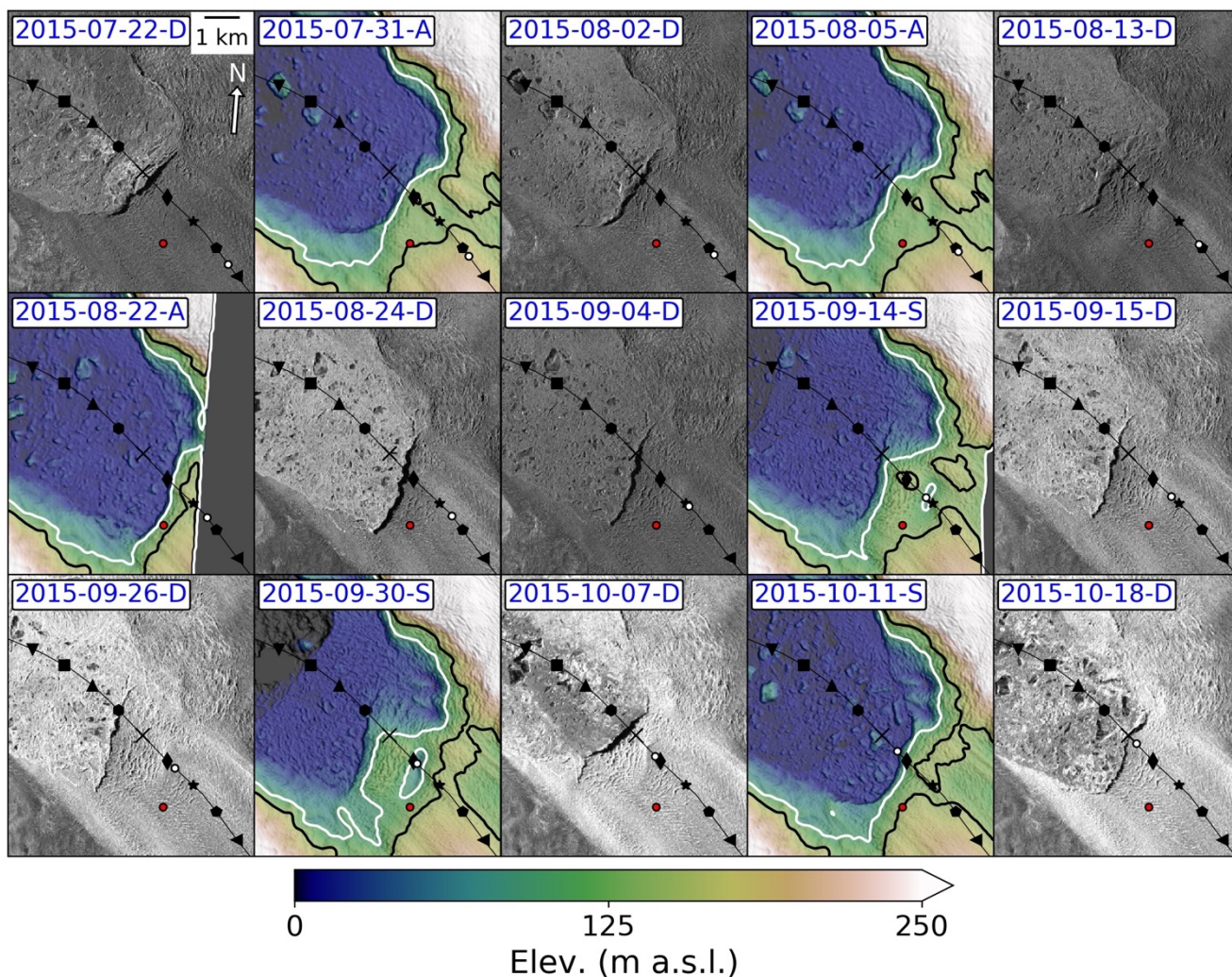
Figure 8. Time series of TerraSAR-X SAR backscatter amplitude imagery and colour shaded relief maps for late summer 2015 identified by date of acquisition (YYYY-MM-DD). The source of the data in each map is indicated by the letter after each date (D: TerraSAR-X images copyright DLR 2015, A: ASP World View DEM, S: SETSM World View DEM). The artificial illumination source for the DEM shaded surfaces was chosen to approximate the illumination angle of the TerraSAR-X radar. Note that the terminus in the radar imagery casts a true shadow, while the corresponding shadows in the shaded relief maps are based on the local slope/aspect. The red circle shows the location of M6, while the white circle tracks the parcel of ice that evolved to form the depression (e.g. September 30) described in the text (see also triangles Fig. 7).
