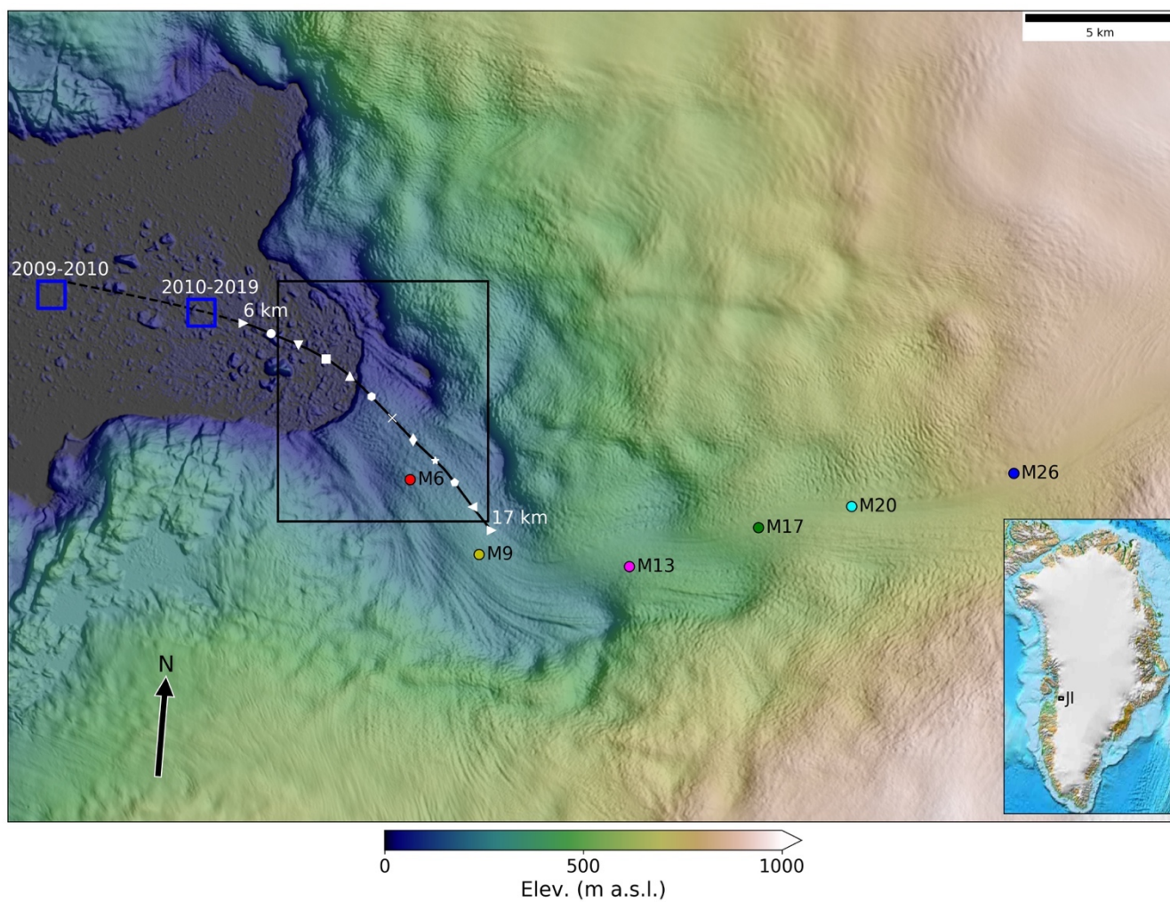
Figure 1: Surface elevation (colour) over shaded relief map derived from the Greenland Ice Mapping Project (GIMP) DEM for the region near the terminus of Jakobshavn Isbrae (see inset for location). The black box shows the location of the images shown in Figs. 4 and 8 and the blue box indicates the areas used to sample mélange as described in the text. The solid black line shows the location of the profile shown in Figs. 3 and 7, with the dashed section used to show the full extent. White markers with assorted symbols denote 1-km intervals along the profile between 6- and 17-km. Coloured markers (M6-M26) show where speed is sampled in Fig. 2 at points consistent with earlier work (Joughin et al., 2008b; 2012b; 2014).
