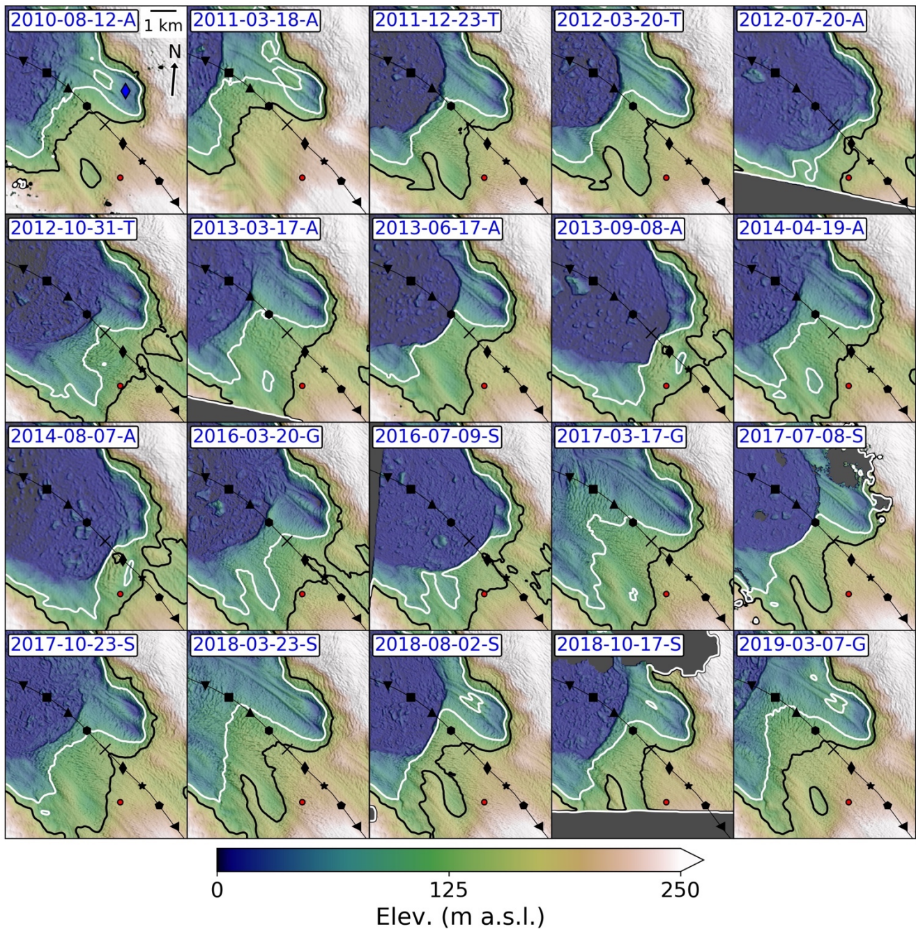
Figure 4. Colour shaded relief maps for a subset of DEMs, excluding maps for 2015, which are included in Fig. 8. Elevation contours of 150 (black) and 100 (white) meters bound the approximate transition from grounded to floating ice. The elevation data were lightly smoothed prior to contouring to eliminate crevasse noise. The letter after the date-string (YYYY-MM-DD) indicates the DEMs source (A: ASP World View, T: TanDEM-X, S: SETSM World View, and G: GLISTIN). The profile with symbols every 1-km is the same as shown in Fig. 1 and the red dot shows the location of M6. The blue diamond in the 2010-08-12 panel is referenced in the text.
