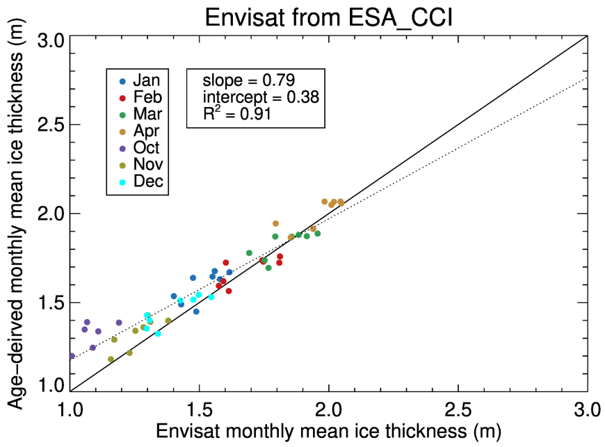
675 Figure 10: Scatterplot of IceAgeDerived and Envisat monthly mean ice thickness, where Envisat data are from ESA CCI. Dashed line represents the regression line of IceAgeDerived monthly mean ice thickness on the Envisat data, with the slope, intercept, and R^2 indicated.
