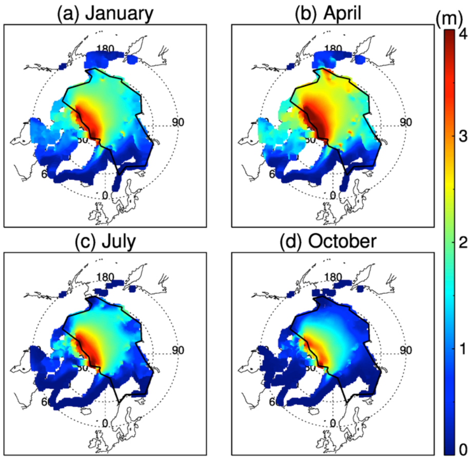
740 Figure A2: Derived climatological mean sea ice thickness distribution in the Arctic from PIOMAS, 1984 to 2018.
