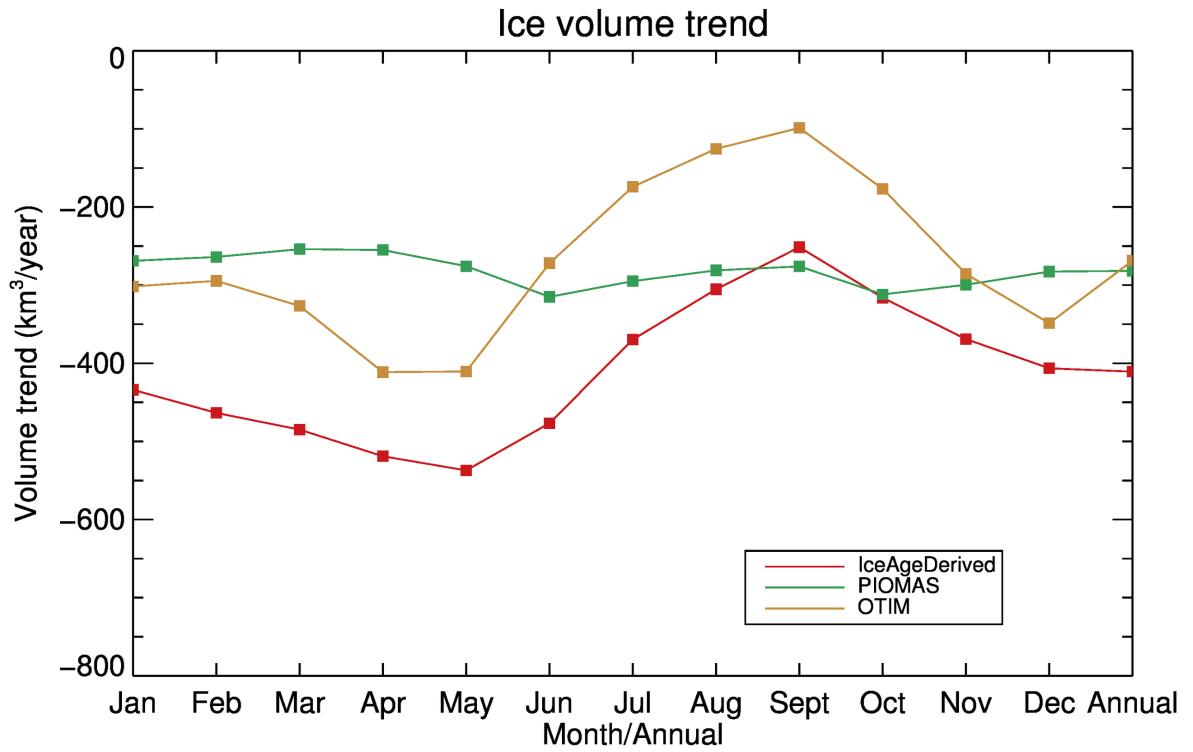
715 Figure 19: Trend of Arctic ice volume in each month and in the annual mean from 1984 to 2018 derived from ice age, PIOMAS, and OTIM over the Arctic Ocean.
