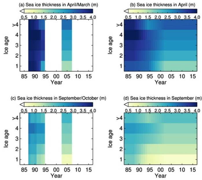
635 Figure 2: Observed relationship of ice age and ice thickness from 1988 to 1995 from submarine data in April (a) and September (c), and from 2004 to 2008 from ICESat in March (a) and October (c), and derived relationship of ice age and ice thickness from 1984 to 2018 in April (b) and September (d).
