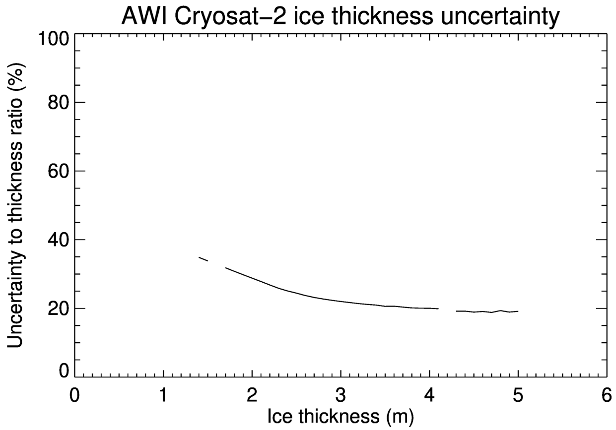
735 Figure A1: The percentage of uncertainty to sea ice thickness in AWI CryoSat-2 monthly mean ice thickness 2011-2018.
