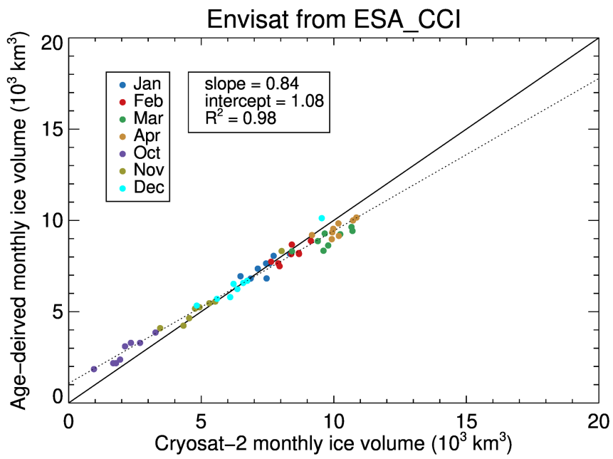
Figure 11: Same as Figure 10 except for ice volume.
