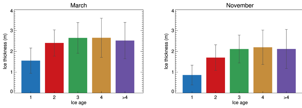
Figure 12: Ice age versus ice thickness from collocated ice age and AWI CryoSat-2 ice thickness. The error bar shows one standard deviation above and below the mean ice thickness in each ice age category.
