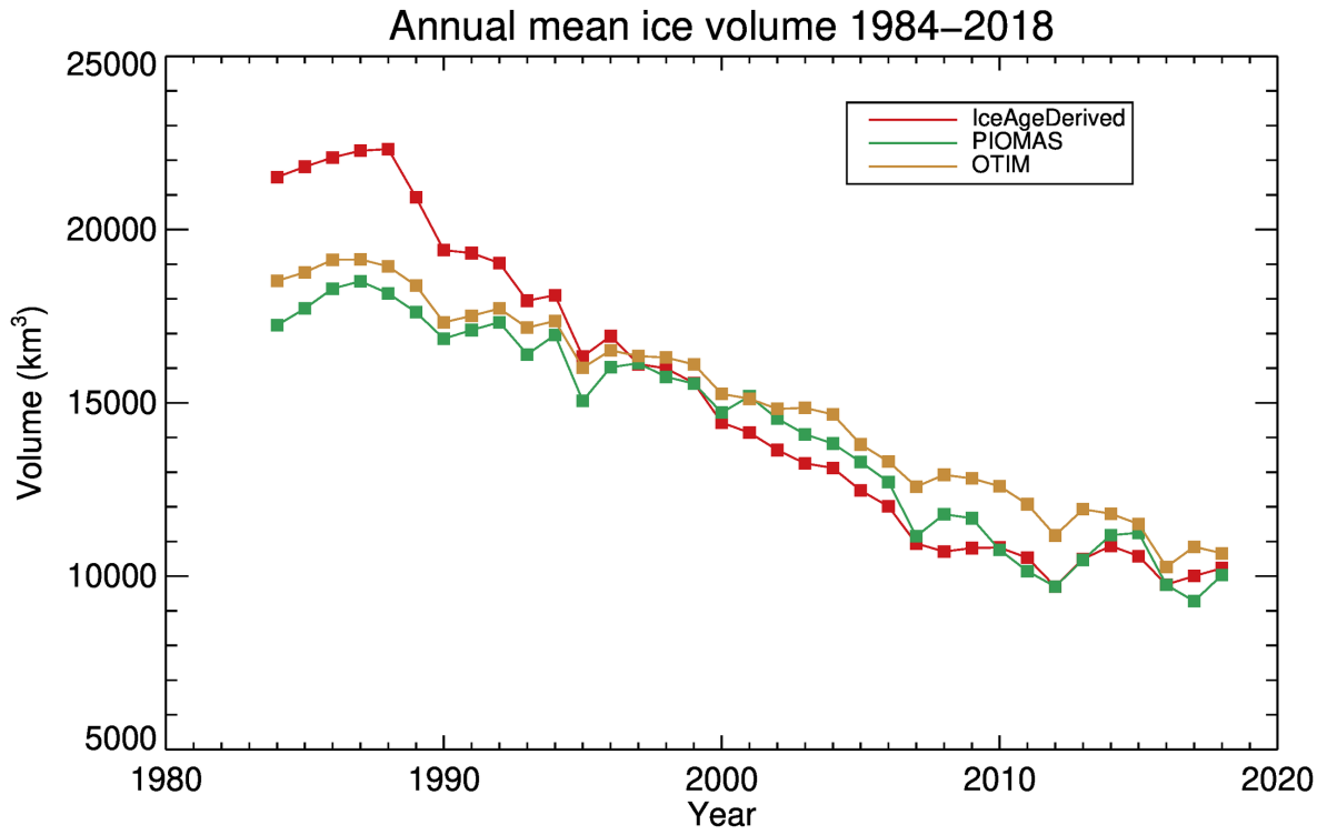
710 Figure 18: Time series of annual mean Arctic ice volume from 1984 to 2018 derived from ice age, PIOMAS, and OTIM over the Arctic Ocean.
