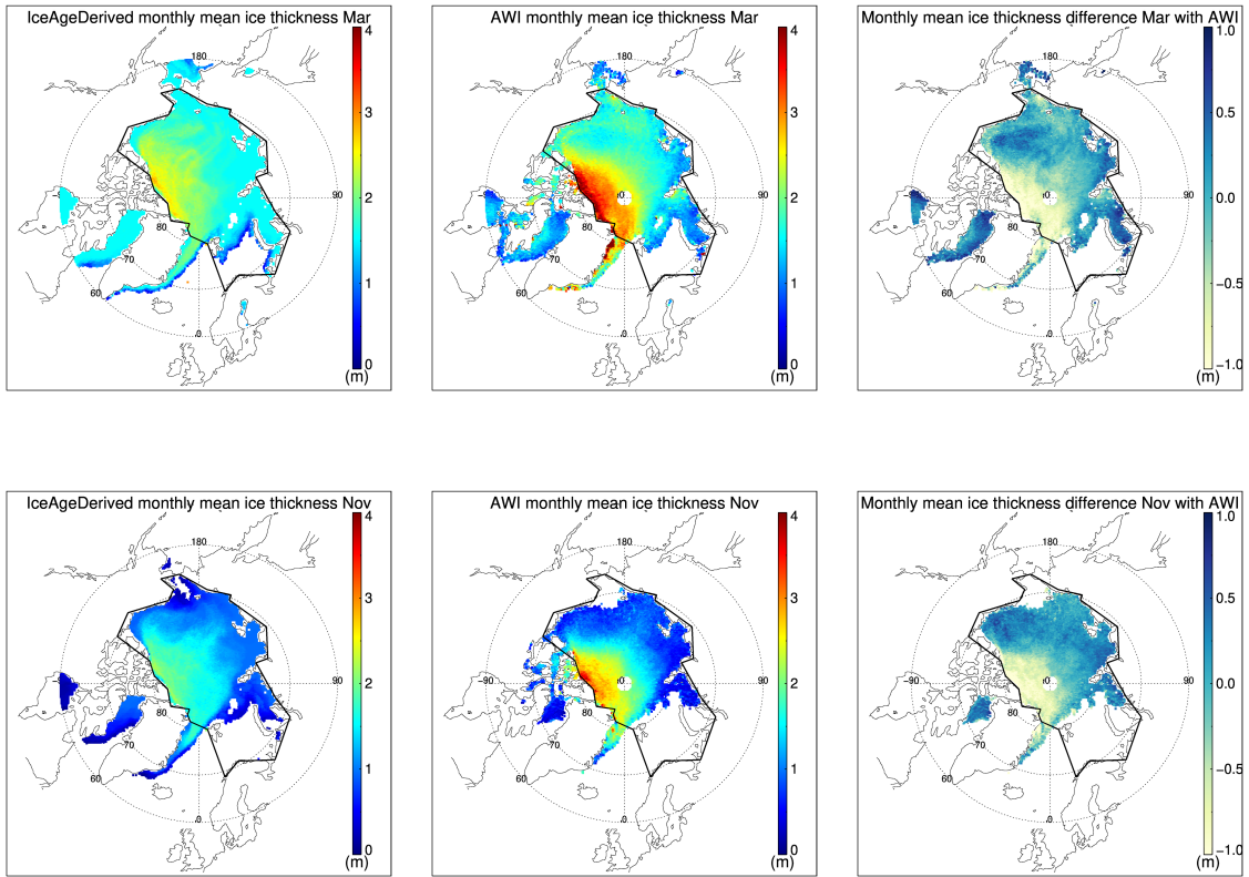
Figure 9: Monthly mean ice thickness from IceAgeDerived (top left), from AWI CryoSat-2 (top middle), and their difference in March 2011-2018; and monthly mean ice thickness from IceAgeDerived (bottom left), from AWI CryoSat-2 (bottom middle), and their difference in November 2011-2018.
