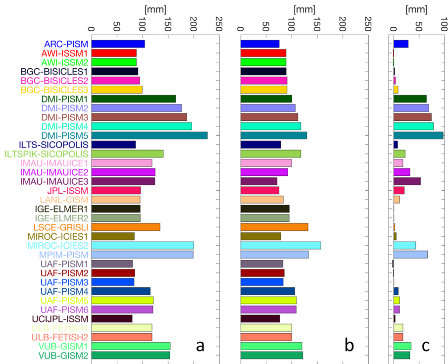
Figure 12 Sea-level contribution in 2100 derived by integrating a transient aSMB over the initial ice mask of each initMIP-Greenland model, (a) without remapping, but extension to the modelled ice sheet extent, (b) with remapping to the initial surface elevation of each individual model and (c) difference (a)-(b).
