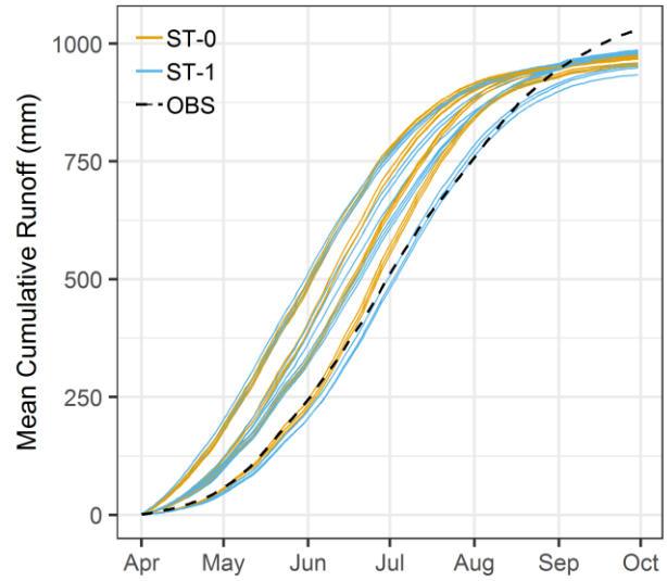
(b) Secondary Control on Snowpack Runoff - Stability Adjustment Option
