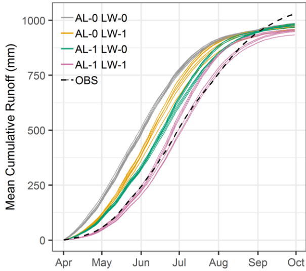
(a) Primary Controls on Snowpack Runoff - Albedo and Liquid Water Combinations
