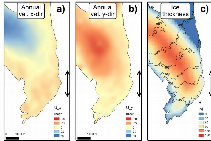
Figure S1. Components required for calculating ice emergence rate. The zone of maximum thinning ( ZMT ) is defined by the double-headed arrow in each panel. a) Mean annual velocity in the x direction. Positive is to the right and negative to the left b) Mean annual velocity in the y direction. Positive is for flow towards the top of the figure and negative is for flow towards the bottom c) Ice thickness estimated across the study area based on Huss and Farinotti (2012). Note that we did not calculate the emergence rate for Root glacier (blue area at the upper end of the panel).
