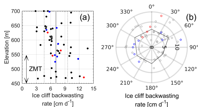
Figure 7. Ice cliff backwasting rate measurements. Ice cliff backwasting rates are corrected for the different measurement periods (Sect. S1.2). Cliffs with streams at their base are blue. Cliffs with ponds at their base are red. (a) Ice cliff backwasting rate as it varies with elevation. The solid grey line is the mean of all data 7.1 \text{ cm d}^{-1} . The dashed lines are \pm 1\sigma bounds used in the distributed melt calculations. The double-headed arrow represents the zone of maximum thinning (ZMT). (b) Ice cliff backwasting rate as it varies with aspect. The corners in the solid black line represent the mean backwasting rate from 60^\circ bins. During the field survey, ice cliffs with ponds at their base were only found facing northward (between 300 and 30^\circ ).
