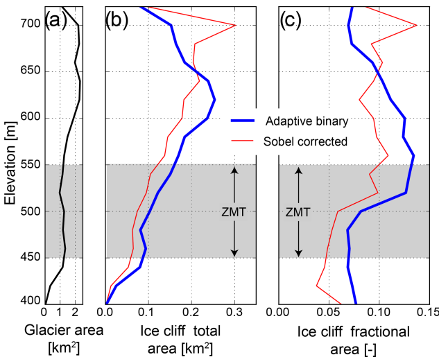
Figure 10. Results from the two ice cliff delineation methods with elevation. All panels use 20 m elevation bins. (a) Glacier area as a function of elevation. (b) Ice cliff area as a function of elevation. The red line shows results from the SED approach after false positives on dark-colored ice are removed. (c) Ice cliff area as a function of elevation, normalized by the glacier area within each elevation band. Note that fractional area \times 100 is the percentage of ice cliff coverage.
