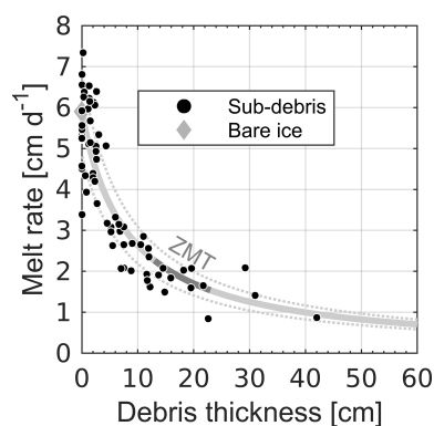
Figure 6. Sub-debris melt rate measurements. Melt rate as it varies with debris thickness. Sub-debris melt rates are corrected for the different measurement periods (see Sect. S1.1). The solid line is the curve fit using the hyper-fit CE2 model for the best debris thickness–melt CE3 relationship (RMSE of the data is 0.8 \text{ cm d}^{-1} ). The portion of the best curve fit in the zone of maximum thinning (ZMT) is shaded darker than the rest of the line. The dotted lines represent the \pm 1\sigma error bounds used in the uncertainty estimates of distributed melt.
