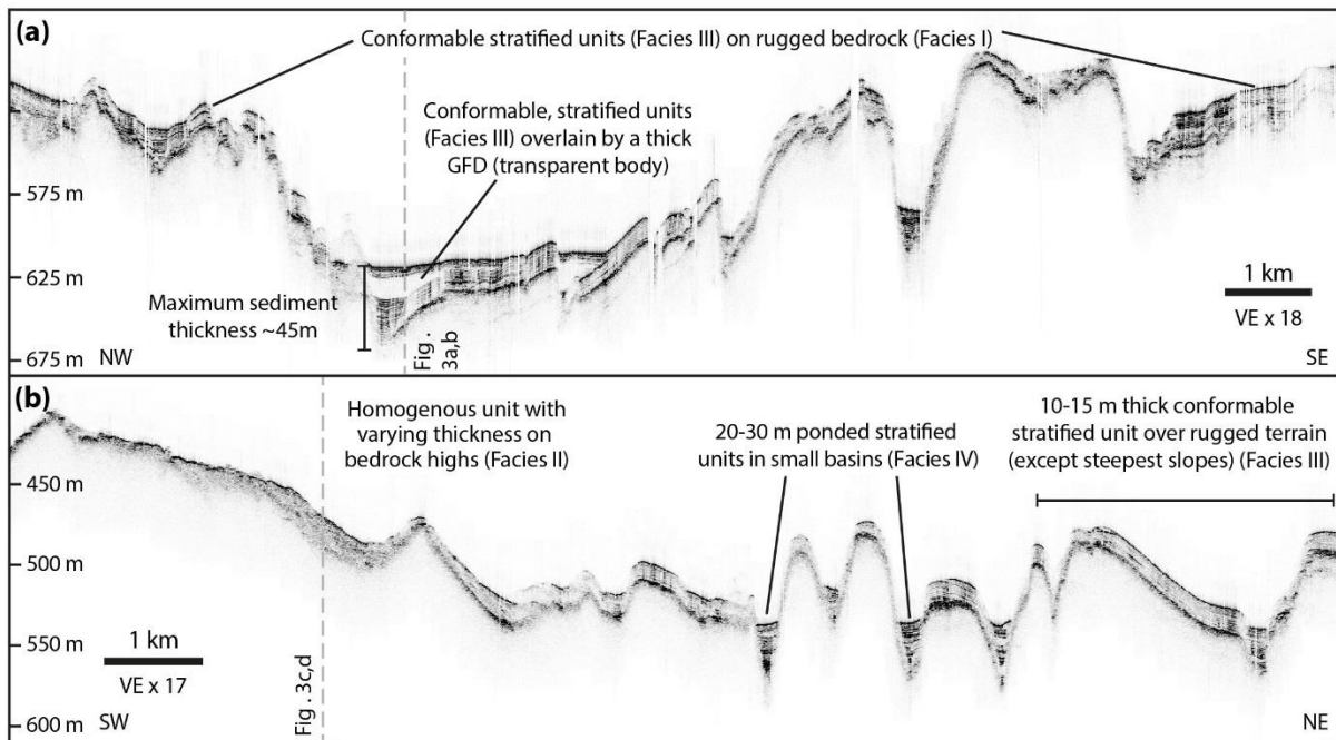
1045 Figure 8. Examples of SBP profiles from Hall Basin, Nares Strait (see Fig. 2 for locations). (a) NW-SE profile in Hall Basin showing bedrock topography ( Facies I ) mantled with conformable sediment ( Facies III ) and ponded basin fill, sometimes with significant GFDs in local depressions ( Facies IV ). (b) A SW-NE profile between the Petermann sill and S1 high showing a similar stratigraphy but including non-conformable, homogenous sediment on steep slopes ( Facies II ). Intersections with Figs. 3a-d are marked with vertical grey dashed lines.
