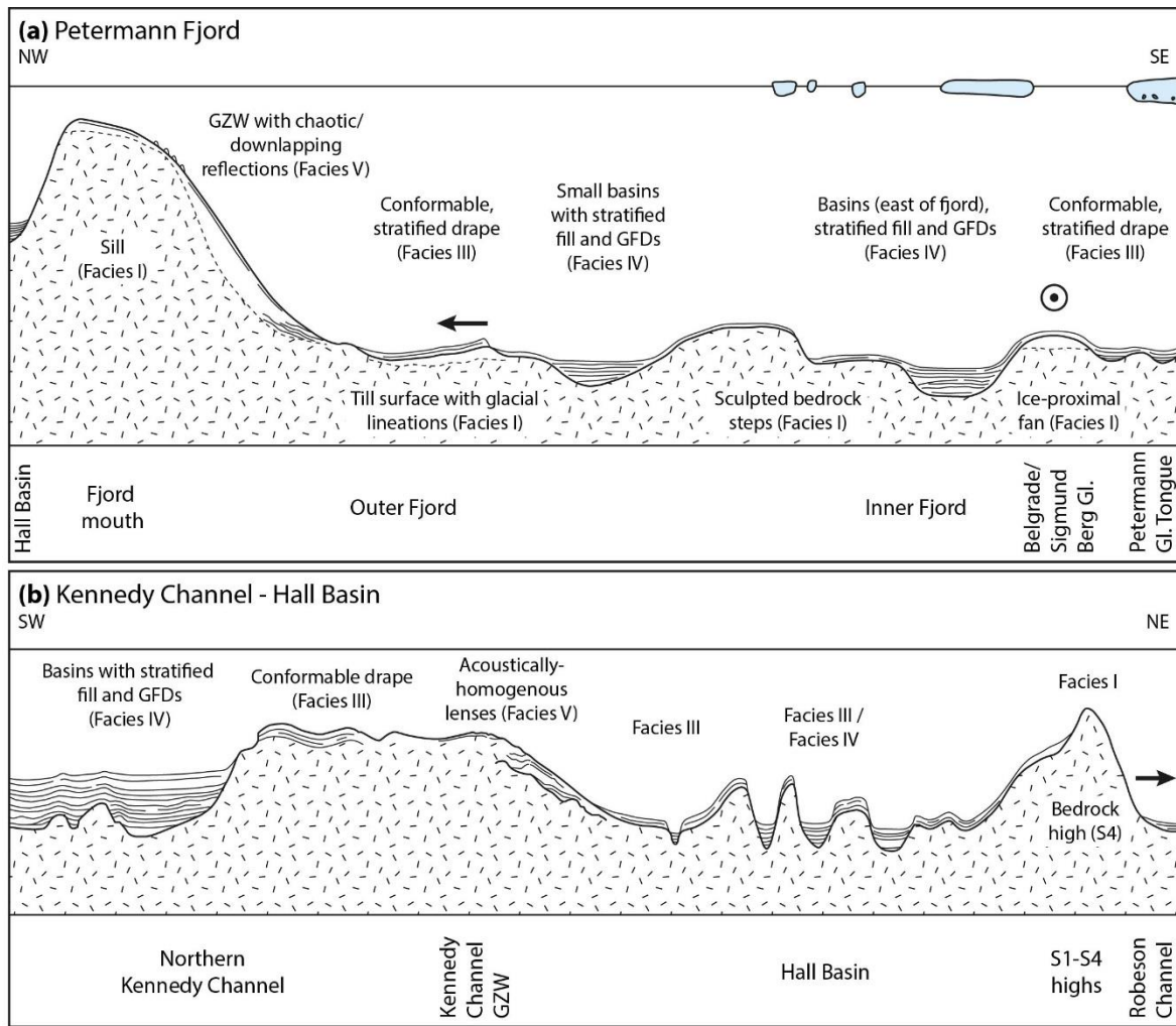
Figure 12. Conceptual transects showing the seismic stratigraphy and distribution of glacial marine sediments in the Petermann Fjord-Nares Strait area. (a) Petermann Fjord with the fjord-mouth sill with GZW on the left side; localized sediment input into the NE side of the fjord from tributary glaciers and building an ice-proximal fan is shown as the bullseye. (b) Deglacial sediment cover in Nares Strait from Kennedy Channel to Hall Basin to Robeson Channel. Not to scale. Black arrows show the former ice flow direction through the system.
