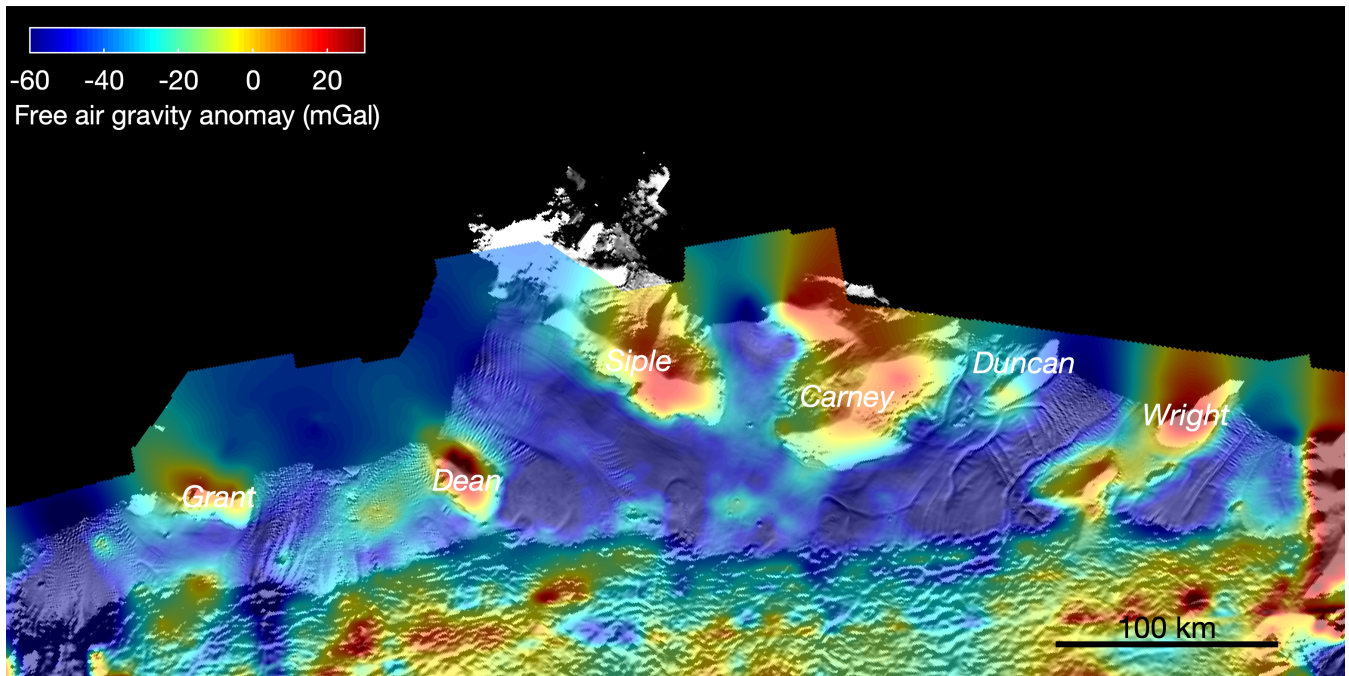
Figure 2. The free air gravity anomalies over Getz Ice Shelf. Lines of gravity data is shown in Figure 1 of the main text. The background image is MODIS-derived Mosaic of Antarctica (Scambos et al., 2007).
