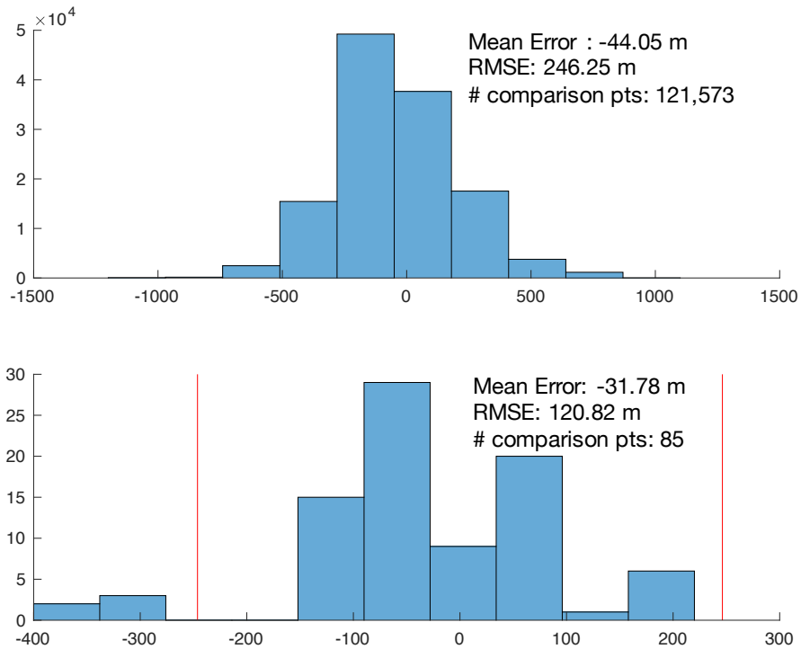
Figure 4. Uncertainty estimation using known ice bottom elevations. The top panel is the histograms with the Mean Error and Root Mean Square Error between inverted and measured ice bottom elevation over grounded ice survey lines. The bottom panel shows the histogram with the Mean and Root Mean Square Error between inverted bathymetry and known ship measured bathymetry from ship track (Nitsche et al., 2007). The two vertical red lines are RMSE = \pm 246.25 m.
