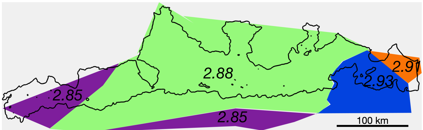
Figure 3. The selected bulk density values used in the final bathymetry inversion. The unit of the label number is \text{kg} \cdot \text{m}^{-3} .
