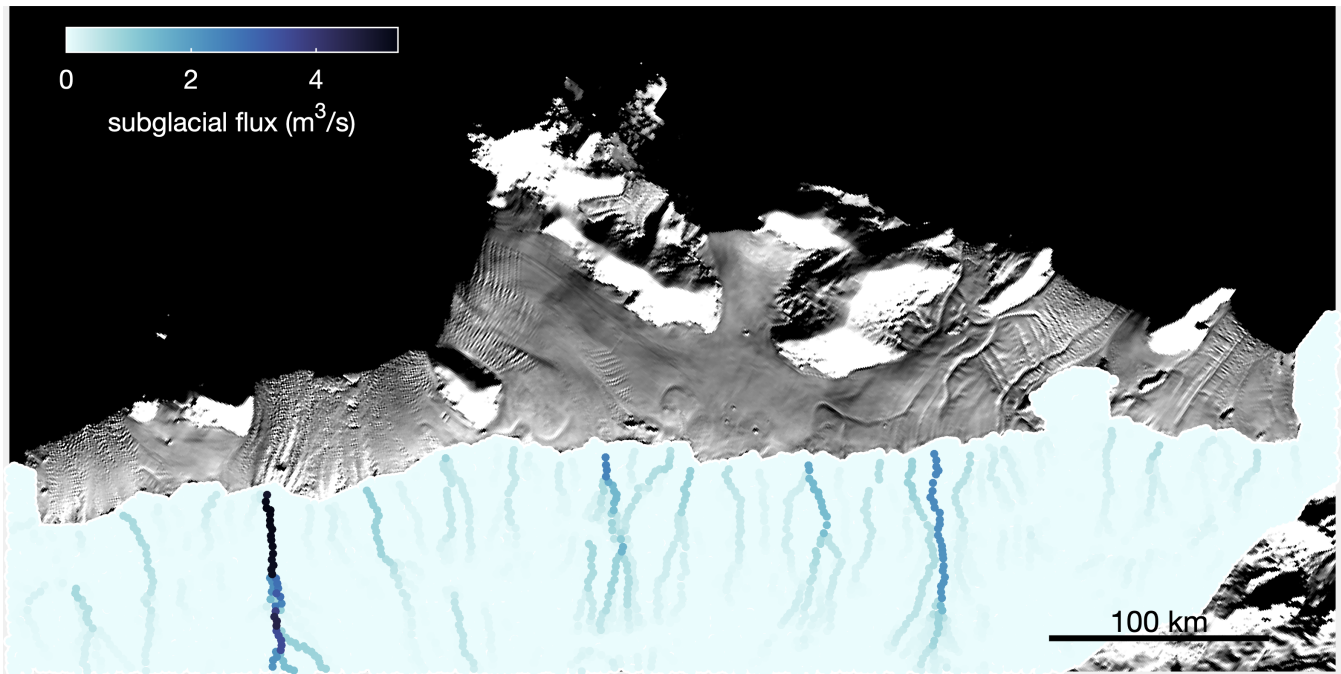
Figure 6. Surface channels over Getz Ice Shelf line up with the channel outlets. The background image is MODIS-derived Mosaic of Antarctica (Scambos et al., 2007).
