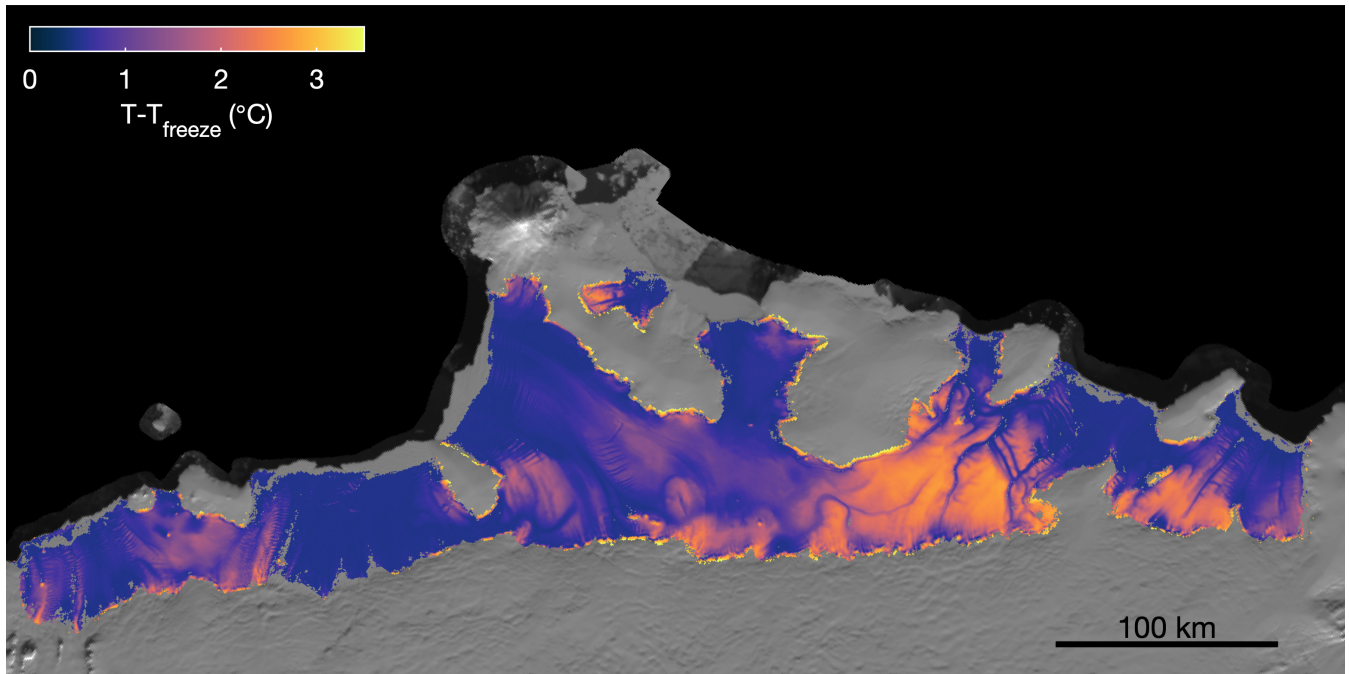
Figure 5. Local temperatures above freezing at depths corresponding to the ice shelf base. Temperatures are interpolated from the mean profile of 25 CTD casts (Locarnini et al., 2013) acquired at the Getz Ice Shelf front.
