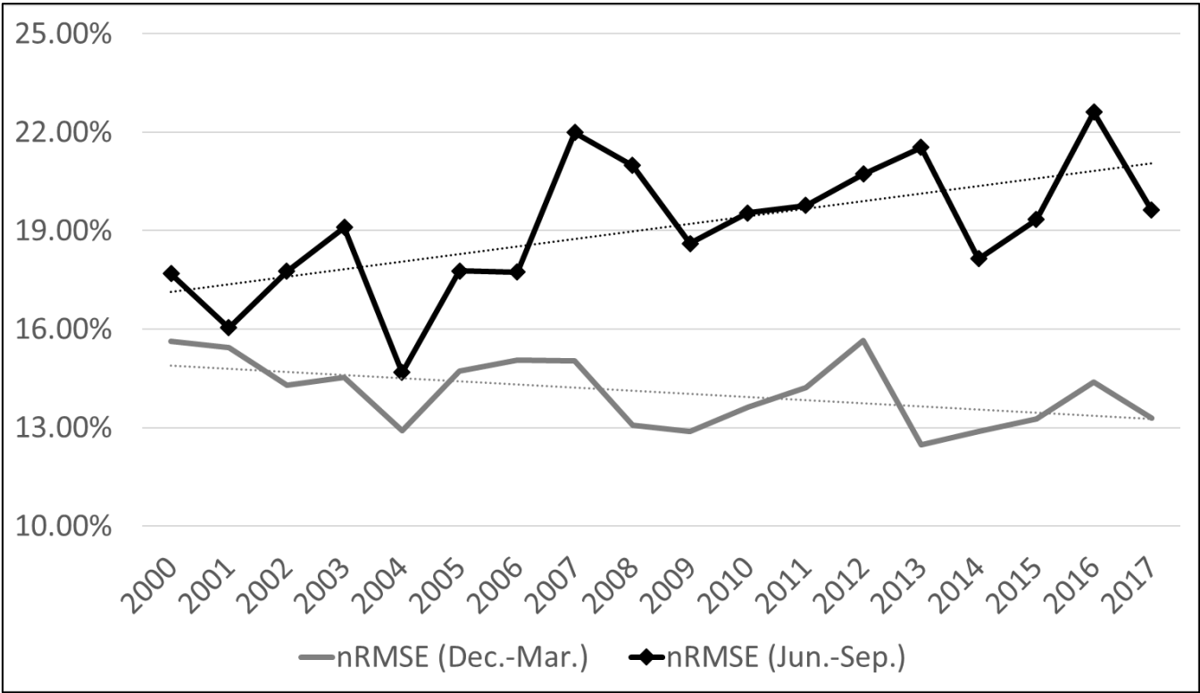
Figure 7. Changes of prediction accuracy (nRMSE) using CNN model in freezing (Dec.-Mar.) and melting (Jun.-Sep.) season (2000-2017, dotted lines show trend).
