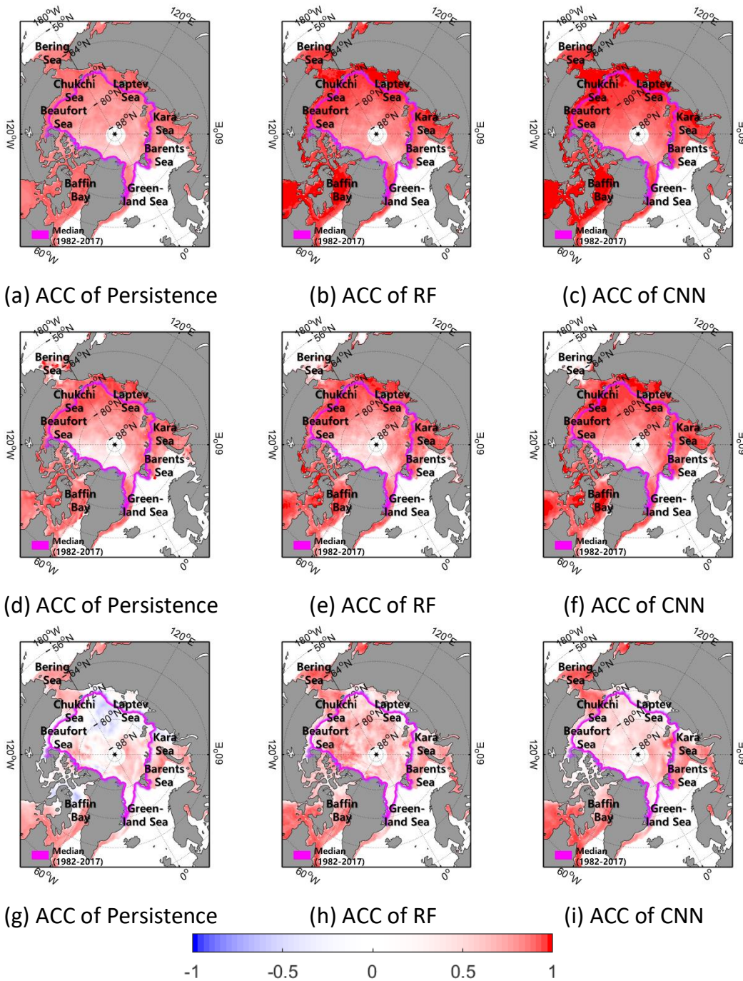
305 Figure 3. The temporal ACC of the persistence (a), RF (b) and CNN (c) during 2000-2017. As in (a) - (c), but for the melting (Jun. – Sep.) and freezing (Dec. – Mar.) seasons, (d) - (f) and (g) - (i), respectively.
