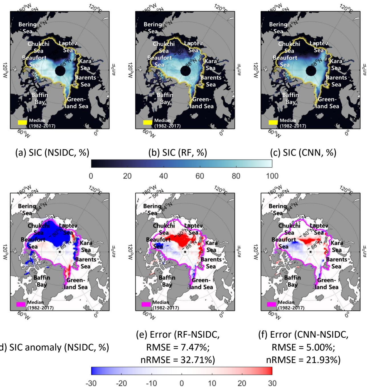
385 Figure 8. The actual SIC (a), predicted SICs (b-c), SIC anomaly (d), and errors between predicted and the actual SICs (e-f) in September 2007.
