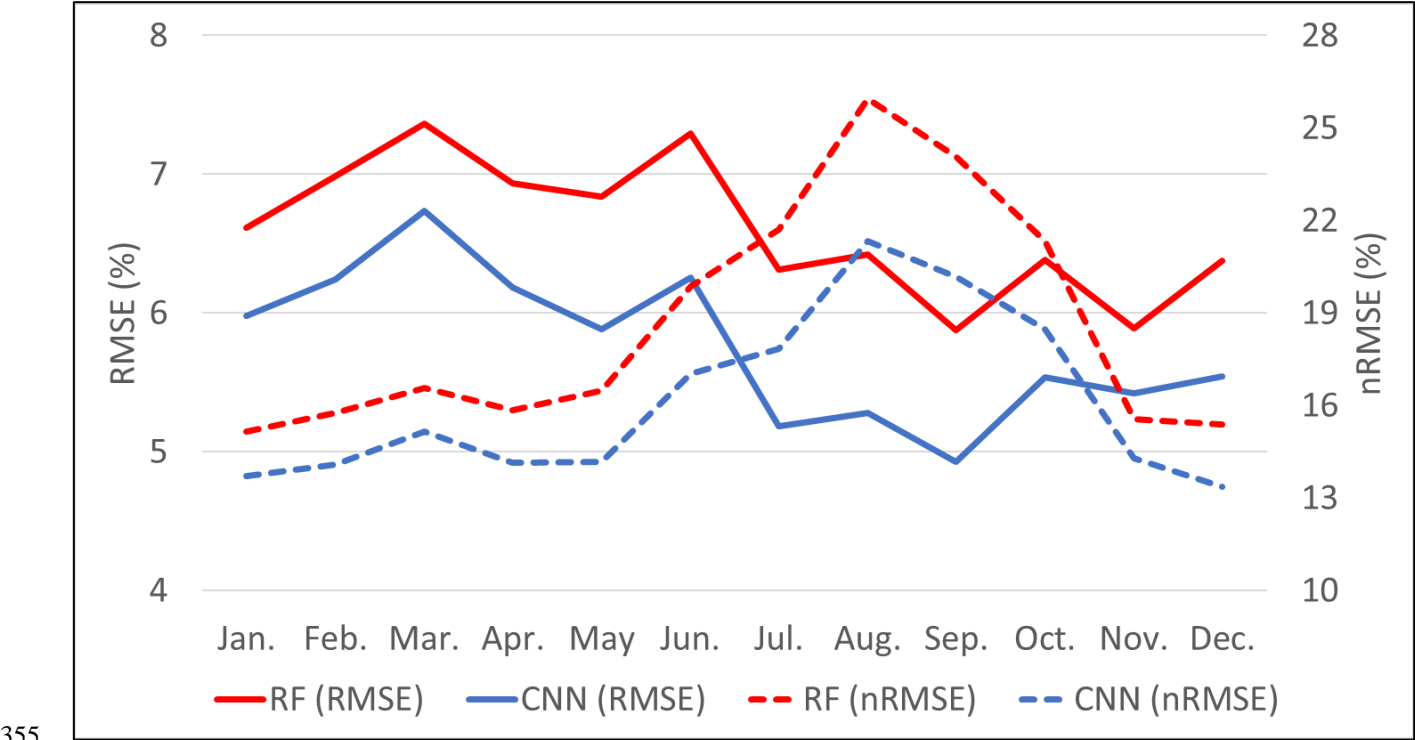
Figure 6. Monthly prediction accuracies with differences between two models for the entire periods (2000-2017, RMSEs and nRMSEs).
