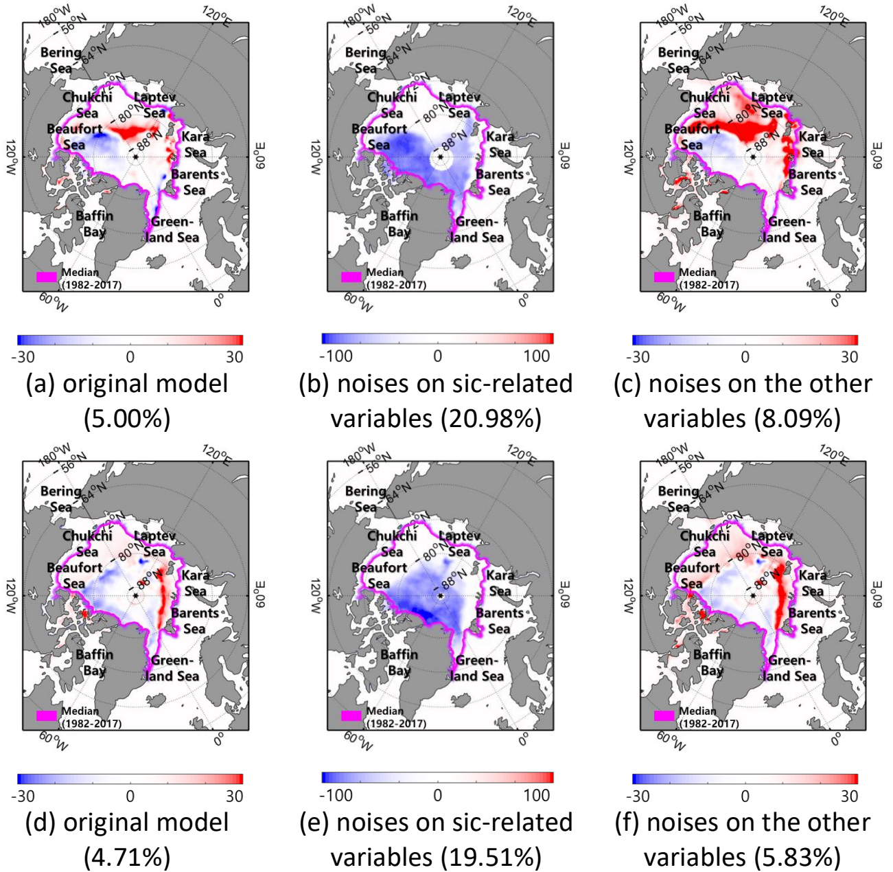
455 Figure 12. The prediction errors (predictions by CNN – NSIDC, %) and RMSE (%) from three prediction results in (a-c) September 2007 (d-f) and 2012: (a and d) original model, (b and e) with noises on SIC variables (sic_1y, sic_1m, ano_1y, and ano_1m), (c and f) with noises 460 on the other variables.
