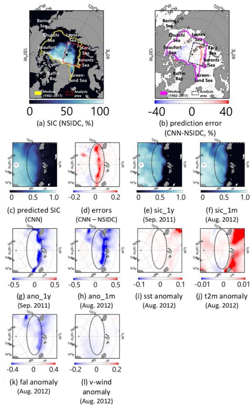
410 Figure 11. Comparison of the prediction results of both models with eight input variables in the Barents Sea–Kara Sea in September 2012. Dotted black circle: the region shows higher prediction errors.
