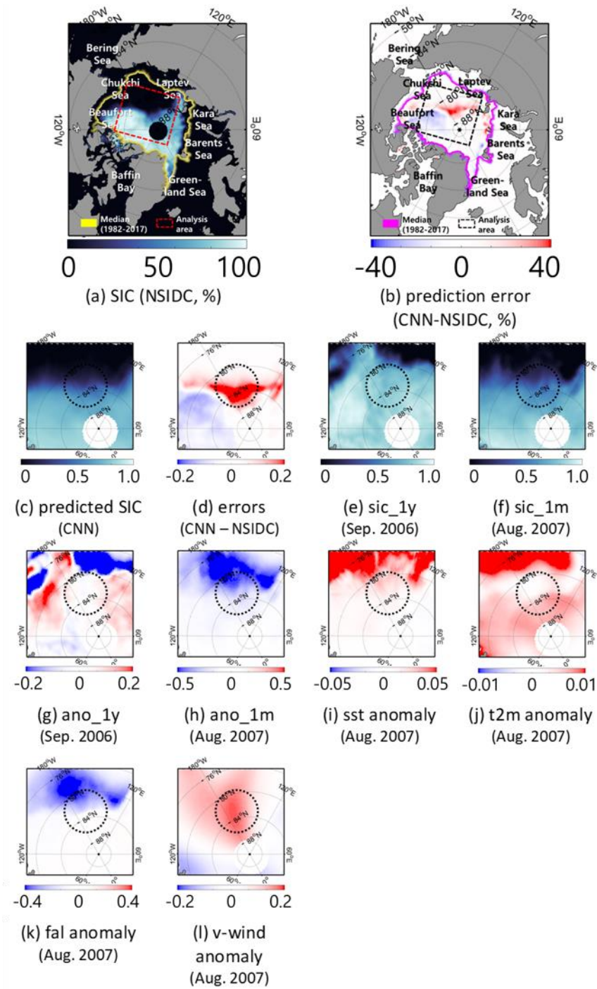
Figure 10. Comparison of the prediction results of both models with eight input variables in the Beaufort Sea–Laptev Sea in September 2007. Dotted black circle: the region shows higher prediction errors.
