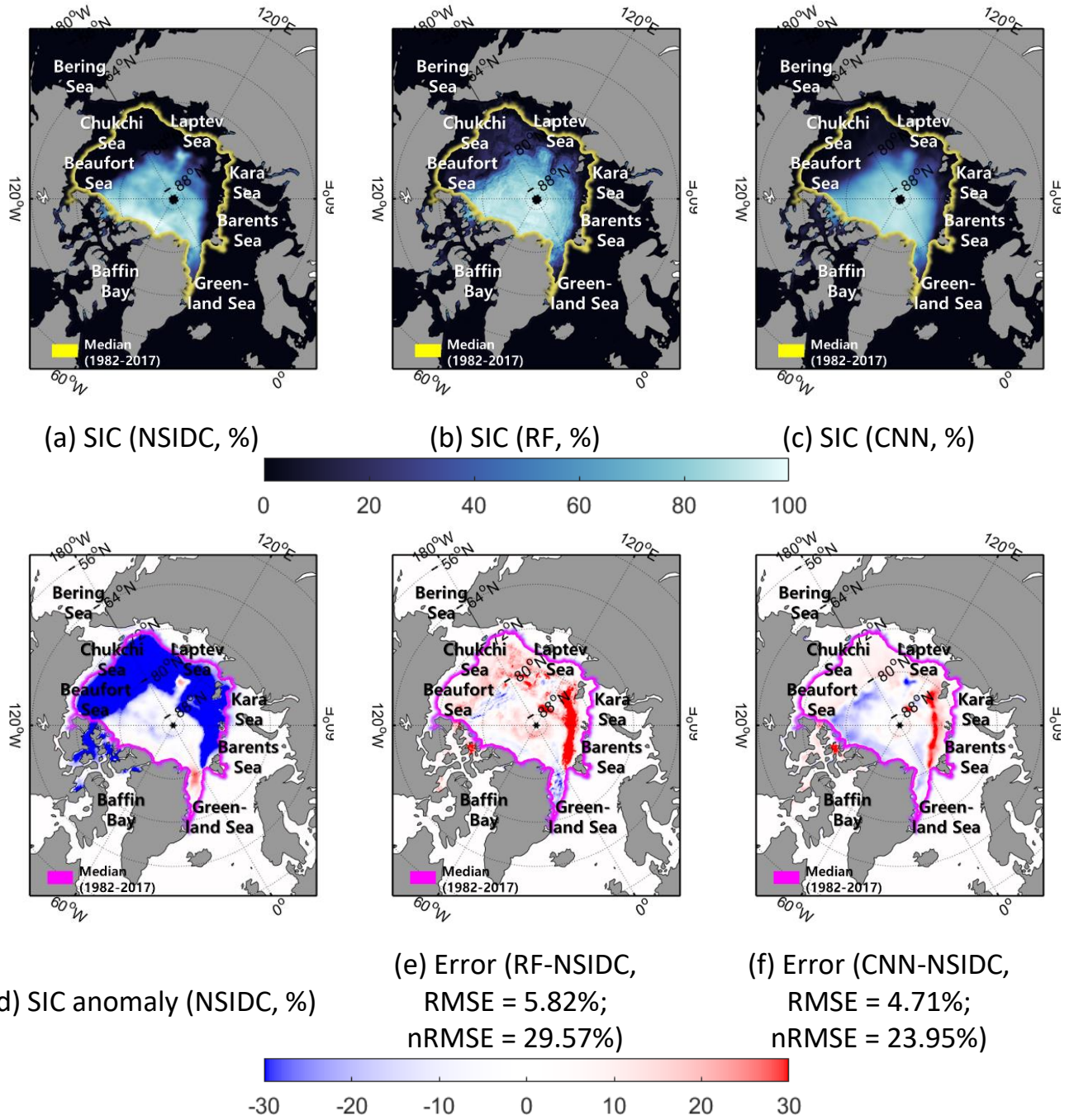
Figure 9. The actual SIC (a), predicted SICs (b-c), SIC anomaly (d), and errors between predicted and the actual SICs (e-f) in September 2012.
