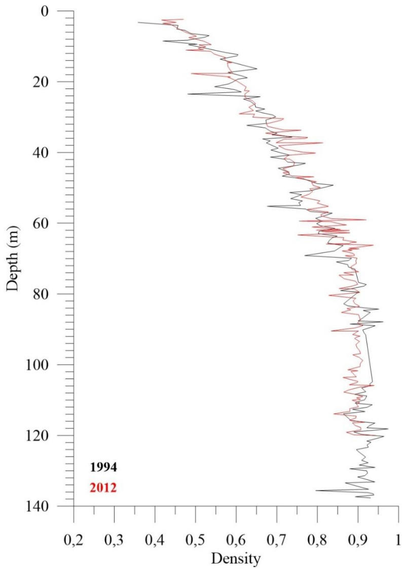
Figure S1: Density profiles in 1994 (black line) and 2012 (red line).
