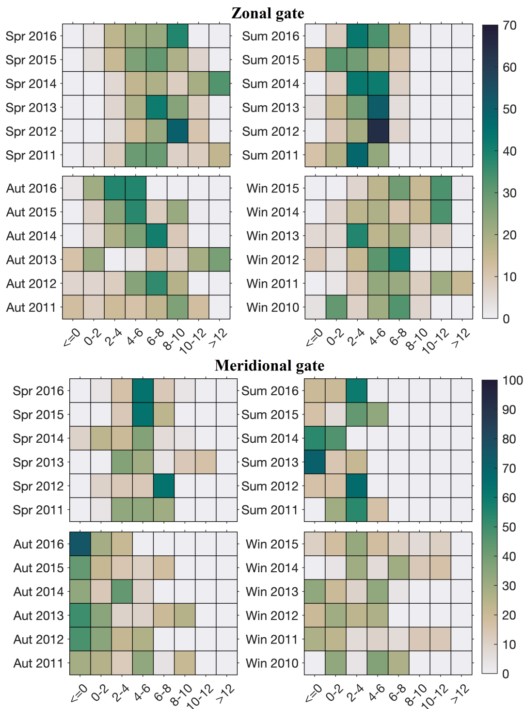
Figure 2. Seasonal variation of relative frequency (unit: %) of CMST sea ice drift (unit: km d -1 ) over the entire Fram Strait gate.
