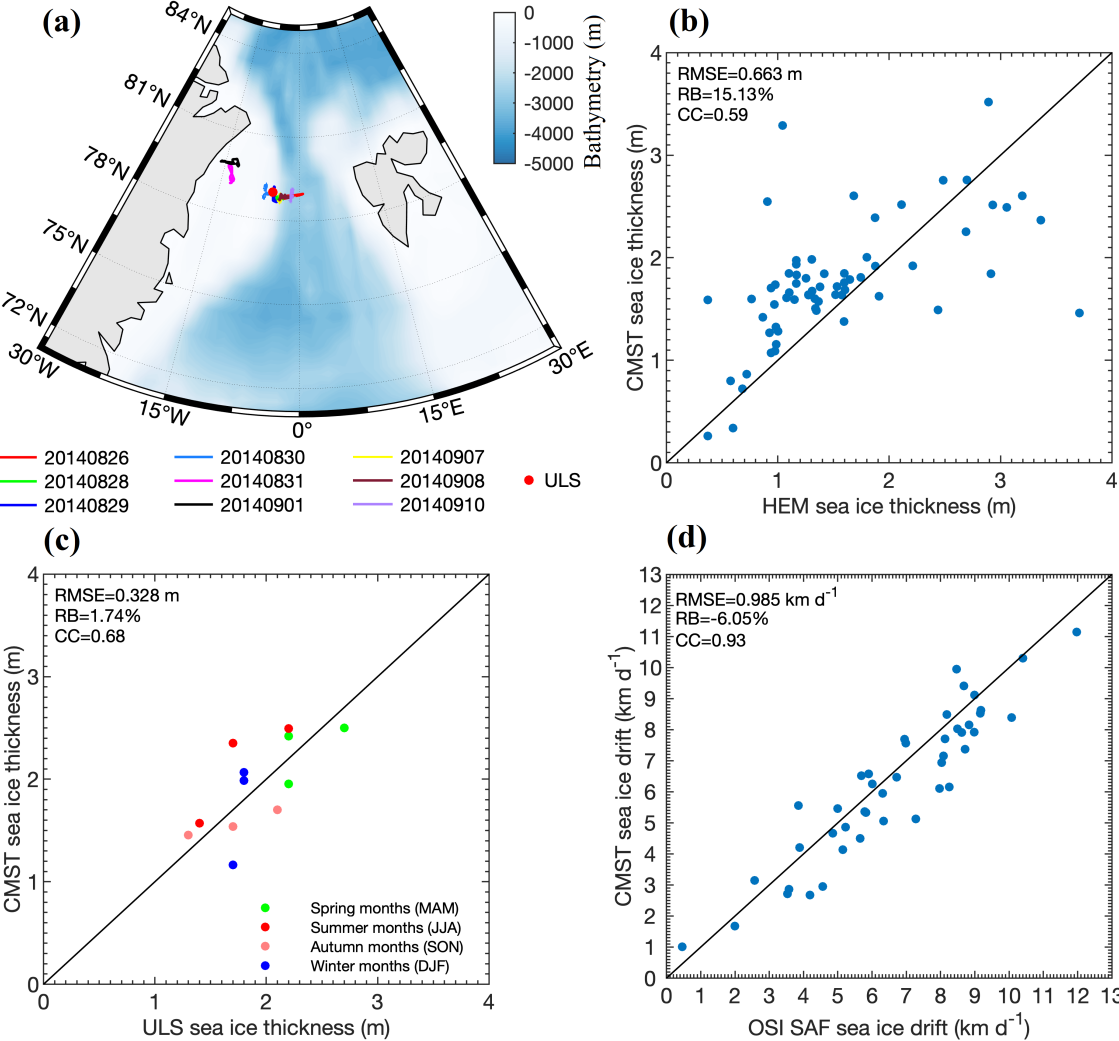
Figure 2. (a) The trajectories of 9 separate flights of HEM measurement campaigns carried out in the Fram Strait and the red dot denotes the site of ULS, -Scatter plots of (b) daily mean sea ice thickness derived from CMST and HEM data, (c) monthly mean sea ice thickness derived from CMST and ULS data, (d) monthly average sea ice drift based on CMST and OSI SAF.
