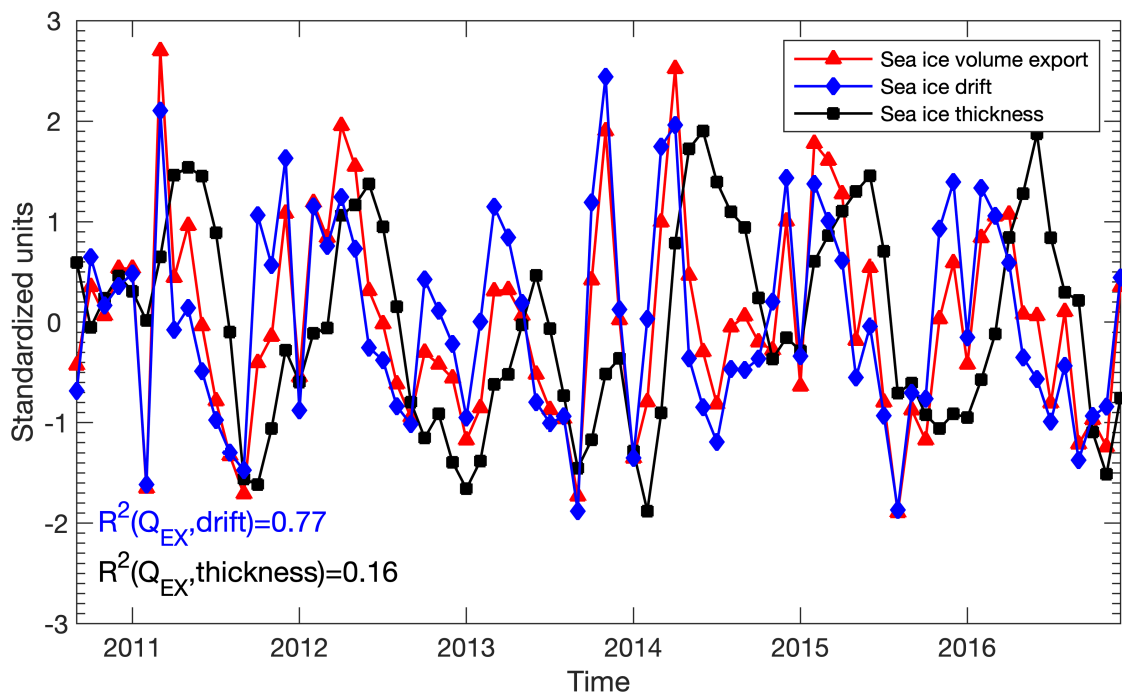
Figure 11. Time series of standardized monthly mean sea ice volume export (red line) and corresponding monthly mean sea ice drift (blue line) and sea ice thickness (black line), including correlation of determination ( R^2 ).
