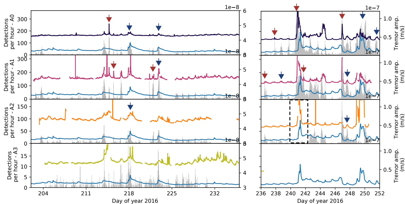
Figure 5. Icequake detections per hour for all arrays (gray bars; see text for details) and the discharge curve of the Simme river (blue line). The black, magenta, orange, and green lines (from top to bottom) are the tremor amplitude curves shown in Fig. 4. Note the different tremor amplitude scaling between the two panels. Blue arrows indicate times where the tremor amplitude correlates with both discharge and icequake rate. Red arrows indicate times where the tremor amplitude correlates with icequake rate, only. The black-dashed rectangle indicates times, where three of five A2 stations tipped over due to diminishing snow cover. The icequake rates in this interval need to be taken with caution.
