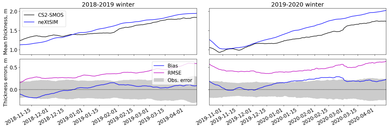
Figure 5. Comparison-Temporal comparison of model and CS2-SMOS thickness for two winters, 2018–2019 in the left-hand columns and 2019–2020 on the right-hand columns . The shaded regions show the RMS uncertainty in the CS2-SMOS product for reference. The mean thickness is the mean over the ocean points in the domain, while the bias is defined as the mean error (model – observation) over the region where either the model or observations have ice .
