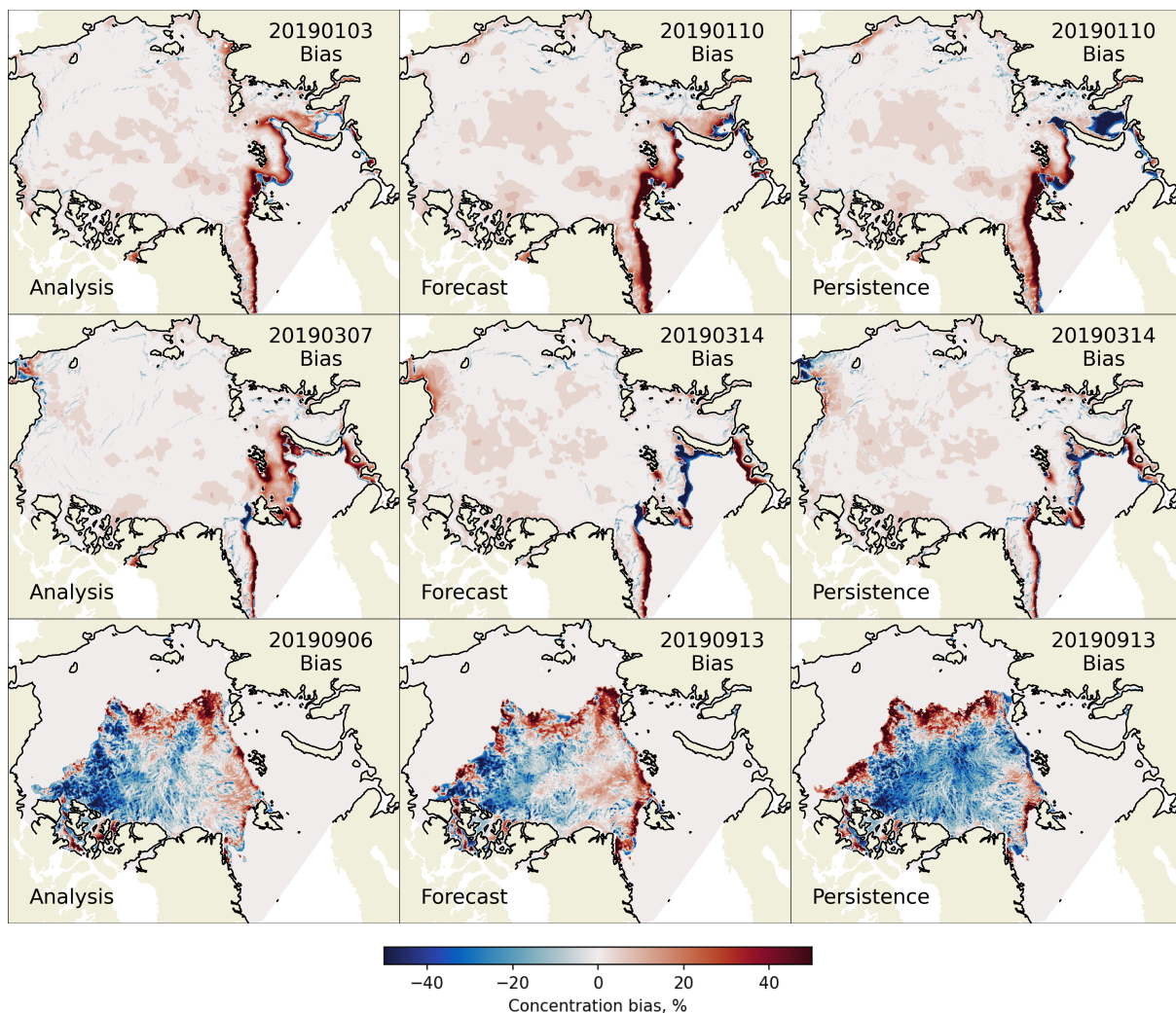
Figure 10. Maps-Selected maps of daily-averaged biases in concentration compared to OSI-SAF SSMI for three examples of forecasts, starting on 3 January 2019 (upper row, positive skill) and the other on 7 March 2019 (middle row, negative skill) and 6 September 2019 (lower row, positive). The left hand columns show the evaluation for the first day of simulation (lead time -1: analysis or hindcast) while the right hand columns show the evaluation for the eighth day of simulation (lead time 7). The right hand columns show the bias in the persistence forecast for lead time 7. The bias is defined as model – observation.
