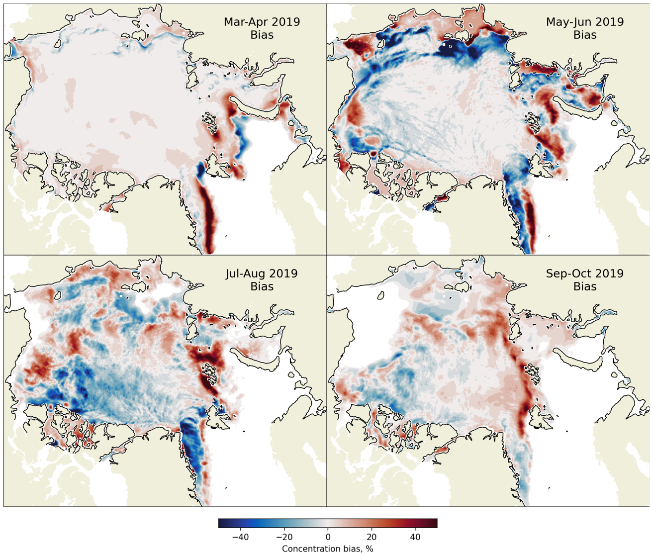
Figure 4. Spatial comparisons Selected maps of selected-the 2-monthly-averaged concentrations from-concentration biases between the free model run and from OSI-SAF SSMI. The bias is defined as model – observation.
