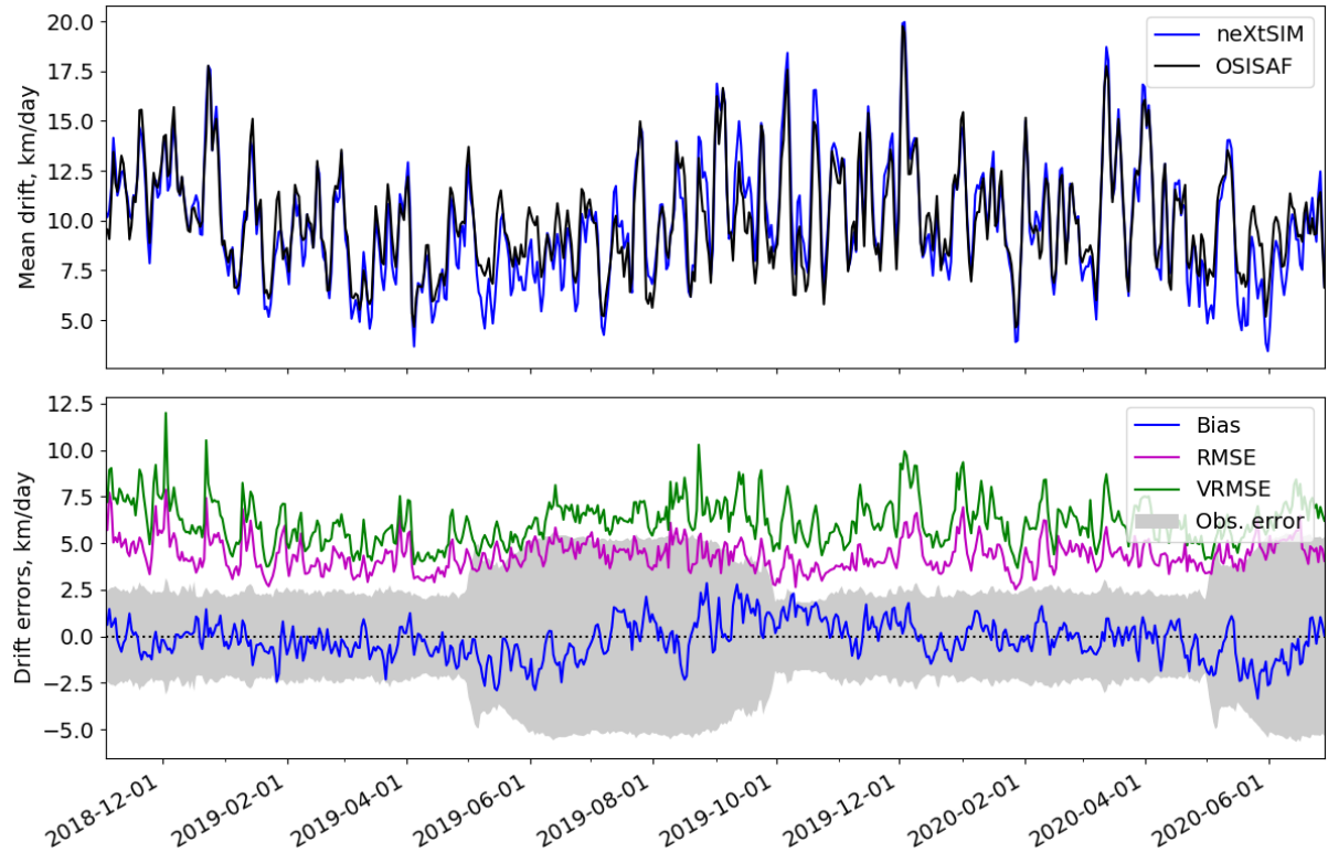
Figure 7. Comparison-Temporal comparison of model and OSI-SAF drift. The shaded region shows the RMS uncertainty in the OSI-SAF drift product. The bias is defined as model-the mean modelled speed – observationobserved speed . The mean drift and errors are averages over the regions where both model and observations have valid drift vectors. Valid observations here are those that have reported errors less than 10 km/day.
