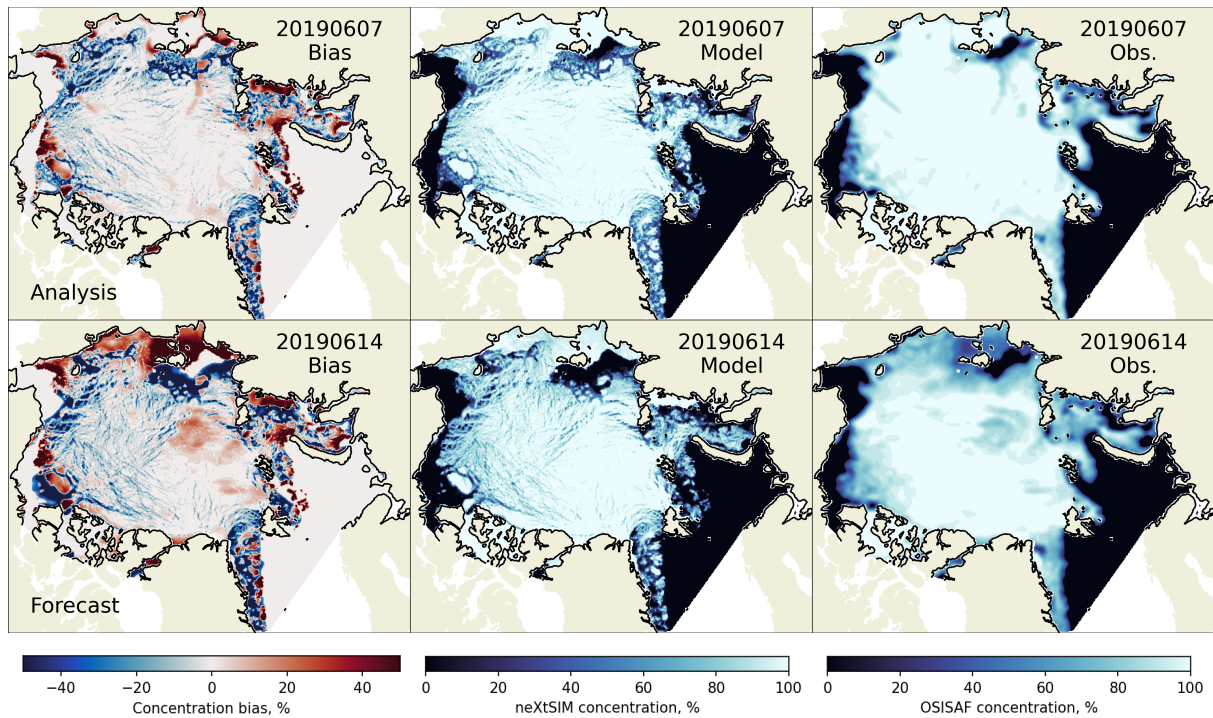
Figure 11. Maps of daily-averaged biases (left-hand columns) in concentration compared to OSI-SAF SSMI, and modelled (centre column) and observed (right-hand column) concentrations, for an example forecast starting on 6 June 2019. The upper row shows the comparison for the first day of simulation while the lower row shows the comparison for the seventh day of simulation. The bias is defined as model – observation.
