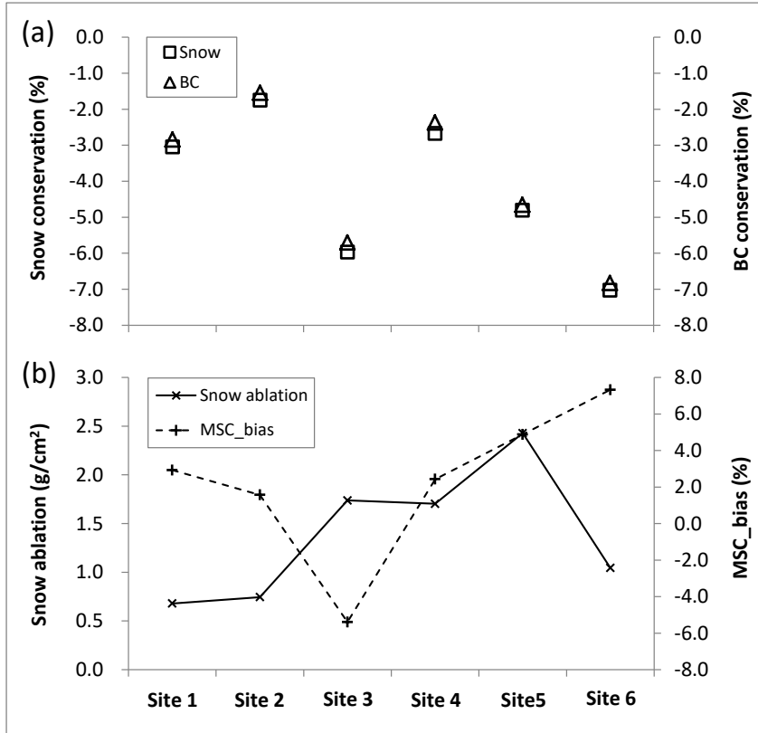
Figure 24: The deviations from 100% conserved for snow and BC after ablation (a), snow ablation ( h_1 \cdot \rho_1 - h_2 \cdot \rho_2 ) during the melt event and the bias ((MSC_2 - MSC_1) / MSC_1) * 100\% of estimated MSC based on Eq. (2) (b). The ticks on the X-axis are matching sites given in Table S21.
