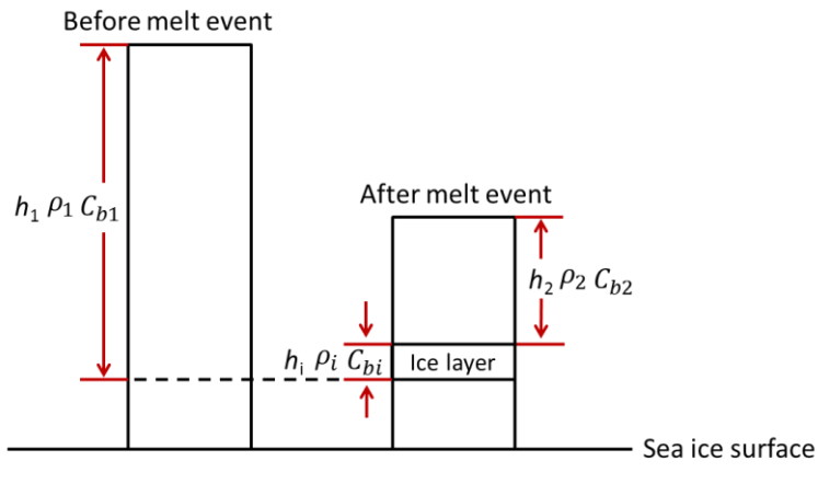
Figure 3: Conceptual sketch of snow overlying sea ice before and after the melt event. Variables relating to the snow and ice layer mentioned in Eq. (1) and Eq. (2) are shown.
