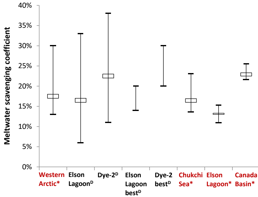
Figure 35: MSC of BC in different regions over the western Arctic. Superscript ‘*’ indicates the results of this study (red), and ‘ D ’ indicates the results of Doherty et al. (2013). Elson Lagoon best D and Dye-2 best D indicate the best-best -estimated range of MSC 2 respectively in Elson Lagoon and Dye-2, Greenland published in Doherty et al. (2013). The values of the western Arctic were estimated based on the observations in all measurement regions, and the best-best -estimated values in Dye-2 and Elson Lagoon were employed in the estimation. The box indicates shows the mean (upper) and median (bottom) values, and the whiskers depict the extent.
