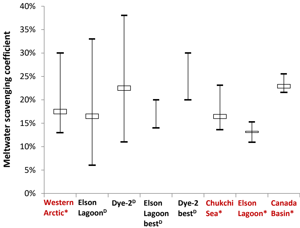
320 | Figure 35: MSC of BC in different regions over the western Arctic. Superscript ‘*’ indicates the results of this study (red), and ‘ D ’ indicates the results of Doherty et al. (2013). Elson Lagoon best D and Dye-2 best D indicate the best-best -estimated range of MSC z respectively in Elson Lagoon and Dye-2, Greenland published in Doherty et al. (2013). The values of the western Arctic were estimated based on the observations in all measurement regions, and the best-best -estimated values in Dye-2 and Elson Lagoon were employed in the estimation. The box indicates-shows the mean (upper) and median (bottom) values, and the whiskers depict 325 | the extent.
