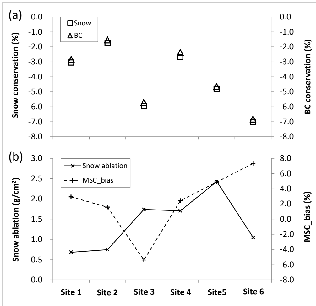
315 | Figure 24: Deviations from 100% conserved for snow and BC after ablation (a), snow ablation ( h_1 \cdot \rho_1 - h_2 \cdot \rho_2 ) during the melt event and the bias ((MSC_2 - MSC_1) / MSC_1) \cdot 100\% of estimated MSC based on Eq. (2) (b). The ticks on the X-axis are matching sites given in Table S21.
