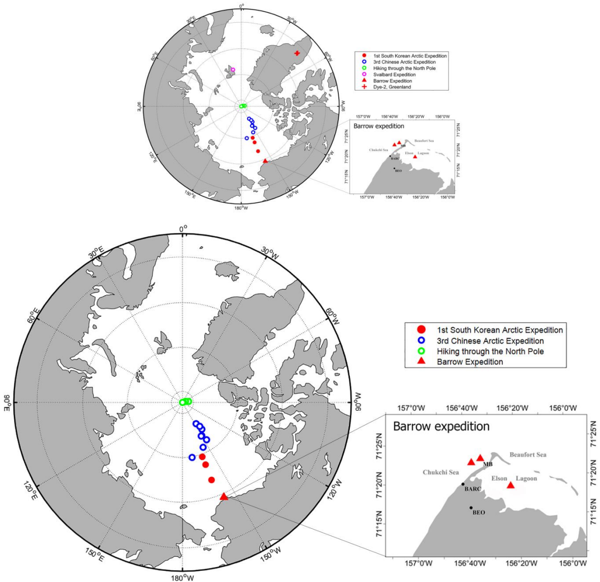
295 Figure 1: Locations of snow and ice layer sampling and the measurements of snow thickness and density in this study. Barrow Expeditions include the field measurements carried out in the Elson Lagoon in 2015, and in the Chukchi Sea in 2017 and 2018; the 3 rd Chinese Arctic Expedition was conducted over the Canada Basin and the center-centre region of Arctic Ocean in 2008; the 1 st South Korean Arctic Expedition was conducted over the Canada Basin in 2010; the North Pole Expedition refers to the first Chinese expedition hiking through the North Pole from 88 °N to 90 °N in 1995 (Xiao et al., 1997); the Svalbard Expedition was conducted by Eckerstorfer et al. (2011) in the field observations in 2007–2009. The open circle indicates the point at which the ice layer is observed. Solid triangles and squares mark the locations for both sampling and on-site measurements. Cross marks the location of Dye-2 where the MSC was estimated by Doherty et al. (2013). 300
