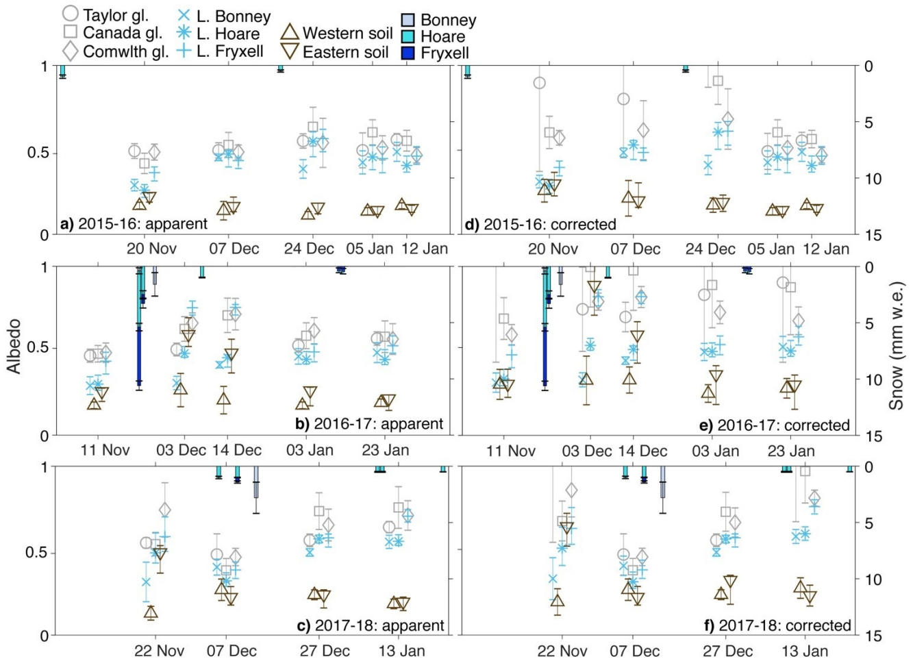
Figure 5. Mean and one standard deviation of albedo measured over the three main glaciers and lakes, and soil in the western (Bonney and Hoare basins) and eastern (Fryxell basin) Taylor Valley during each of the flights. Apparent albedo is shown in a) 2015-16 b) 2016-17 and c) 2017-18 seasons. Corrected albedo is shown in d) 2015-16 e) 2016-17 and f) 2017-18 seasons.
