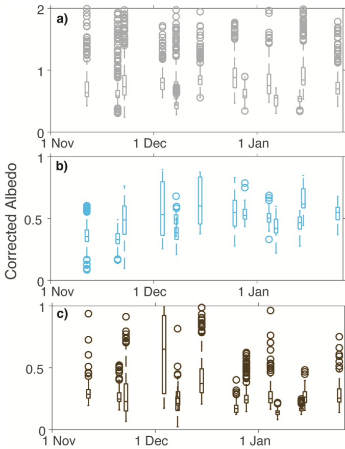
Figure 4. Box plots of corrected albedo from all points measured over a) glaciers, b) lakes, and c) soils. All flights across seasons are shown in plots of each surface type. Boxes are one standard deviation with a line at the mean. Whiskers are 99 percent of data with open circles signifying outliers. Note different y-axis scale for glaciers.
