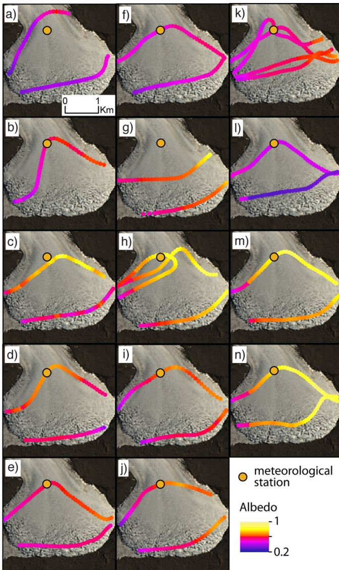
Figure 11. Flight paths of each flight on Canada Glacier in the 2015-16 season (a-e) 2016-17 season (f-j) and 2017-18 season (k-n). Points are locations of measurements made along the flight path color scaled by apparent albedo at that location. Background imagery is provided by USGS/NASA; Landsat8 image collected on 14 January, 2016.
