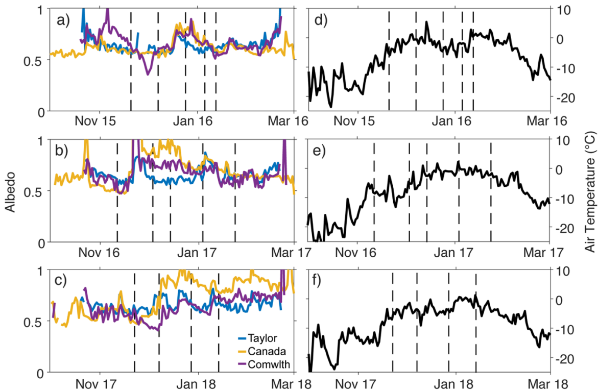
Figure 6. Timeseries of albedo measured at Taylor, Canada, and Commonwealth meteorological stations over the a) 2015-16, b) 2016-17 and c) 2017-18 seasons. Time series of air temperature measured at the Lake Hoare station of the d) 2015-16, e) 2016-17 and f) 2017-18 seasons. Lake Hoare has the best temperature record and is representative of temperature across the entire valley. Vertical dashed black lines on all figures are the times are which airborne albedo measurements were made.
