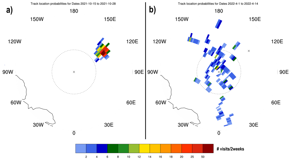
Figure S1: Counts of visits to each grid cell by Seasonal Arctic tracks in a two-week period during Oct.15-Oct.28 (a) and Apr.1-Apr.14 (b). Black 'X's mark the starting location of the campaign as well as the North Pole. The Black circle marks the location of highest counts in the two-week time period. The dashed black line at 87°N shows where satellite coverage is not available.
