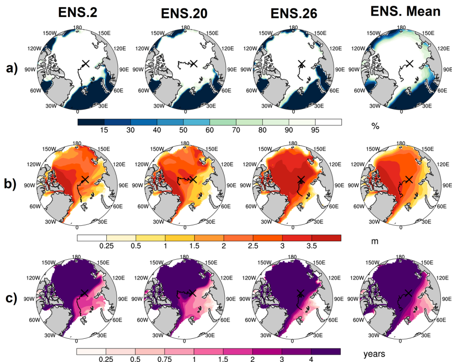
480 Figure 4: Perennial grid cell daily mean sea ice concentration (a), thickness (b), and ice age (c) on October 15. Three random ensembles from the CESM-LE and the ensemble mean are shown. The black 'X' in each map denotes the campaign starting location. Overlain as black lines are the Lagrangian tracks for each ensemble member and the representative track from Fig.1 for the ensemble mean.
