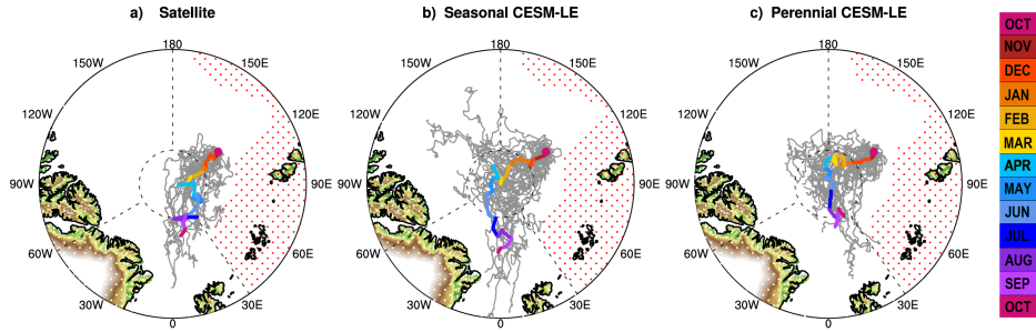
440 Figure 1: Unique ice floe tracks (grey) for satellite observations (a), Seasonal (b) and Perennial (c) CESM-LE ensembles. Representative tracks (coloured with corresponding months shown at far right) based on the individual tracks are overlain. Dashed lines indicate boundaries for the Transpolar Drift, North Pole, Russian, and Canadian sectors described in Table 1. The Russian exclusive economic zone (EEZ) is shown by red stipples.
