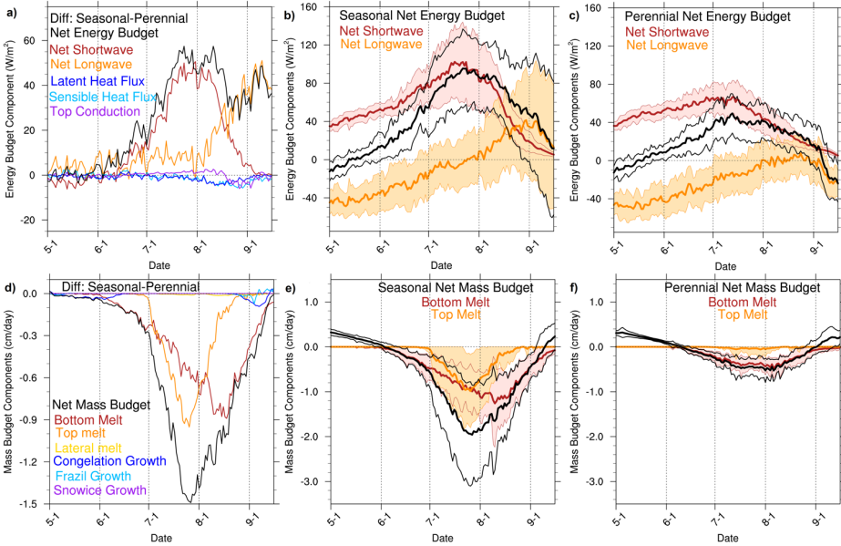
Figure 7: Melt season daily along-track mean surface energy budget (a) and mass budget (d) differences (Seasonal tracks minus Perennial tracks). The ensemble mean (solid) and +/-1 standard deviation envelope (shaded) are shown for the components with the largest differences for the energy budget (b, c) and mass budget (e, f). Components of the energy budget include: net (black), net shortwave (red), net longwave (orange), latent heat flux (dark blue), sensible heat flux (light blue), and top conductive flux (purple). Components of the mass budget include: net (black), bottom melt (red), top melt (orange), lateral melt (gold), congelation growth (dark blue), frazil growth (light blue), and snow-ice growth (purple). The melt season shown here corresponds to May 1 to September 15.
