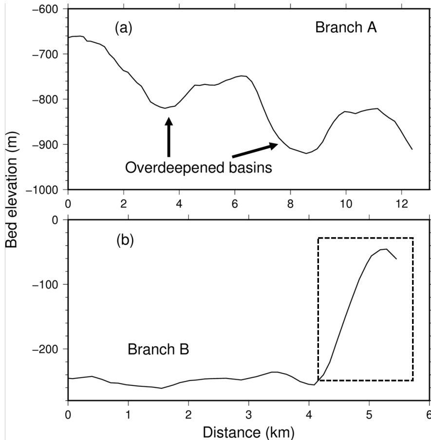
10 Figure 8. Bed elevation profiles of two branches derived from BedMachine v3 (Morlighem et al., 2017). The profile locations are shown in Fig. 1a. The dashed box shows the zone where the bed slopes uphill inland.
