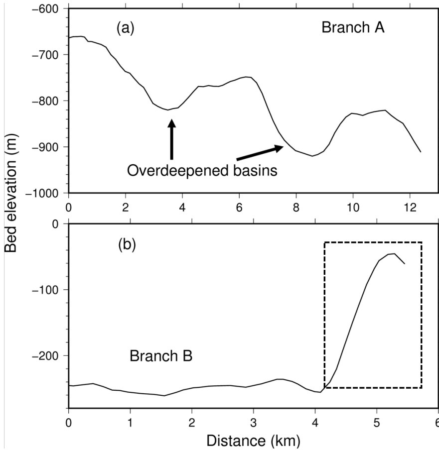
Figure 8. Bed elevation profiles of two branches derived from BedMachine v3 (Morlighem et al., 2017). The profile locations are shown in Fig. 1a. The dashed box shows the zone where the bed slopes uphill inland.
